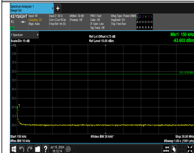
5-5-3MHz-5MHz-16QAM-16QAM-20586-20625-1RB#0-0R B#0-0.15~30MHz-PASS
