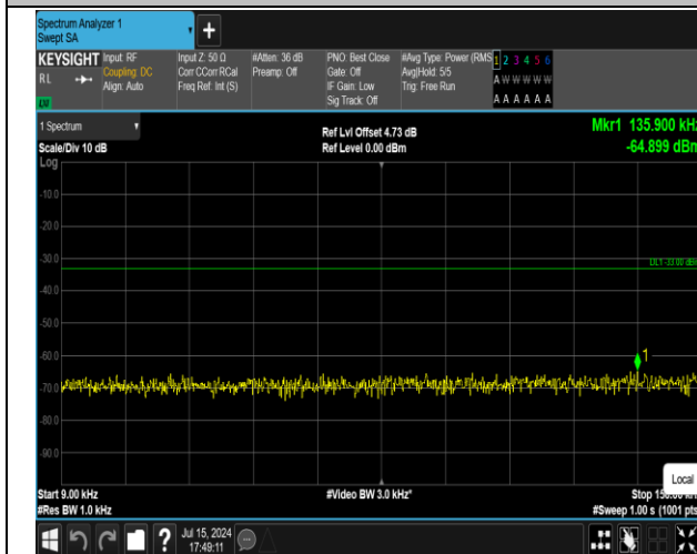
5-5-3MHz-5MHz-QPSK-QPSK-20416-20455-1RB#0-1RB# 24-0.009~0.15MHz-PASS
