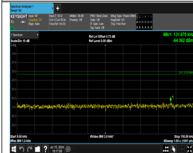
5-5-3MHz-5MHz-QPSK-QPSK-20586-20625-15RB#0-25R B#0-0.009~0.15MHz-PASS
