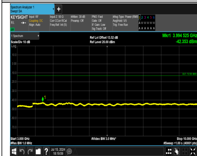
5-5-3MHz-5MHz-16QAM-16QAM-20586-20625-15RB#0-2 5RB#0-3000~10000MHz-PASS
