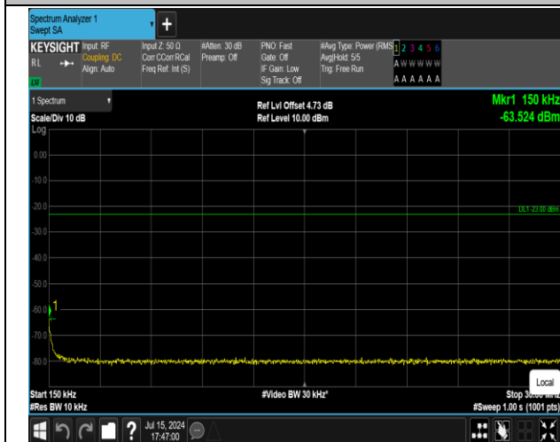
5-5-3MHz-5MHz-QPSK-QPSK-20416-20455-1RB#14-0RB #0-0.15~30MHz-PASS
