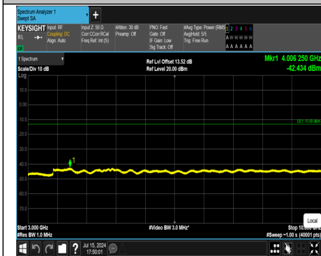
5-5-3MHz-5MHz-QPSK-QPSK-20416-20455-1RB#0-1RB# 24-3000~10000MHz-PASS
