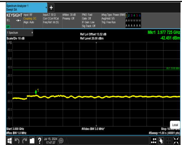
5-5-3MHz-5MHz-QPSK-QPSK-20416-20455-1RB#14-0RB #0-3000~10000MHz-PASS
