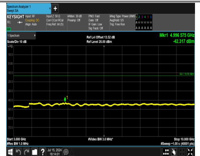
5-5-3MHz-5MHz-QPSK-QPSK-20586-20625-1RB#14-0RB #0-3000~10000MHz-PASS
