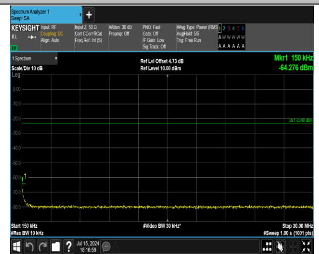
5-5-3MHz-5MHz-16QAM-16QAM-20586-20625-1RB#0-1R B#24-0.15~30MHz-PASS
