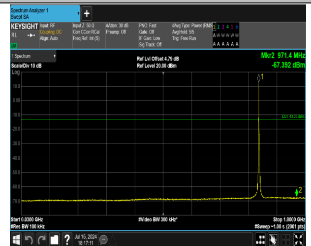
5-5-3MHz-5MHz-16QAM-16QAM-20586-20625-1RB#0-1R B#24-30~1000MHz-PASS
