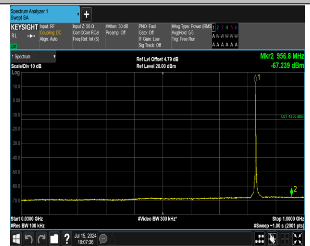
5-5-3MHz-5MHz-16QAM-16QAM-20501-20540-1RB#0-1R B#24-30~1000MHz-PASS
