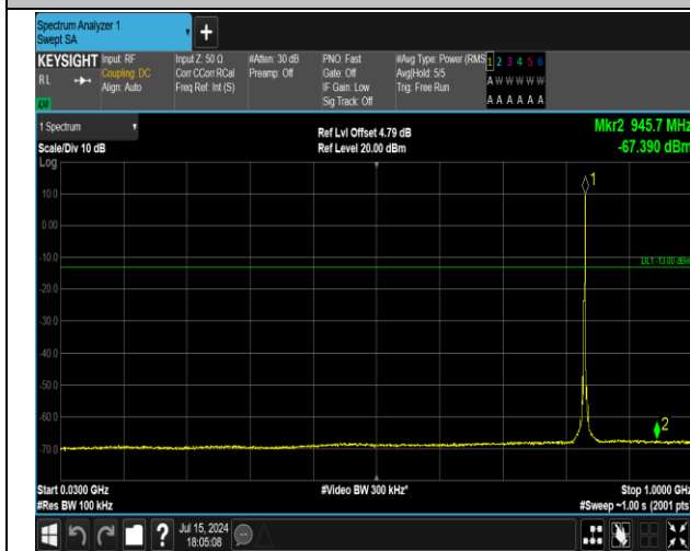
5-5-3MHz-5MHz-16QAM-16QAM-20501-20540-1RB#14-0 RB#0-30~1000MHz-PASS
