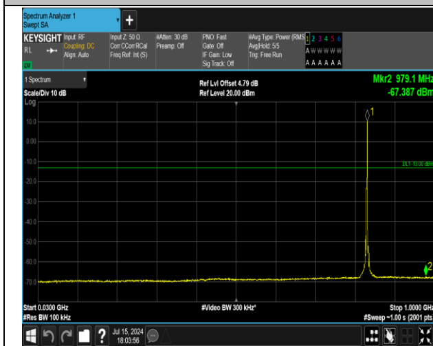
5-5-3MHz-5MHz-QPSK-QPSK-20501-20540-1RB#14-0RB #0-30~1000MHz-PASS
