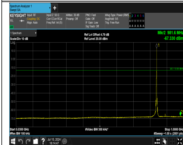
5-5-3MHz-5MHz-16QAM-16QAM-20586-20625-1RB#14-0 RB#0-30~1000MHz-PASS
