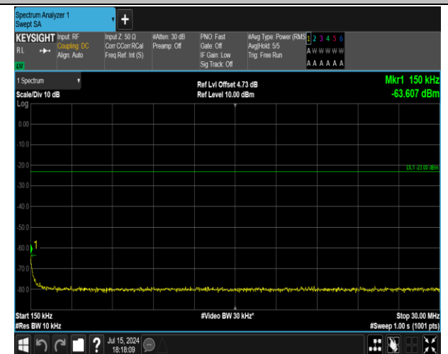
5-5-3MHz-5MHz-QPSK-QPSK-20586-20625-15RB#0-25R B#0-0.15~30MHz-PASS
