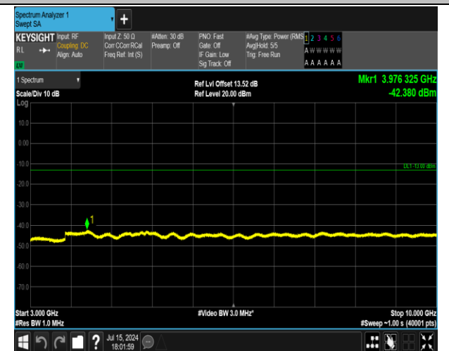
5-5-3MHz-5MHz-QPSK-QPSK-20501-20540-1RB#0-0RB# 0-3000~10000MHz-PASS
