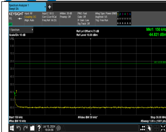
5-5-3MHz-5MHz-16QAM-16QAM-20501-20540-1RB#14-0 RB#0-0.15~30MHz-PASS
