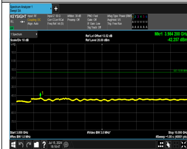
5-5-3MHz-5MHz-QPSK-QPSK-20586-20625-15RB#0-25R B#0-3000~10000MHz-PASS
