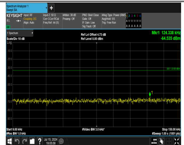
5-5-5MHz-3MHz-16QAM-16QAM-20425-20464-1RB#0-1R B#15-0.009~0.15MHz-PASS
