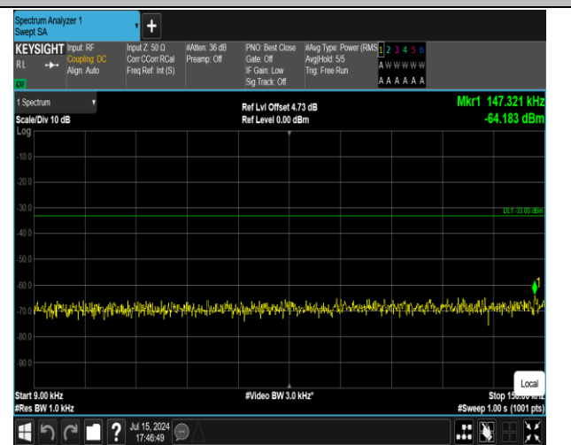
5-5-3MHz-5MHz-QPSK-QPSK-20416-20455-1RB#14-0RB #0-0.009~0.15MHz-PASS
