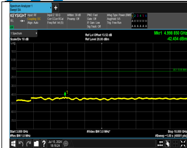
5-5-3MHz-5MHz-QPSK-QPSK-20586-20625-1RB#0-1RB# 24-3000~10000MHz-PASS
