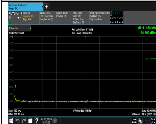
5-5-3MHz-5MHz-QPSK-QPSK-20586-20625-1RB#0-0RB# 0-0.15~30MHz-PASS
