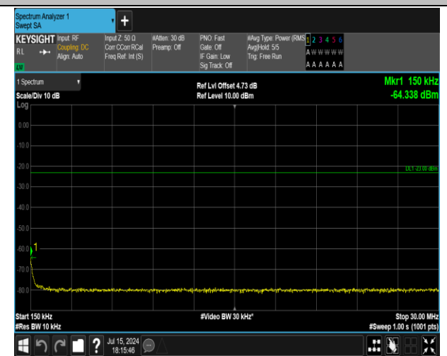
5-5-3MHz-5MHz-QPSK-QPSK-20586-20625-1RB#0-1RB# 24-0.15~30MHz-PASS
