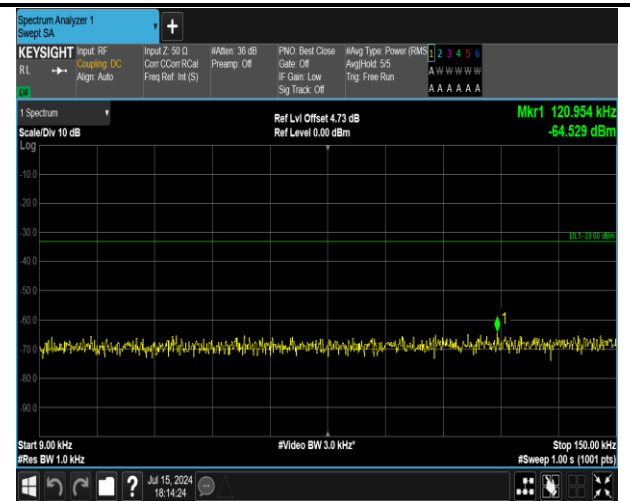
5-5-3MHz-5MHz-16QAM-16QAM-20586-20625-1RB#14-0 RB#0-0.009~0.15MHz-PASS
