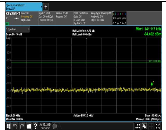
5-5-3MHz-5MHz-QPSK-QPSK-20586-20625-1RB#14-0RB #0-0.009~0.15MHz-PASS
