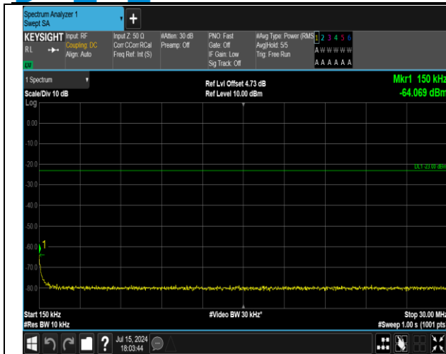
5-5-3MHz-5MHz-QPSK-QPSK-20501-20540-1RB#14-0RB #0-0.15~30MHz-PASS
