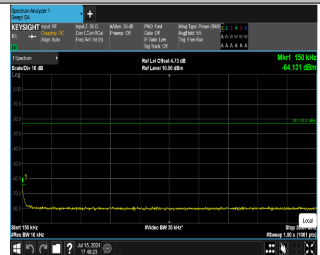
5-5-3MHz-5MHz-QPSK-QPSK-20416-20455-1RB#0-1RB# 24-0.15~30MHz-PASS
