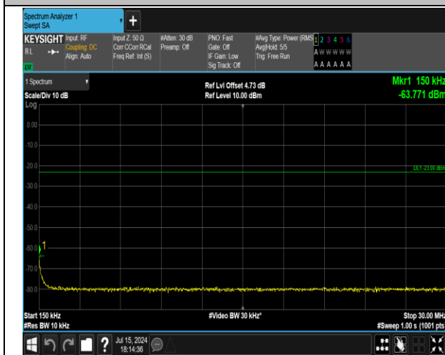
5-5-3MHz-5MHz-16QAM-16QAM-20586-20625-1RB#14-0 RB#0-0.15~30MHz-PASS
