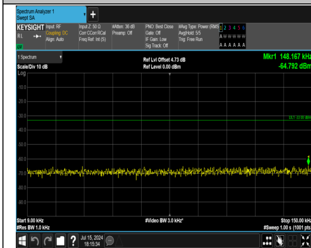
5-5-3MHz-5MHz-QPSK-QPSK-20586-20625-1RB#0-1RB# 24-0.009~0.15MHz-PASS
