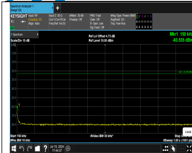
5-5-3MHz-5MHz-QPSK-QPSK-20416-20455-1RB#0-0RB# 0-0.15~30MHz-PASS
