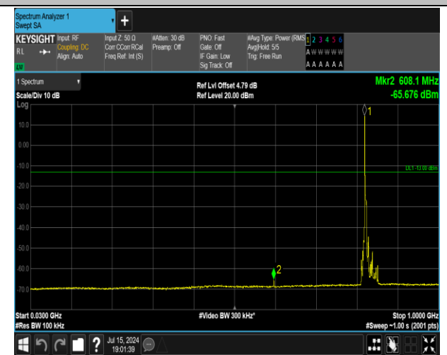
5-5-5MHz-3MHz-16QAM-16QAM-20425-20464-1RB#0-0R B#0-30~1000MHz-PASS
