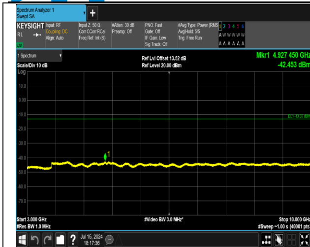
5-5-3MHz-5MHz-16QAM-16QAM-20586-20625-1RB#0-1R B#24-3000~10000MHz-PASS
