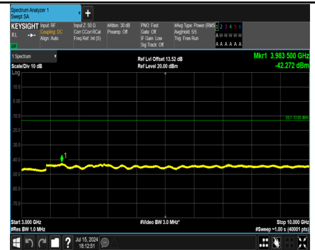
5-5-3MHz-5MHz-16QAM-16QAM-20586-20625-1RB#0-0R B#0-3000~10000MHz-PASS
