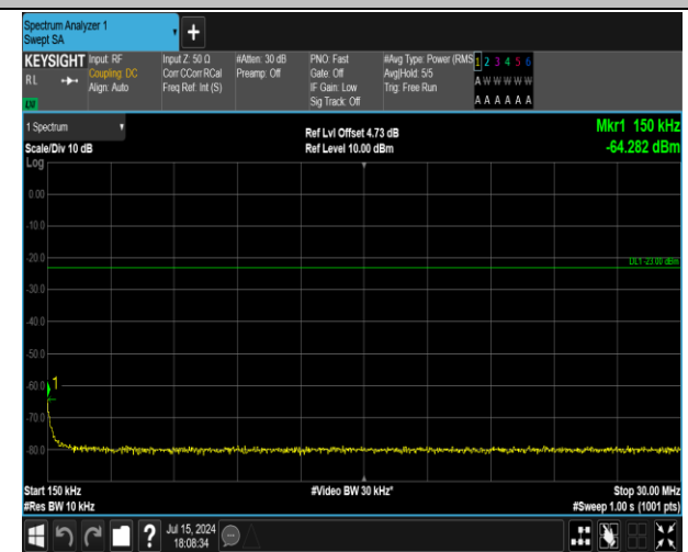
5-5-3MHz-5MHz-QPSK-QPSK-20501-20540-15RB#0-25R B#0-0.15~30MHz-PASS
