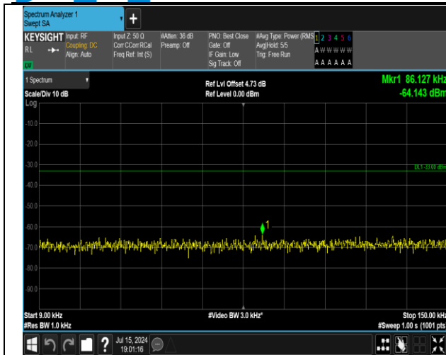
5-5-5MHz-3MHz-16QAM-16QAM-20425-20464-1RB#0-0R B#0-0.009~0.15MHz-PASS
