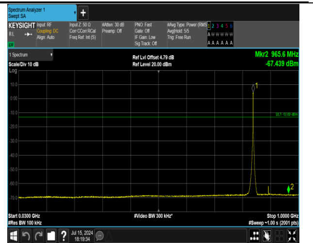
5-5-3MHz-5MHz-16QAM-16QAM-20586-20625-15RB#0-2 5RB#0-30~1000MHz-PASS
