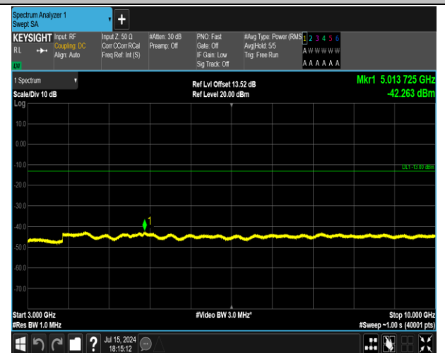
5-5-3MHz-5MHz-16QAM-16QAM-20586-20625-1RB#14-0 RB#0-3000~10000MHz-PASS
