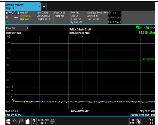
5-5-5MHz-3MHz-16QAM-16QAM-20425-20464-1RB#0-0R B#0-0.15~30MHz-PASS
