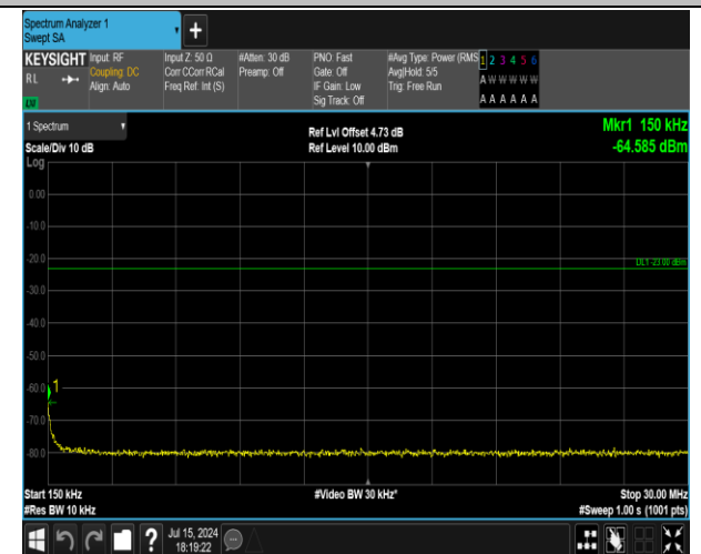
5-5-3MHz-5MHz-16QAM-16QAM-20586-20625-15RB#0-2 5RB#0-0.15~30MHz-PASS
