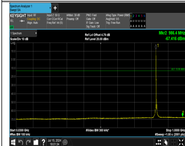
5-5-3MHz-5MHz-QPSK-QPSK-20501-20540-1RB#0-0RB# 0-30~1000MHz-PASS
