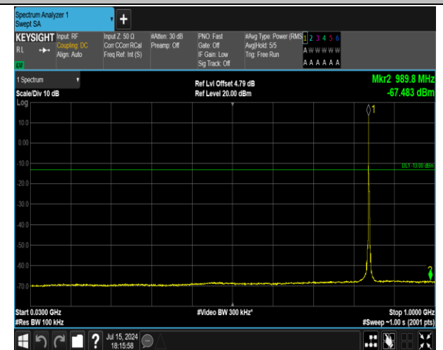
5-5-3MHz-5MHz-QPSK-QPSK-20586-20625-1RB#0-1RB# 24-30~1000MHz-PASS
