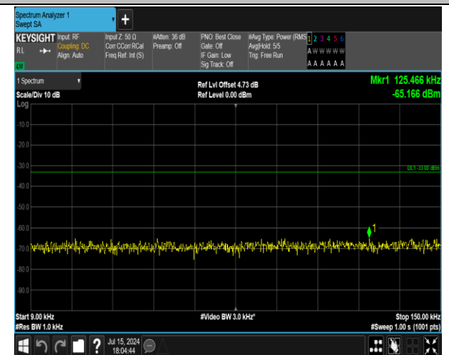
5-5-3MHz-5MHz-16QAM-16QAM-20501-20540-1RB#14-0 RB#0-0.009~0.15MHz-PASS
