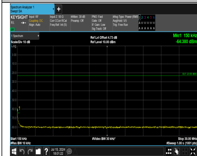
5-5-3MHz-5MHz-QPSK-QPSK-20501-20540-1RB#0-0RB# 0-0.15~30MHz-PASS
