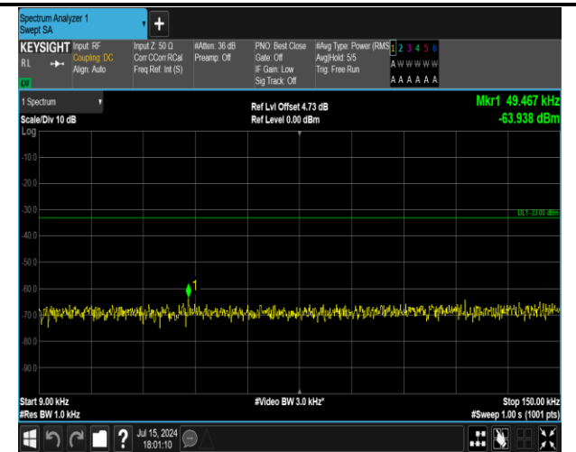
5-5-3MHz-5MHz-QPSK-QPSK-20501-20540-1RB#0-0RB# 0-0.009~0.15MHz-PASS
