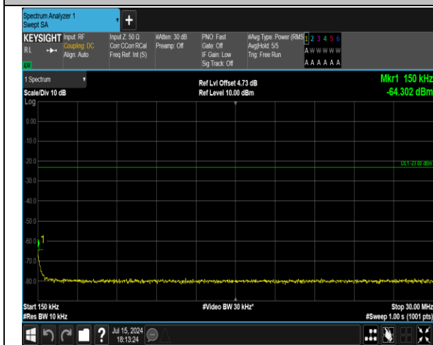
5-5-3MHz-5MHz-QPSK-QPSK-20586-20625-1RB#14-0RB #0-0.15~30MHz-PASS
