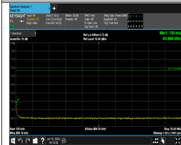
5-5-5MHz-3MHz-QPSK-QPSK-20510-20549-1RB#0-1RB# 15-0.15~30MHz-PASS
