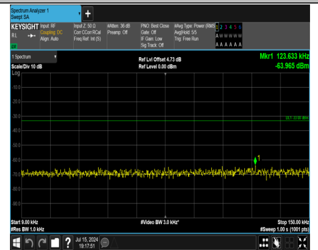
5-5-5MHz-3MHz-16QAM-16QAM-20510-20549-25RB#0-1 5RB#0-0.009~0.15MHz-PASS
