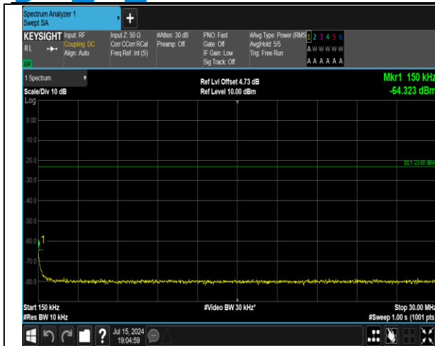
5-5-5MHz-3MHz-QPSK-QPSK-20425-20464-1RB#0-1RB# 15-0.15~30MHz-PASS
