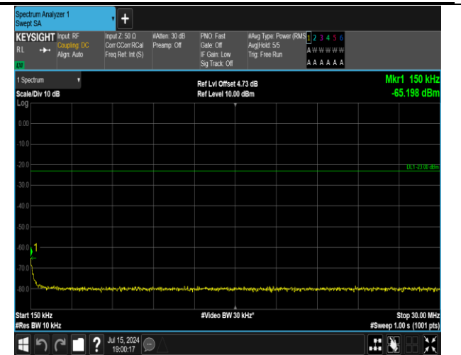
5-5-5MHz-3MHz-QPSK-QPSK-20425-20464-1RB#0-0RB# 0-0.15~30MHz-PASS
