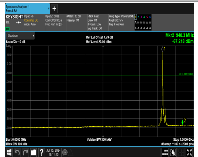
5-5-5MHz-3MHz-16QAM-16QAM-20510-20549-1RB#0-0R B#0-30~1000MHz-PASS
