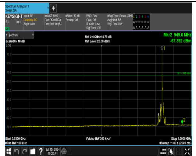
5-5-5MHz-3MHz-16QAM-16QAM-20595-20634-1RB#0-0R B#0-30~1000MHz-PASS
