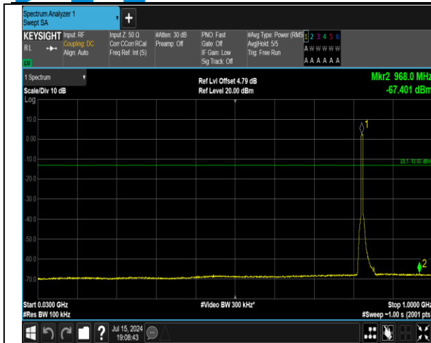
5-5-5MHz-3MHz-16QAM-16QAM-20425-20464-25RB#0-1 5RB#0-30~1000MHz-PASS
