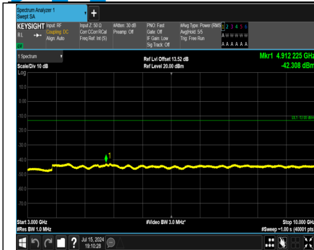
5-5-5MHz-3MHz-QPSK-QPSK-20510-20549-1RB#0-0RB# 0-3000~10000MHz-PASS
