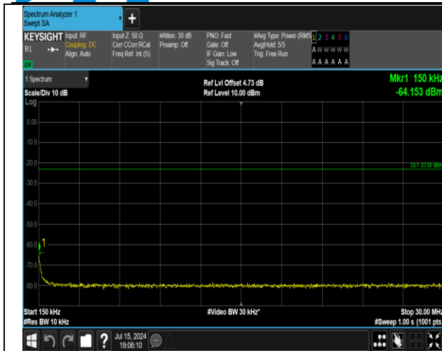
5-5-5MHz-3MHz-16QAM-16QAM-20425-20464-1RB#0-1R B#15-0.15~30MHz-PASS
