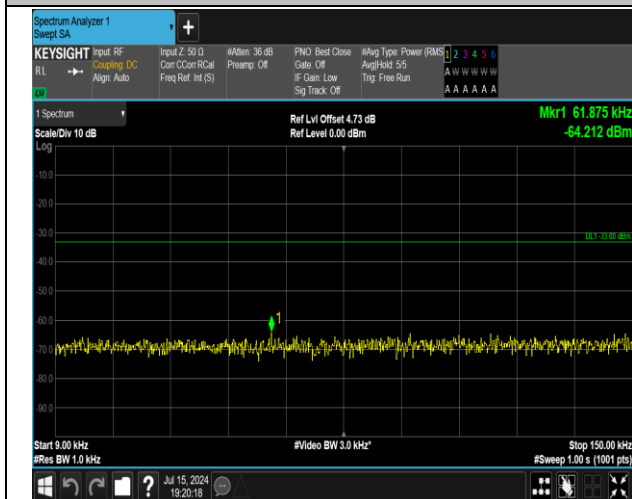
5-5-5MHz-3MHz-16QAM-16QAM-20595-20634-1RB#0-0R B#0-0.009~0.15MHz-PASS
