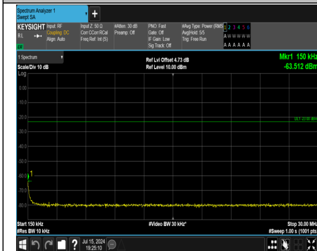
5-5-5MHz-3MHz-16QAM-16QAM-20595-20634-1RB#0-1R B#15-0.15~30MHz-PASS
