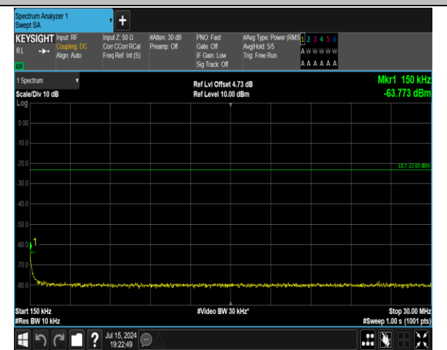
5-5-5MHz-3MHz-16QAM-16QAM-20595-20634-1RB#24-0 RB#0-0.15~30MHz-PASS
