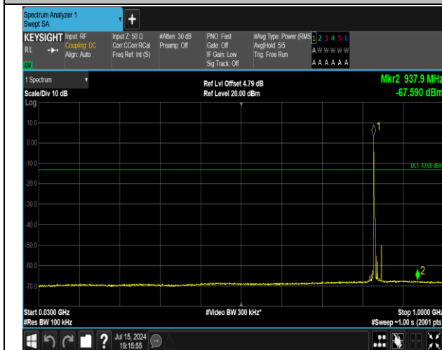
5-5-5MHz-3MHz-16QAM-16QAM-20510-20549-1RB#0-1R B#15-30~1000MHz-PASS
