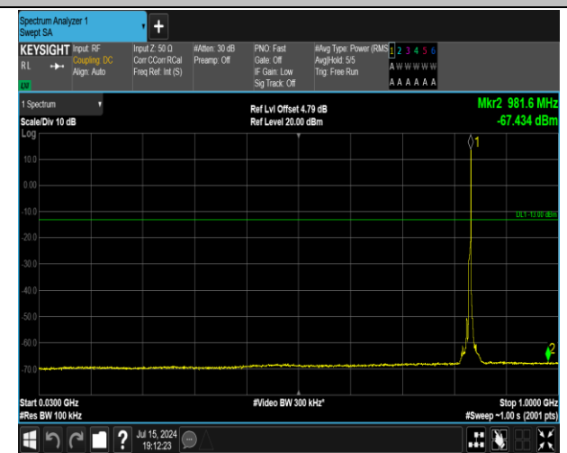
5-5-5MHz-3MHz-QPSK-QPSK-20510-20549-1RB#24-0RB #0-30~1000MHz-PASS
