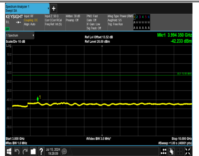
5-5-5MHz-3MHz-16QAM-16QAM-20595-20634-25RB#0-1 5RB#0-3000~10000MHz-PASS
