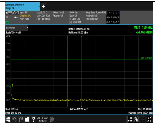
5-5-5MHz-3MHz-QPSK-QPSK-20510-20549-1RB#24-0RB #0-0.15~30MHz-PASS
