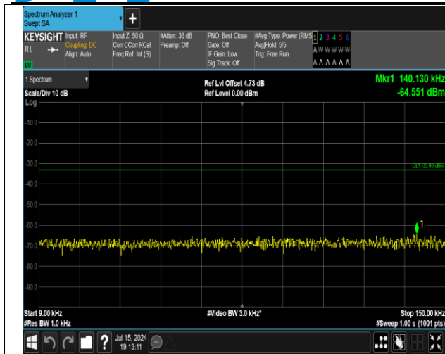
5-5-5MHz-3MHz-16QAM-16QAM-20510-20549-1RB#24-0 RB#0-0.009~0.15MHz-PASS
