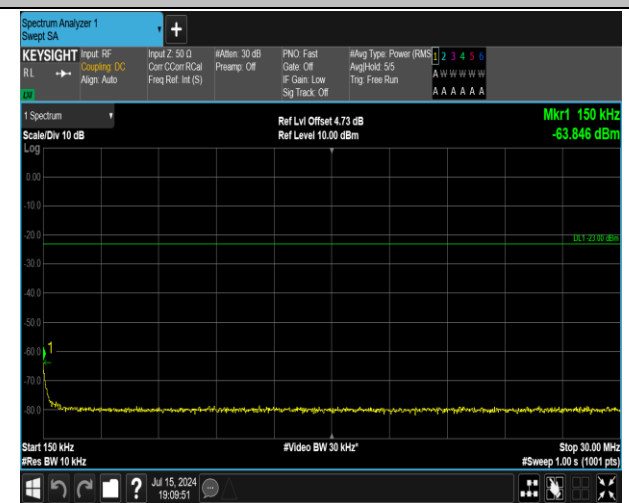
5-5-5MHz-3MHz-QPSK-QPSK-20510-20549-1RB#0-0RB# 0-0.15~30MHz-PASS
