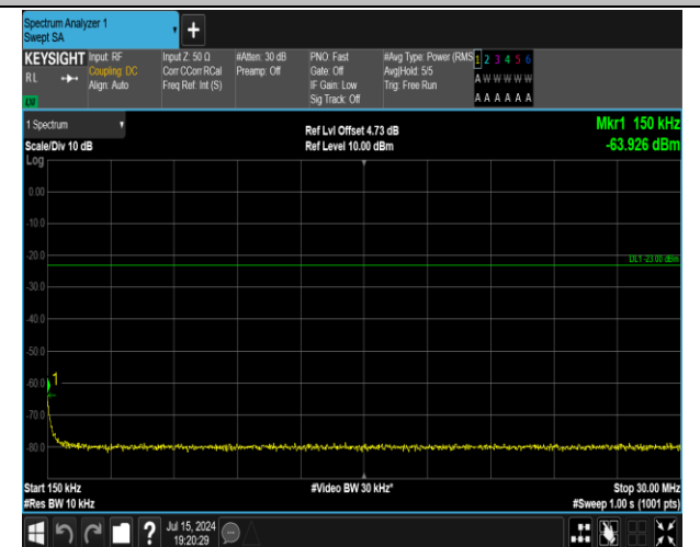
5-5-5MHz-3MHz-16QAM-16QAM-20595-20634-1RB#0-0R B#0-0.15~30MHz-PASS
