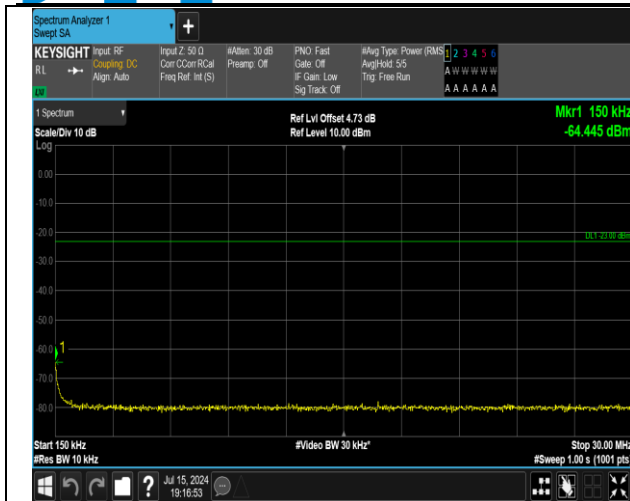
5-5-5MHz-3MHz-QPSK-QPSK-20510-20549-25RB#0-15R B#0-0.15~30MHz-PASS
