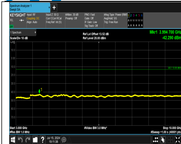
5-5-5MHz-3MHz-16QAM-16QAM-20510-20549-1RB#0-0R B#0-3000~10000MHz-PASS
