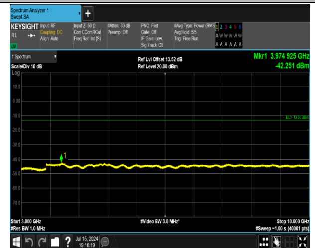
5-5-5MHz-3MHz-16QAM-16QAM-20510-20549-1RB#0-1R B#15-3000~10000MHz-PASS
