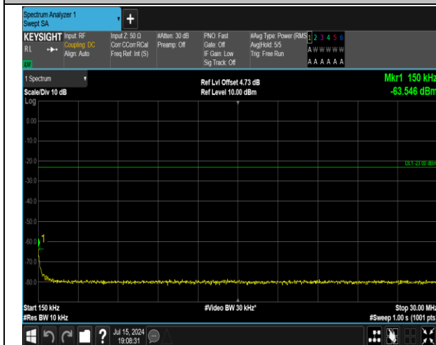
5-5-5MHz-3MHz-16QAM-16QAM-20425-20464-25RB#0-1 5RB#0-0.15~30MHz-PASS
