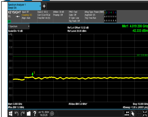
5-5-5MHz-3MHz-16QAM-16QAM-20595-20634-1RB#24-0 RB#0-3000~10000MHz-PASS
