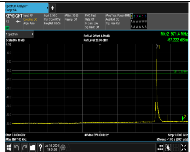
5-5-5MHz-3MHz-16QAM-16QAM-20425-20464-1RB#24-0 RB#0-30~1000MHz-PASS
