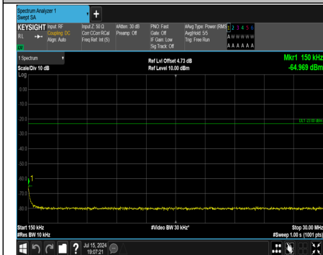
5-5-5MHz-3MHz-QPSK-QPSK-20425-20464-25RB#0-15R B#0-0.15~30MHz-PASS
