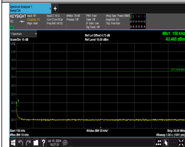
5-5-5MHz-3MHz-16QAM-16QAM-20595-20634-25RB#0-1 5RB#0-0.15~30MHz-PASS
