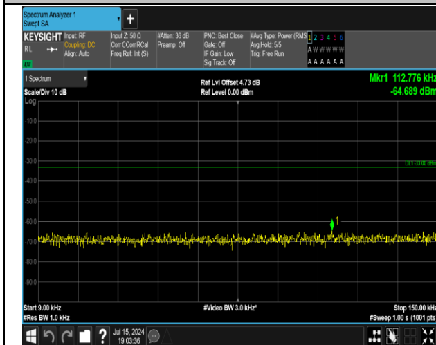
5-5-5MHz-3MHz-16QAM-16QAM-20425-20464-1RB#24-0 RB#0-0.009~0.15MHz-PASS
