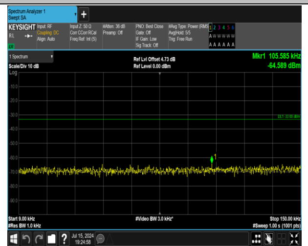
5-5-5MHz-3MHz-16QAM-16QAM-20595-20634-1RB#0-1R B#15-0.009~0.15MHz-PASS
