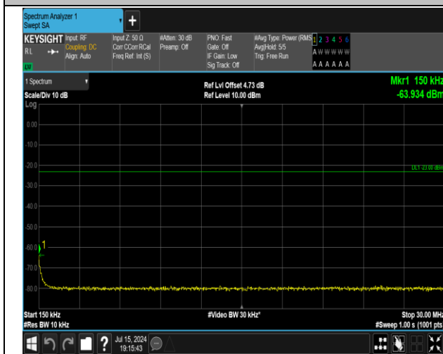
5-5-5MHz-3MHz-16QAM-16QAM-20510-20549-1RB#0-1R B#15-0.15~30MHz-PASS
