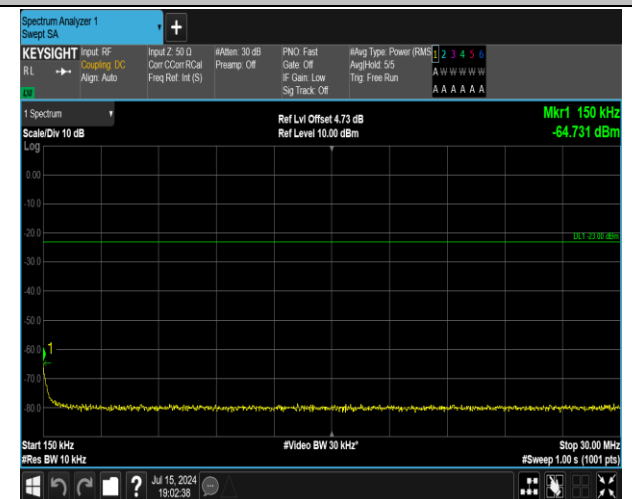
5-5-5MHz-3MHz-QPSK-QPSK-20425-20464-1RB#24-0RB #0-0.15~30MHz-PASS
