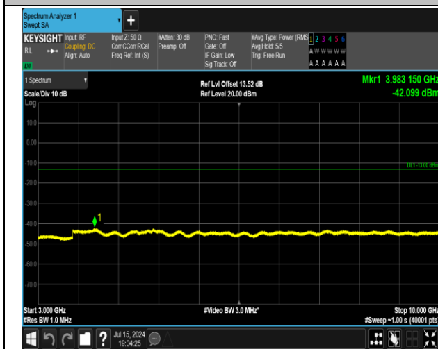
5-5-5MHz-3MHz-16QAM-16QAM-20425-20464-1RB#24-0 RB#0-3000~10000MHz-PASS
