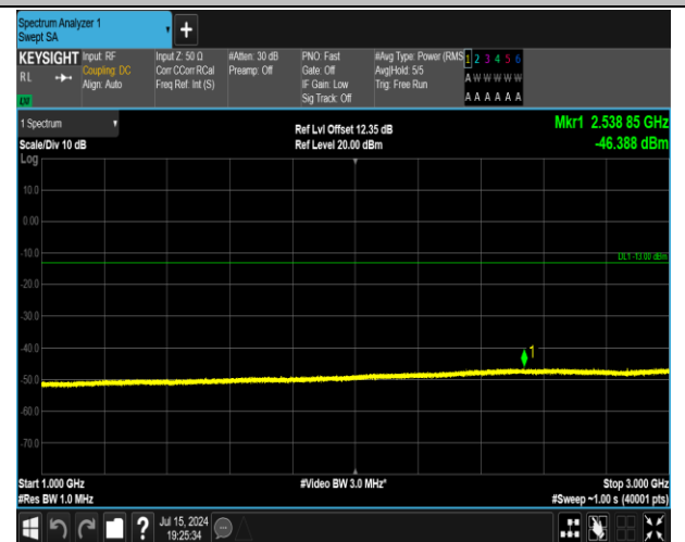
5-5-5MHz-3MHz-16QAM-16QAM-20595-20634-1RB#0-1R B#15-1000~3000MHz-PASS
