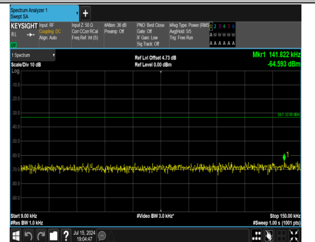
5-5-5MHz-3MHz-QPSK-QPSK-20425-20464-1RB#0-1RB# 15-0.009~0.15MHz-PASS
