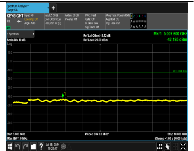
5-5-5MHz-3MHz-16QAM-16QAM-20595-20634-1RB#0-1R B#15-3000~10000MHz-PASS
