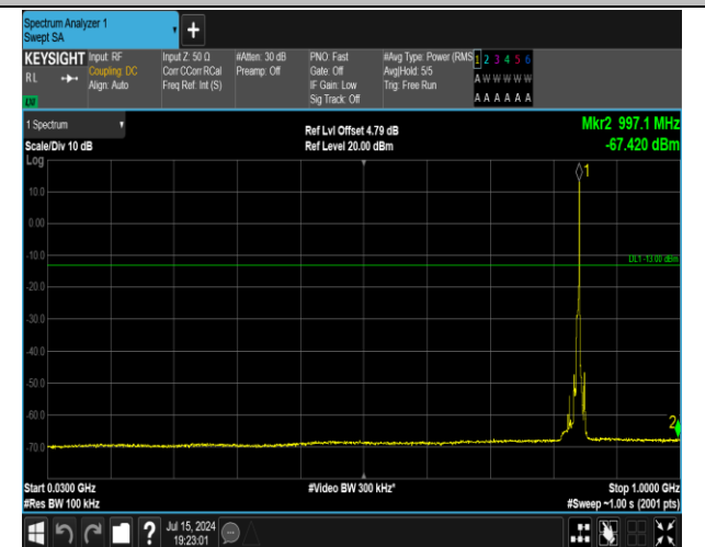
5-5-5MHz-3MHz-16QAM-16QAM-20595-20634-1RB#24-0 RB#0-30~1000MHz-PASS
