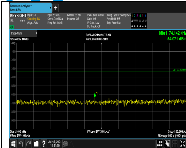
5-5-5MHz-3MHz-QPSK-QPSK-20510-20549-1RB#24-0RB #0-0.009~0.15MHz-PASS
