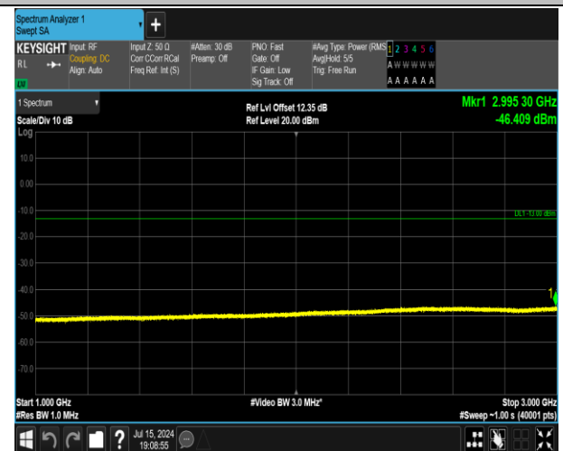
5-5-5MHz-3MHz-16QAM-16QAM-20425-20464-25RB#0-1 5RB#0-1000~3000MHz-PASS
