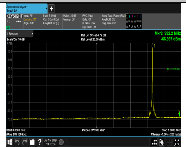
5-5-5MHz-3MHz-16QAM-16QAM-20510-20549-1RB#24-0 RB#0-30~1000MHz-PASS
