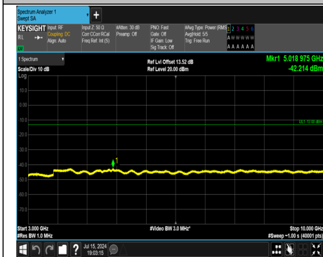
5-5-5MHz-3MHz-QPSK-QPSK-20425-20464-1RB#24-0RB #0-3000~10000MHz-PASS
