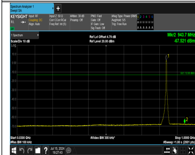
5-5-5MHz-3MHz-16QAM-16QAM-20595-20634-25RB#0-1 5RB#0-30~1000MHz-PASS
