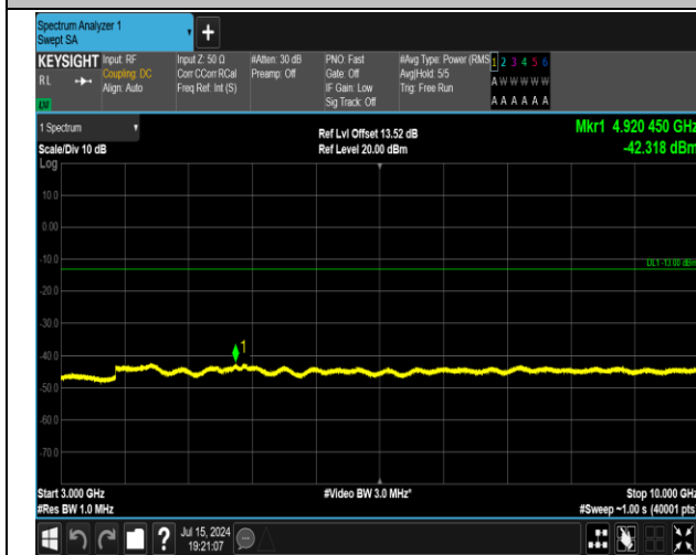
5-5-5MHz-3MHz-16QAM-16QAM-20595-20634-1RB#0-0R B#0-3000~10000MHz-PASS
