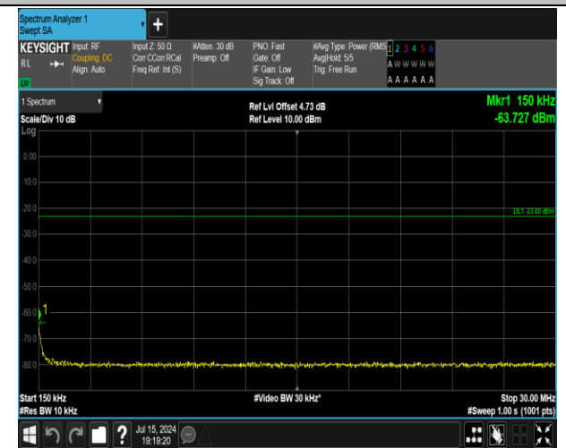
5-5-5MHz-3MHz-QPSK-QPSK-20595-20634-1RB#0-0RB# 0-0.15~30MHz-PASS
