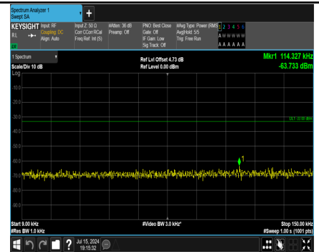
5-5-5MHz-3MHz-16QAM-16QAM-20510-20549-1RB#0-1R B#15-0.009~0.15MHz-PASS
