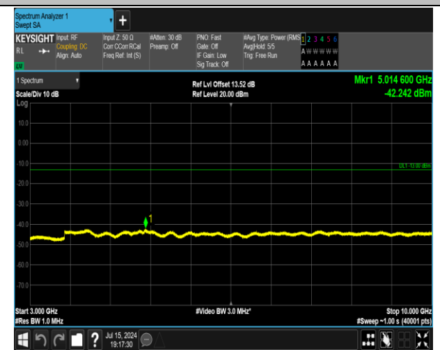
5-5-5MHz-3MHz-QPSK-QPSK-20510-20549-25RB#0-15R B#0-3000~10000MHz-PASS
