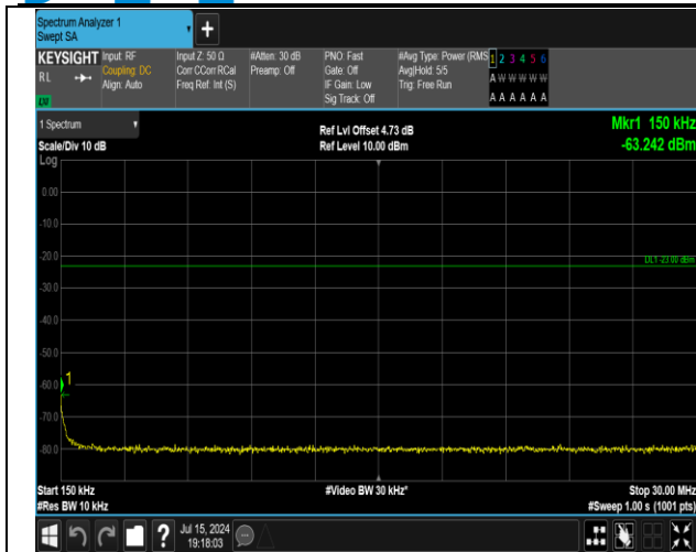
5-5-5MHz-3MHz-16QAM-16QAM-20510-20549-25RB#0-1 5RB#0-0.15~30MHz-PASS
