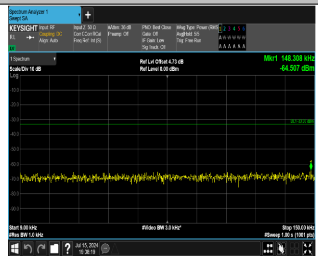
5-5-5MHz-3MHz-16QAM-16QAM-20425-20464-25RB#0-1 5RB#0-0.009~0.15MHz-PASS
