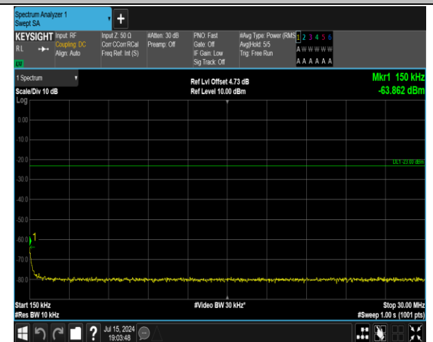
5-5-5MHz-3MHz-16QAM-16QAM-20425-20464-1RB#24-0 RB#0-0.15~30MHz-PASS
