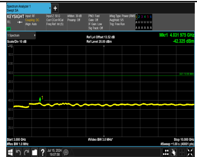
5-5-5MHz-3MHz-QPSK-QPSK-20425-20464-25RB#0-15R B#0-3000~10000MHz-PASS
