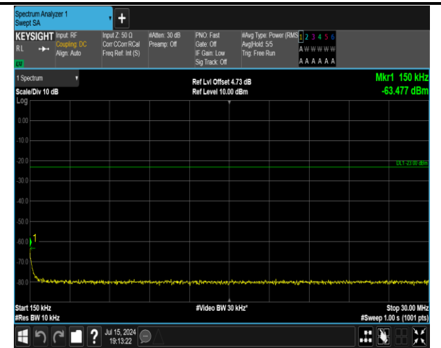
5-5-5MHz-3MHz-16QAM-16QAM-20510-20549-1RB#24-0 RB#0-0.15~30MHz-PASS
