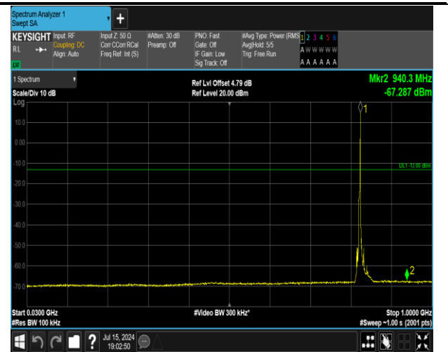
5-5-5MHz-3MHz-QPSK-QPSK-20425-20464-1RB#24-0RB #0-30~1000MHz-PASS
