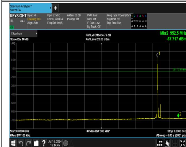
5-5-5MHz-3MHz-QPSK-QPSK-20510-20549-1RB#0-1RB# 15-30~1000MHz-PASS
