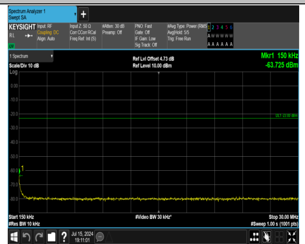
5-5-5MHz-3MHz-16QAM-16QAM-20510-20549-1RB#0-0R B#0-0.15~30MHz-PASS
