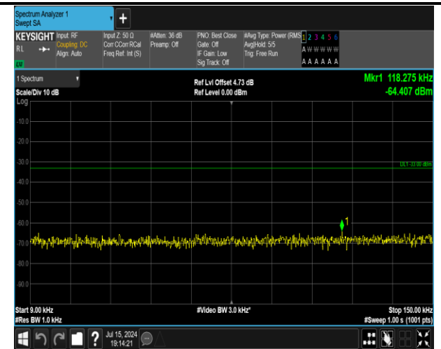
5-5-5MHz-3MHz-QPSK-QPSK-20510-20549-1RB#0-1RB# 15-0.009~0.15MHz-PASS
