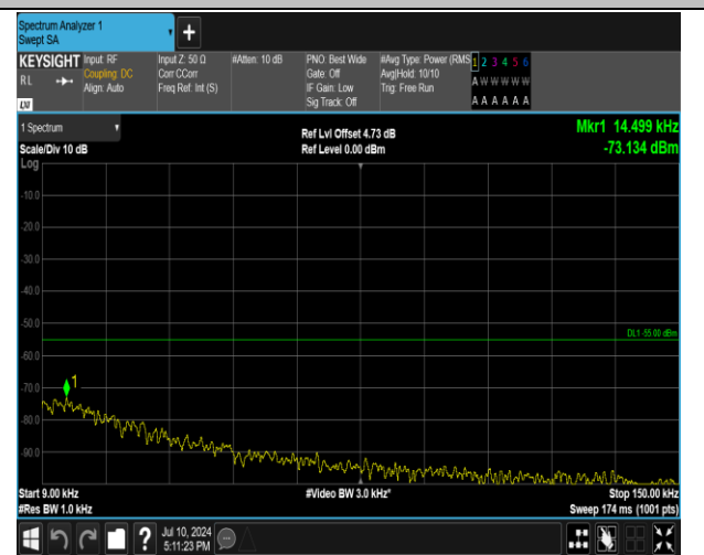
7-7-15MHz-10MHz-QPSK-QPSK-20825-20945-75RB#0-50 RB#0-0.009~0.15MHz-PASS
