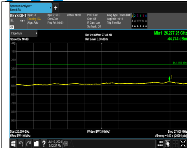
7-7-15MHz-10MHz-QPSK-QPSK-20825-20945-75RB#0-5 ORB#0-20000~27000MHz-PASS
