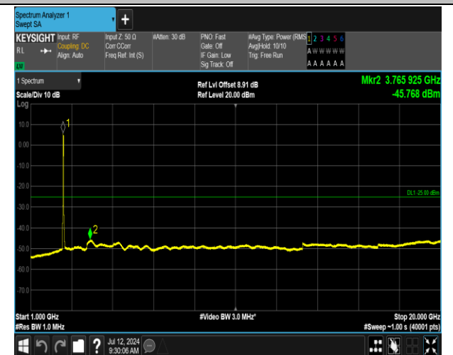
7-7-15MHz-15MHz-16QAM-16QAM-20825-20975-75RB#0 -75RB#0-1000~20000MHz-PASS
