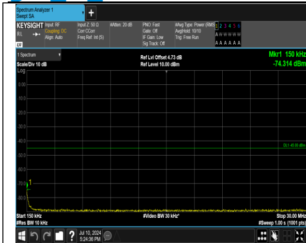
7-7-15MHz-10MHz-QPSK-QPSK-21051-21171-75RB#0-5 ORB#0-0.15~30MHz-PASS
