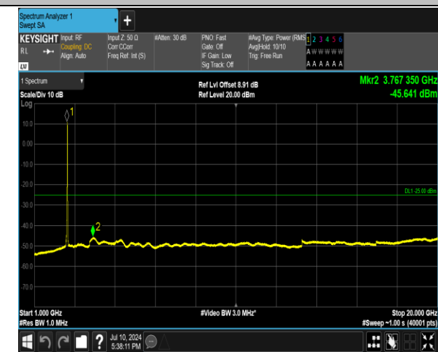
7-7-15MHz-10MHz-QPSK-QPSK-21277-21397-75RB#0-50 RB#0-1000~20000MHz-PASS
