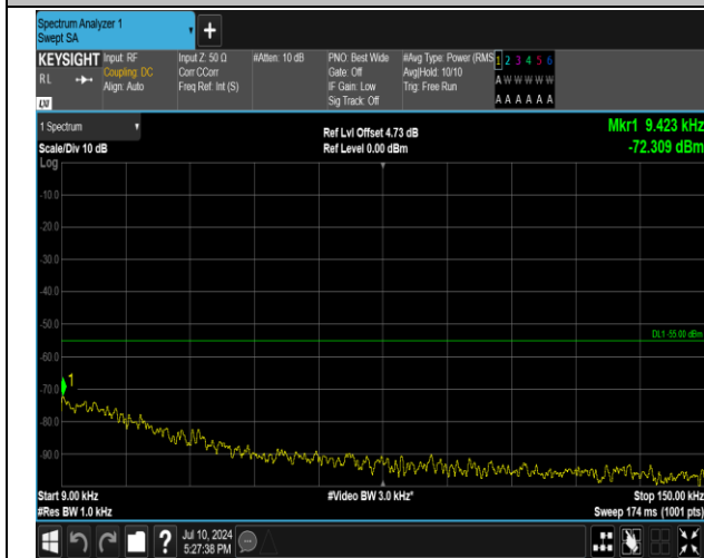
7-7-15MHz-10MHz-QPSK-QPSK-21277-21397-1RB#0-0R B#0-0.009~0.15MHz-PASS
