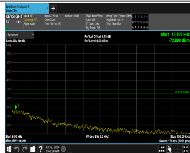
7-7-15MHz-15MHz-16QAM-16QAM-21025-21175-75RB#0 -75RB#0-0.009~0.15MHz-PASS
