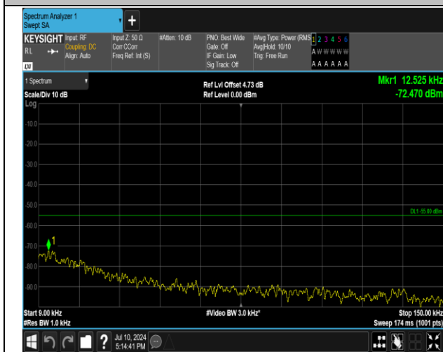
7-7-15MHz-10MHz-QPSK-QPSK-21051-21171-1RB#0-0R B#0-0.009~0.15MHz-PASS
