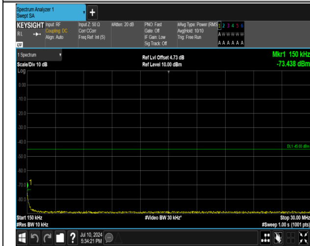
7-7-15MHz-10MHz-QPSK-QPSK-21277-21397-1RB#0-1R B#49-0.15~30MHz-PASS
