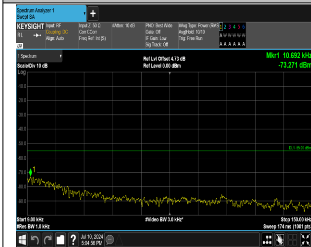
7-7-15MHz-10MHz-QPSK-QPSK-20825-20945-1RB#74-0 RB#0-0.009~0.15MHz-PASS
