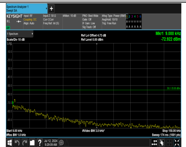
7-7-15MHz-15MHz-16QAM-16QAM-20825-20975-75RB#0 -75RB#0-0.009~0.15MHz-PASS
