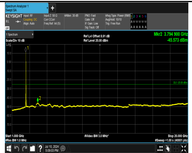
7-7-15MHz-10MHz-QPSK-QPSK-20825-20945-1RB#0-1R B#49-1000~20000MHz-PASS
