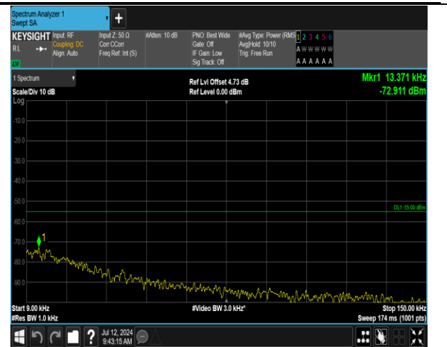
7-7-15MHz-15MHz-16QAM-16QAM-21025-21175-1RB#0- 1RB#74-0.009~0.15MHz-PASS
