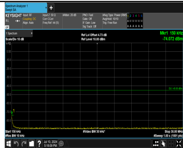
7-7-15MHz-10MHz-QPSK-QPSK-21051-21171-1RB#74-0 RB#0-0.15~30MHz-PASS
