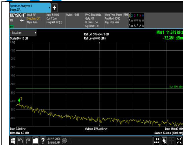
7-7-15MHz-15MHz-16QAM-16QAM-21025-21175-1RB#74 -ORB#0-0.009~0.15MHz-PASS
