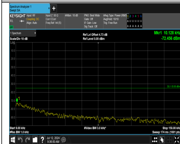
7-7-15MHz-15MHz-16QAM-16QAM-21025-21175-1RB#0- ORB#0-0.009~0.15MHz-PASS
