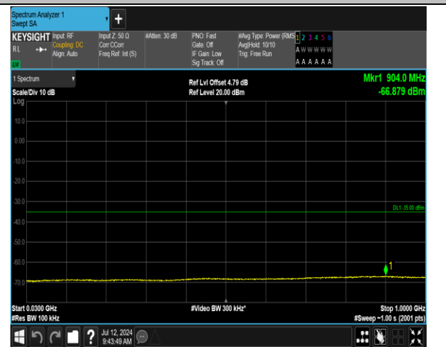
7-7-15MHz-15MHz-16QAM-16QAM-21025-21175-1RB#0- 1RB#74-30~1000MHz-PASS
