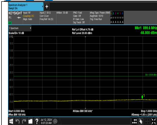
7-7-15MHz-15MHz-16QAM-16QAM-21025-21175-1RB#0- ORB#0-30~1000MHz-PASS
