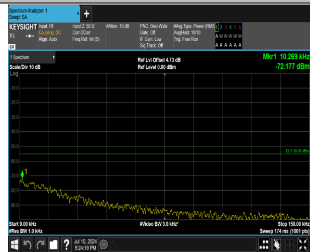
7-7-15MHz-10MHz-QPSK-QPSK-21051-21171-75RB#0-50 RB#0-0.009~0.15MHz-PASS
