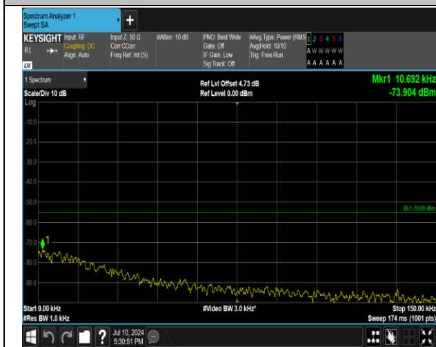
7-7-15MHz-10MHz-QPSK-QPSK-21277-21397-1RB#74-0 RB#0-0.009~0.15MHz-PASS
