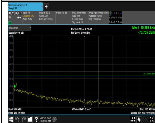
7-7-15MHz-15MHz-16QAM-16QAM-21225-21375-1RB#0- ORB#0-0.009~0.15MHz-PASS
