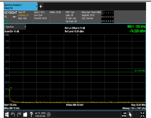
7-7-15MHz-15MHz-16QAM-16QAM-21225-21375-1RB#0- ORB#0-0.15~30MHz-PASS
