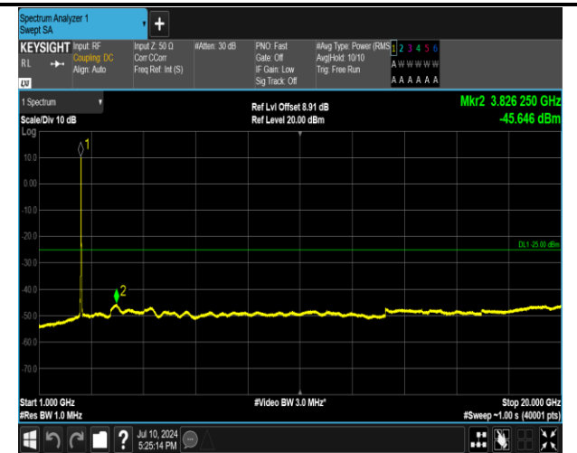
7-7-15MHz-10MHz-QPSK-QPSK-21051-21171-75RB#0-50 RB#0-1000~20000MHz-PASS
