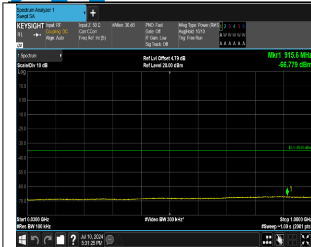
7-7-15MHz-10MHz-QPSK-QPSK-21277-21397-1RB#74-0 RB#0-30~1000MHz-PASS
