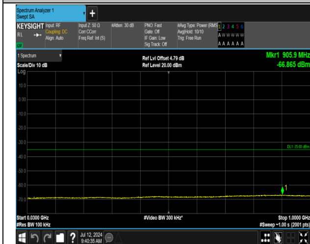
7-7-15MHz-15MHz-16QAM-16QAM-21025-21175-1RB#74 -ORB#0-30~1000MHz-PASS
