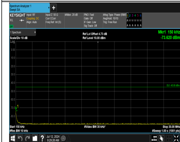
7-7-15MHz-15MHz-16QAM-16QAM-20825-20975-75RB# 0-75RB#0-0.15~30MHz-PASS
