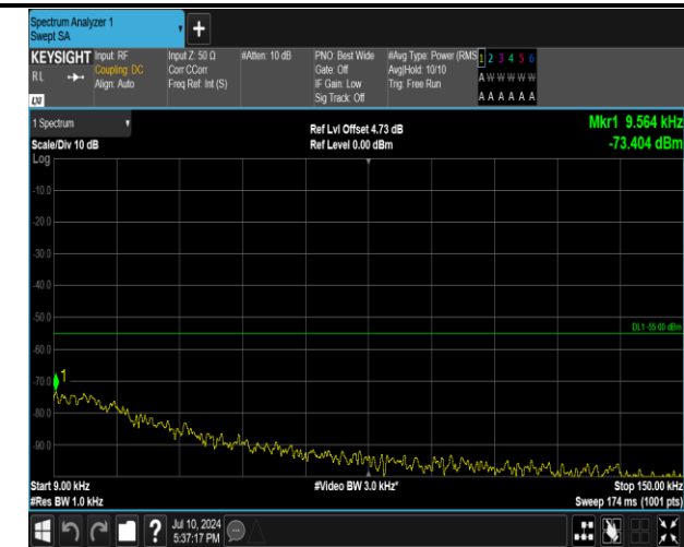
7-7-15MHz-10MHz-QPSK-QPSK-21277-21397-75RB#0-50 RB#0-0.009~0.15MHz-PASS
