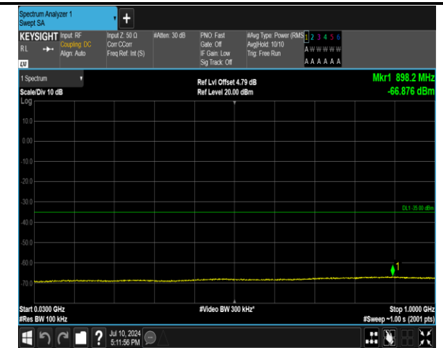
7-7-15MHz-10MHz-QPSK-QPSK-20825-20945-75RB#0-50 RB#0-30~1000MHz-PASS
