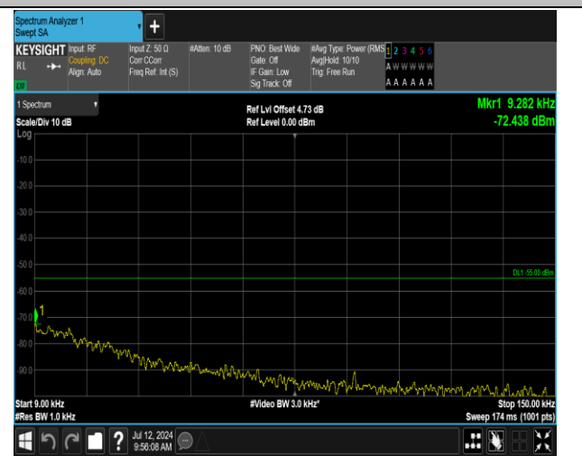
7-7-15MHz-15MHz-16QAM-16QAM-21225-21375-1RB#0- 1RB#74-0.009~0.15MHz-PASS
