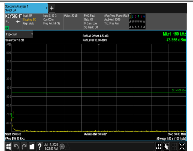
7-7-15MHz-15MHz-16QAM-16QAM-20825-20975-1RB#74 -ORB#0-0.15~30MHz-PASS
