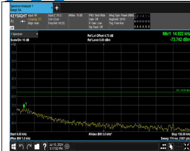
7-7-15MHz-10MHz-QPSK-QPSK-21051-21171-1RB#74-0 RB#0-0.009~0.15MHz-PASS
