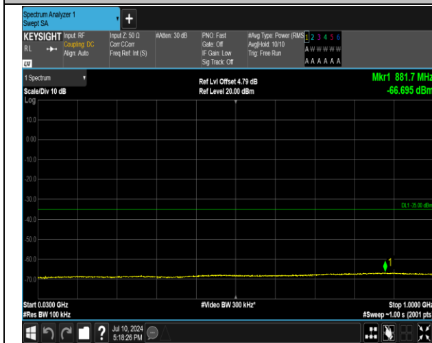
7-7-15MHz-10MHz-QPSK-QPSK-21051-21171-1RB#74-0 RB#0-30~1000MHz-PASS
