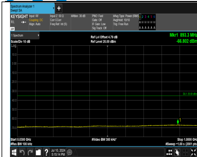
7-7-15MHz-10MHz-QPSK-QPSK-21051-21171-1RB#0-0R B#0-30~1000MHz-PASS
