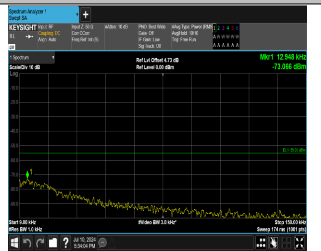
7-7-15MHz-10MHz-QPSK-QPSK-21277-21397-1RB#0-1R B#49-0.009~0.15MHz-PASS
