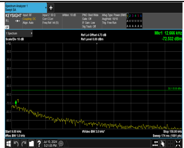
7-7-15MHz-10MHz-QPSK-QPSK-21051-21171-1RB#0-1R B#49-0.009~0.15MHz-PASS
