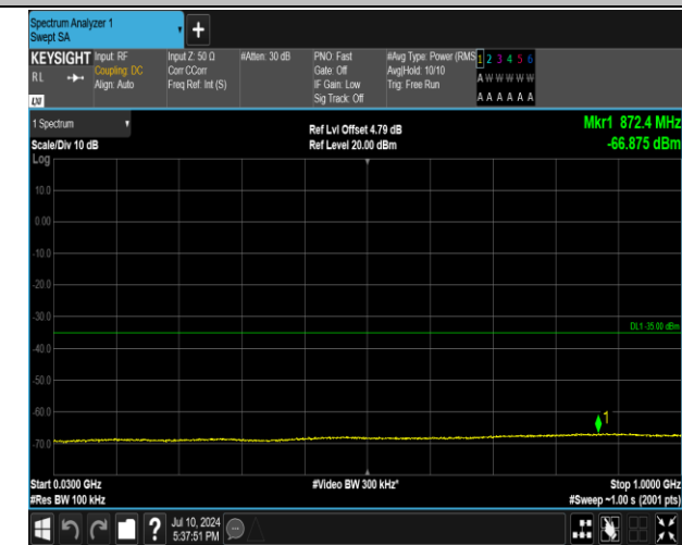
7-7-15MHz-10MHz-QPSK-QPSK-21277-21397-75RB#0-50 RB#0-30~1000MHz-PASS
