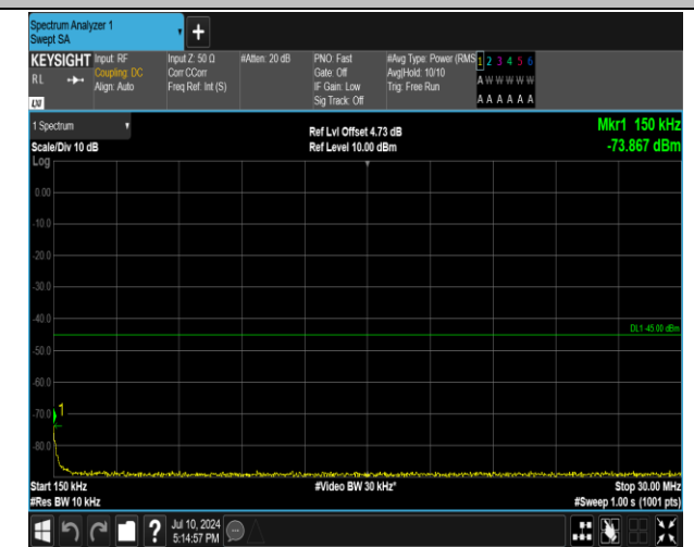
7-7-15MHz-10MHz-QPSK-QPSK-21051-21171-1RB#0-0R B#0-0.15~30MHz-PASS
