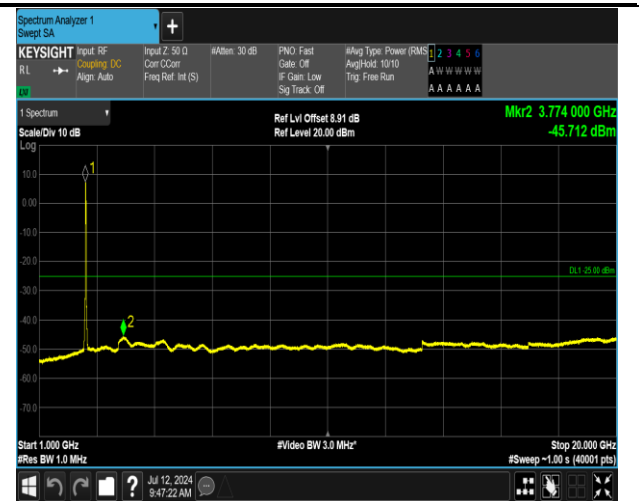
7-7-15MHz-15MHz-16QAM-16QAM-21025-21175-75RB#0 -75RB#0-1000~20000MHz-PASS
