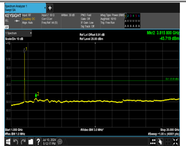
7-7-15MHz-10MHz-QPSK-QPSK-20825-20945-75RB#0-50 RB#0-1000~20000MHz-PASS
