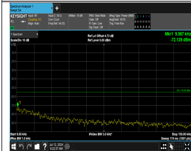
7-7-15MHz-15MHz-16QAM-16QAM-20825-20975-1RB#7 4-ORB#0-0.009~0.15MHz-PASS
