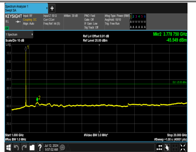
7-7-15MHz-15MHz-16QAM-16QAM-21225-21375-1RB#0- 1RB#74-1000~20000MHz-PASS
