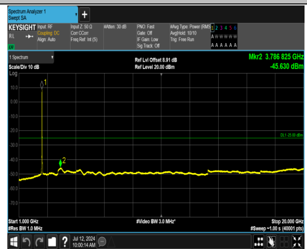
7-7-15MHz-15MHz-16QAM-16QAM-21225-21375-75RB#0 -75RB#0-1000~20000MHz-PASS
