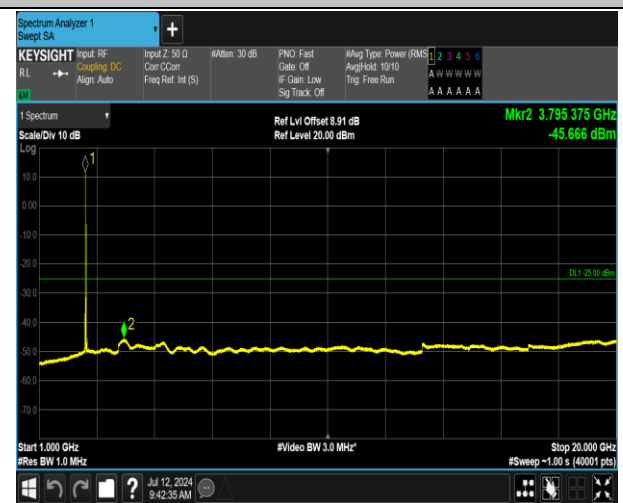
7-7-15MHz-15MHz-QPSK-QPSK-21025-21175-1RB#0-1R B#74-1000~20000MHz-PASS
