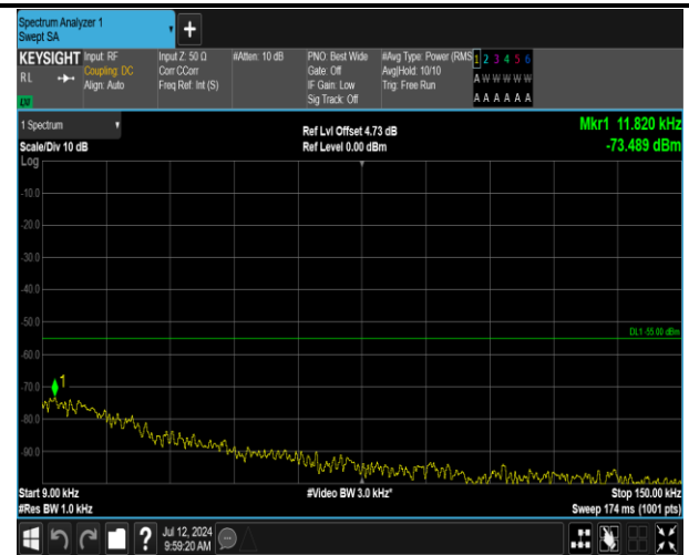
7-7-15MHz-15MHz-16QAM-16QAM-21225-21375-75RB#0 -75RB#0-0.009~0.15MHz-PASS
