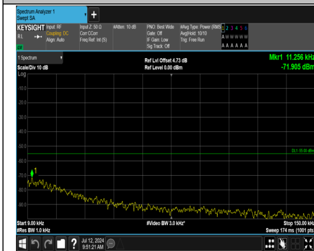
7-7-15MHz-15MHz-QPSK-QPSK-21225-21375-1RB#74-0 RB#0-0.009~0.15MHz-PASS
