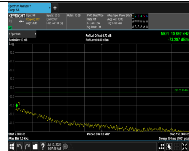
7-7-15MHz-15MHz-QPSK-QPSK-21225-21375-75RB#0-75 RB#0-0.009~0.15MHz-PASS
