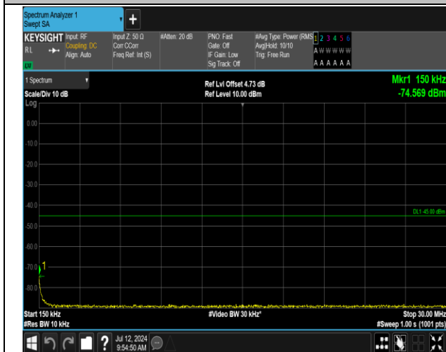
7-7-15MHz-15MHz-QPSK-QPSK-21225-21375-1RB#0-1R B#74-0.15~30MHz-PASS
