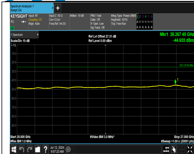
7-7-15MHz-15MHz-16QAM-16QAM-21225-21375-1RB#0-1RB#74-20000~27000MHz-PASS
