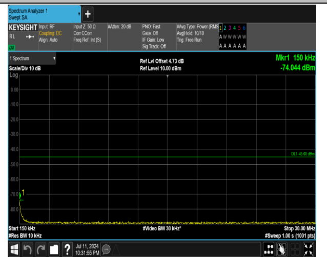
7-7-15MHz-20MHz-16QAM-16QAM-20828-20999-1RB#74-ORB#0-0.15~30MHz-PASS
