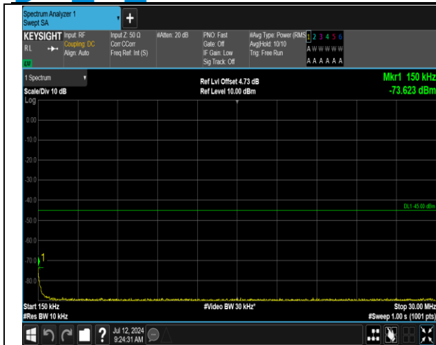
7-7-15MHz-15MHz-QPSK-QPSK-20825-20975-1RB#0-1R B#74-0.15~30MHz-PASS
