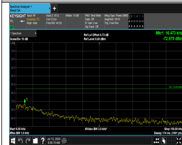
7-7-15MHz-15MHz-QPSK-QPSK-21025-21175-1RB#0-0R B#0-0.009~0.15MHz-PASS
