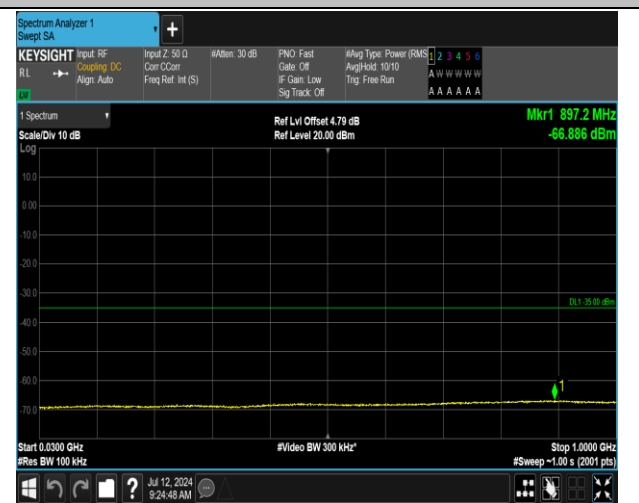
7-7-15MHz-15MHz-QPSK-QPSK-20825-20975-1RB#0-1R B#74-30~1000MHz-PASS
