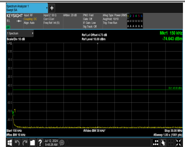
7-7-15MHz-15MHz-QPSK-QPSK-21225-21375-1RB#0-0R B#0-0.15~30MHz-PASS
