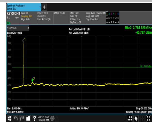
7-7-15MHz-15MHz-QPSK-QPSK-21225-21375-75RB#0-75 RB#0-1000~20000MHz-PASS
