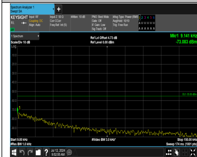
7-7-15MHz-15MHz-16QAM-16QAM-21225-21375-1RB#74-4-ORB#0-0.009~0.15MHz-PASS
