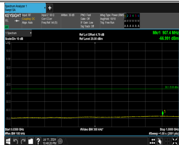
7-7-15MHz-20MHz-16QAM-16QAM-21003-21174-1RB#0- 1RB#99-30~1000MHz-PASS
