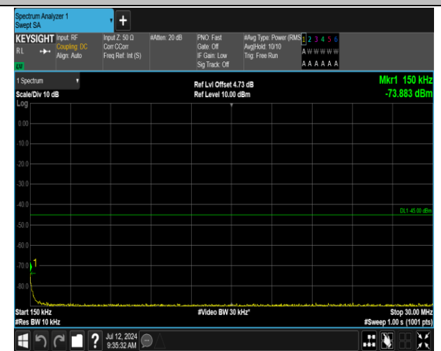
7-7-15MHz-15MHz-QPSK-QPSK-21025-21175-1RB#0-0R B#0-0.15~30MHz-PASS
