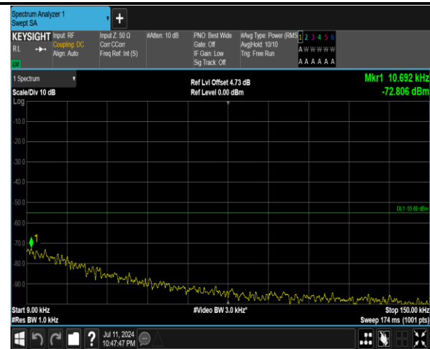
7-7-15MHz-20MHz-16QAM-16QAM-21003-21174-1RB#0- 1RB#99-0.009~0.15MHz-PASS
