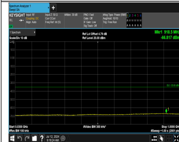
7-7-15MHz-15MHz-QPSK-QPSK-20825-20975-1RB#0-0R B#0-30~1000MHz-PASS
