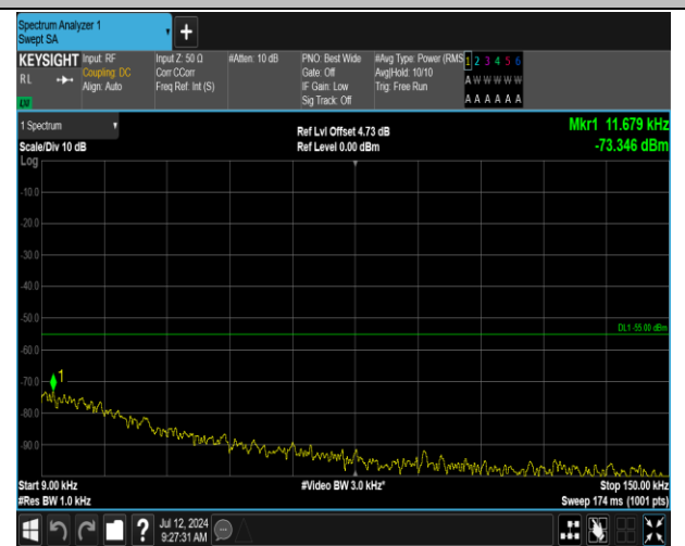
7-7-15MHz-15MHz-QPSK-QPSK-20825-20975-75RB#0-75 RB#0-0.009~0.15MHz-PASS
