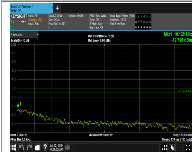
7-7-15MHz-15MHz-QPSK-QPSK-20825-20975-1RB#74-0 RB#0-0.009~0.15MHz-PASS
