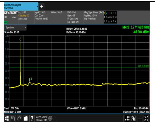
7-7-15MHz-20MHz-16QAM-16QAM-20828-20999-1RB#0-1RB#99-1000~20000MHz-PASS
