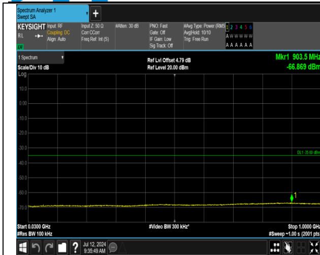
7-7-15MHz-15MHz-QPSK-QPSK-21025-21175-1RB#0-0R B#0-30~1000MHz-PASS
