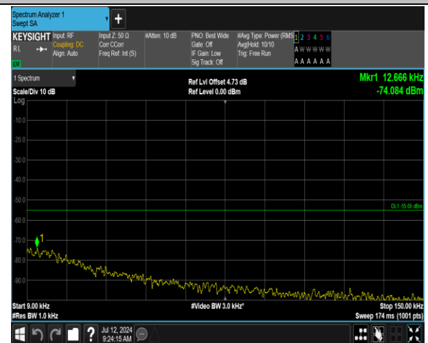
7-7-15MHz-15MHz-QPSK-QPSK-20825-20975-1RB#0-1R B#74-0.009~0.15MHz-PASS
