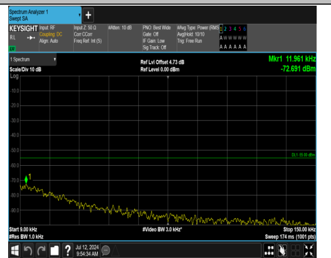
7-7-15MHz-15MHz-QPSK-QPSK-21225-21375-1RB#0-1R B#74-0.009~0.15MHz-PASS
