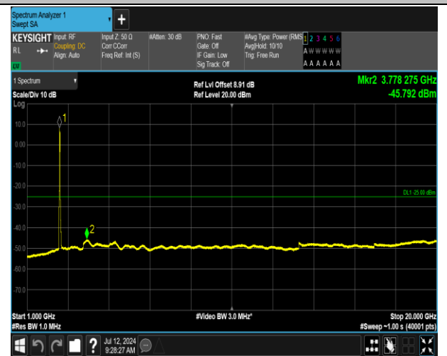
7-7-15MHz-15MHz-QPSK-QPSK-20825-20975-75RB#0-75 RB#0-1000~20000MHz-PASS
