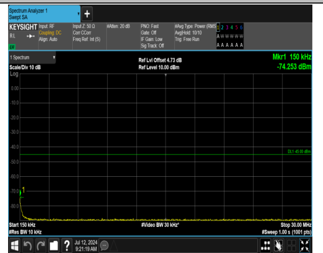
7-7-15MHz-15MHz-QPSK-QPSK-20825-20975-1RB#74-0 RB#0-0.15~30MHz-PASS
