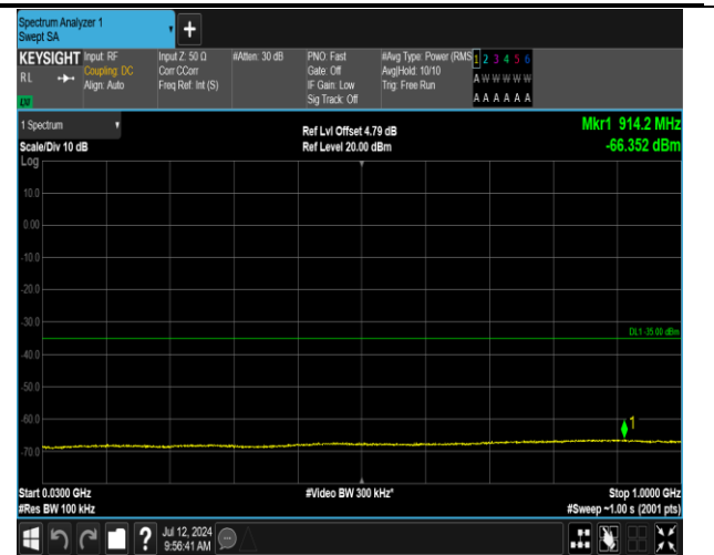
7-7-15MHz-15MHz-16QAM-16QAM-21225-21375-1RB#0-1RB#74-30~1000MHz-PASS
