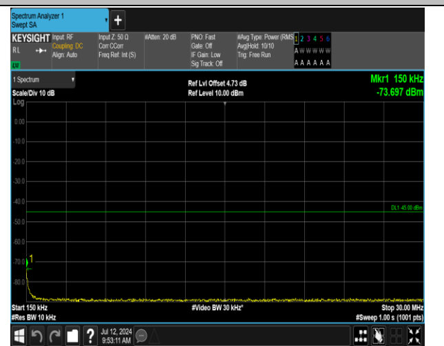
7-7-15MHz-15MHz-16QAM-16QAM-21225-21375-1RB#74-4-ORB#0-0.15~30MHz-PASS
