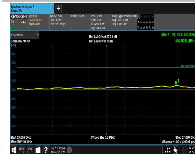
7-7-15MHz-20MHz-16QAM-16QAM-21003-21174-1RB#0- 1RB#99-20000~27000MHz-PASS
