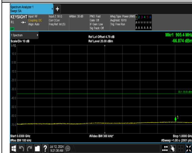
7-7-15MHz-15MHz-QPSK-QPSK-20825-20975-1RB#74-0 RB#0-30~1000MHz-PASS
