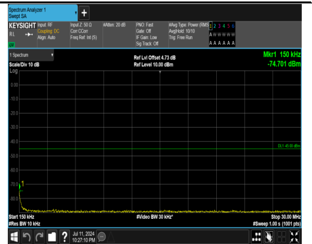
7-7-15MHz-20MHz-QPSK-QPSK-20828-20999-1RB#0-0R B#0-0.15~30MHz-PASS
