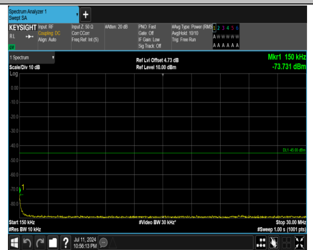
7-7-15MHz-20MHz-QPSK-QPSK-21179-21350-1RB#74-0 RB#0-0.15~30MHz-PASS
