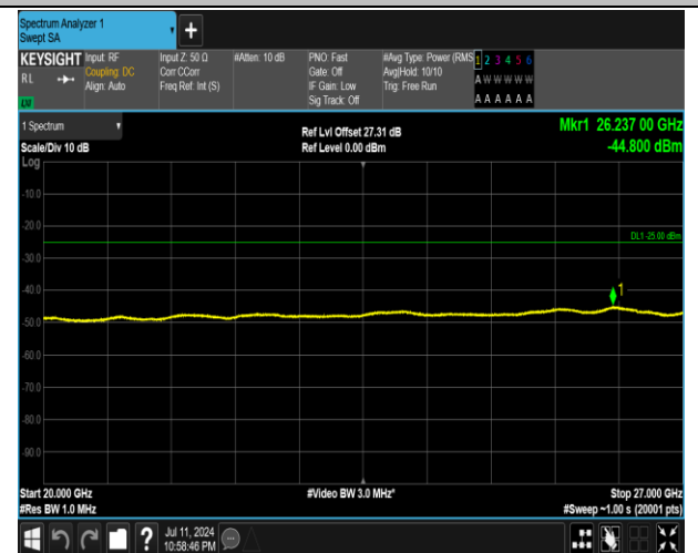
7-7-15MHz-20MHz-16QAM-16QAM-21179-21350-1RB#74-0RB#0-20000~27000MHz-PASS
