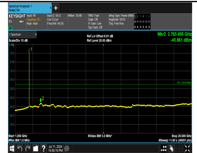
7-7-15MHz-20MHz-QPSK-QPSK-21003-21174-75RB#0-10 0RB#0-1000~20000MHz-PASS
