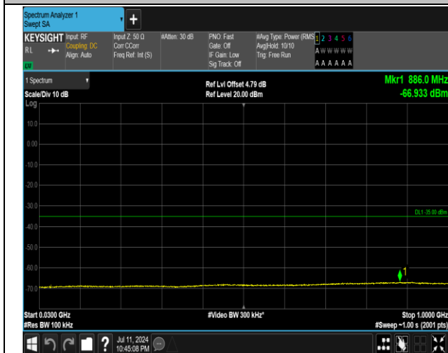
7-7-15MHz-20MHz-16QAM-16QAM-21003-21174-1RB#74 -ORB#0-30~1000MHz-PASS
