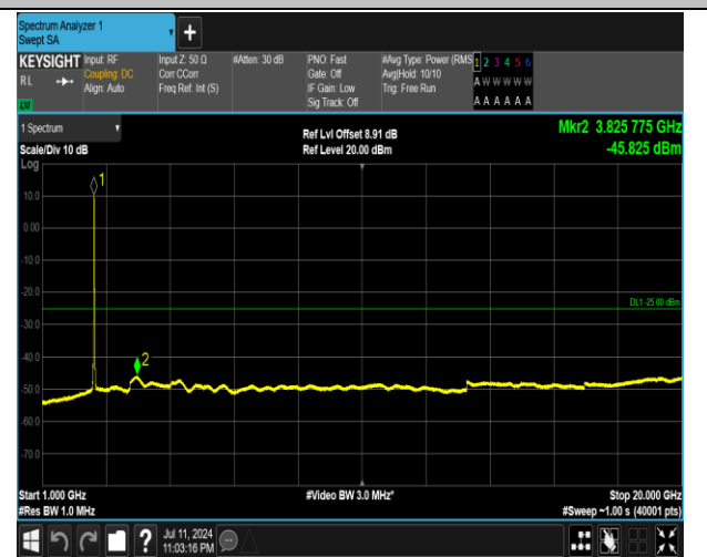
7-7-15MHz-20MHz-QPSK-QPSK-21179-21350-75RB#0-10 ORB#0-1000~20000MHz-PASS
