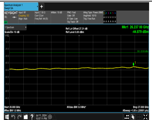
7-7-15MHz-20MHz-QPSK-QPSK-21179-21350-1RB#74-0 RB#0-20000~27000MHz-PASS
