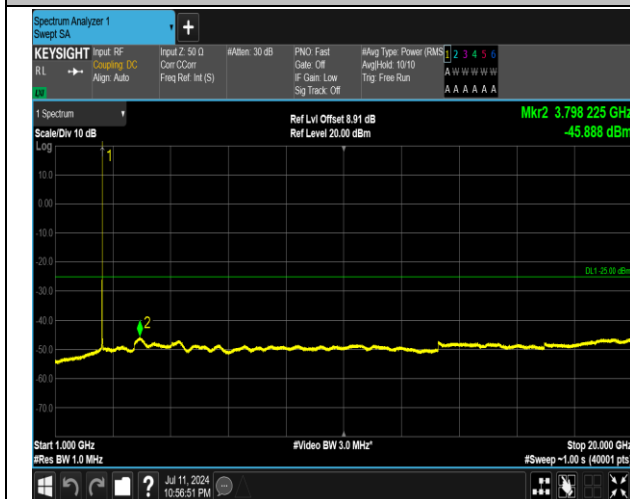
7-7-15MHz-20MHz-QPSK-QPSK-21179-21350-1RB#74-0 RB#0-1000~20000MHz-PASS
