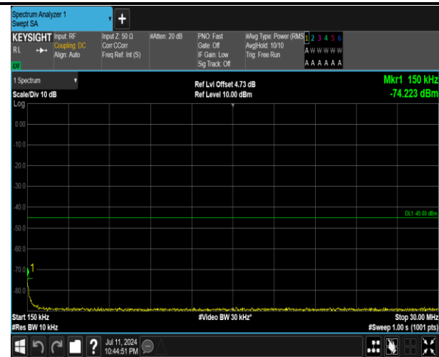
7-7-15MHz-20MHz-16QAM-16QAM-21003-21174-1RB#74 -ORB#0-0.15~30MHz-PASS
