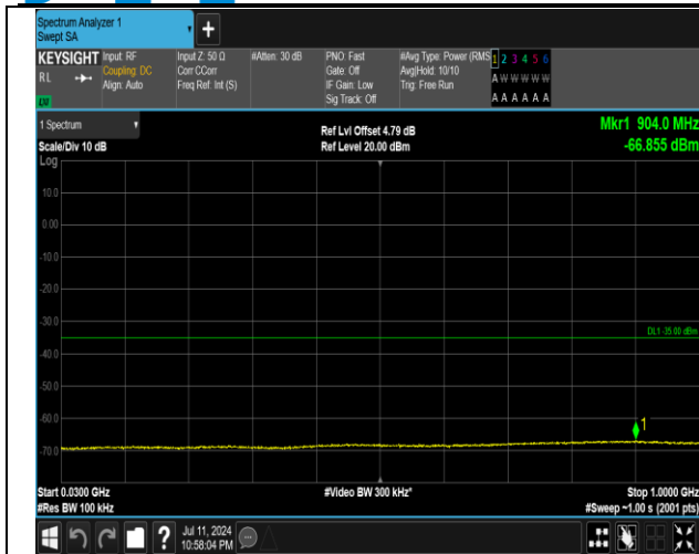
7-7-15MHz-20MHz-16QAM-16QAM-21179-21350-1RB#74 -0RB#0-30~1000MHz-PASS
