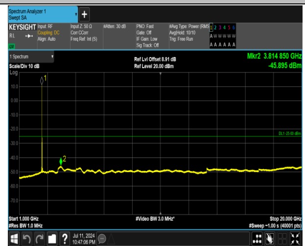
7-7-15MHz-20MHz-QPSK-QPSK-21003-21174-1RB#0-1R B#99-1000~20000MHz-PASS
