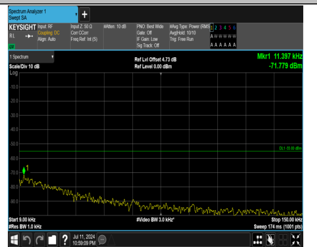
7-7-15MHz-20MHz-QPSK-QPSK-21179-21350-1RB#0-1R B#99-0.009~0.15MHz-PASS
