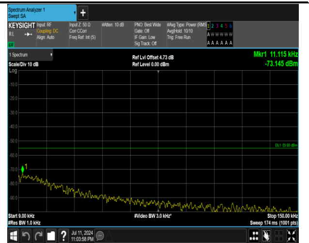
7-7-15MHz-20MHz-16QAM-16QAM-21179-21350-75RB#0 -100RB#0-0.009~0.15MHz-PASS
