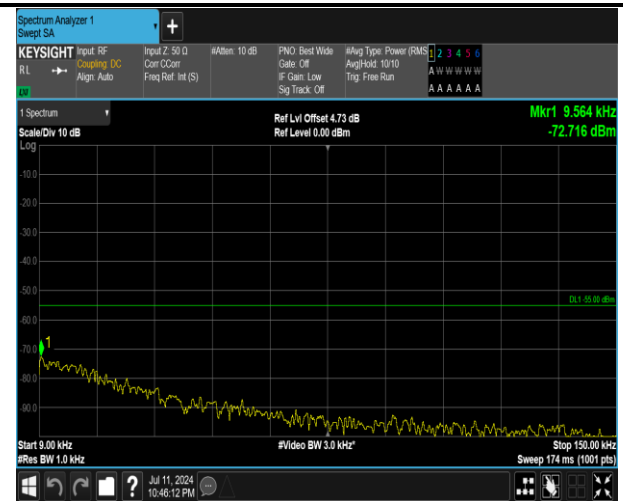
7-7-15MHz-20MHz-QPSK-QPSK-21003-21174-1RB#0-1R B#99-0.009~0.15MHz-PASS
