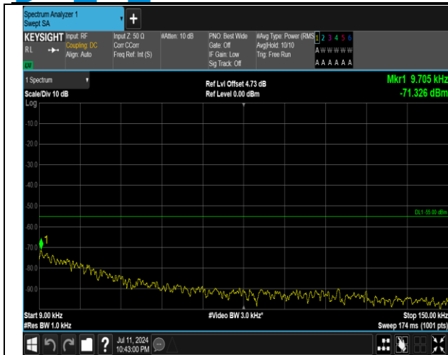
7-7-15MHz-20MHz-QPSK-QPSK-21003-21174-1RB#74-0 RB#0-0.009~0.15MHz-PASS
