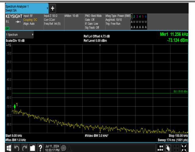
7-7-15MHz-20MHz-QPSK-QPSK-20828-20999-1RB#0-1R B#99-0.009~0.15MHz-PASS
