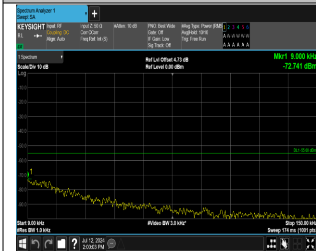
7-7-20MHz-10MHz-16QAM-16QAM-20850-20994-1RB#0- 1RB#49-0.009~0.15MHz-PASS
