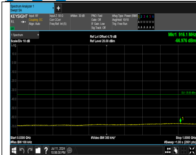
7-7-15MHz-20MHz-QPSK-QPSK-21179-21350-1RB#74-0 RB#0-30~1000MHz-PASS
