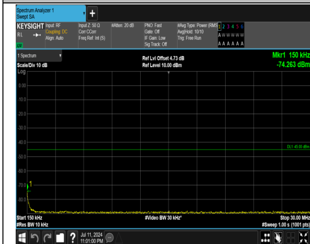
7-7-15MHz-20MHz-16QAM-16QAM-21179-21350-1RB#0- 1RB#99-0.15~30MHz-PASS
