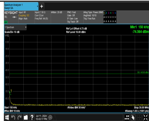
7-7-15MHz-20MHz-QPSK-QPSK-21003-21174-1RB#74-0 RB#0-0.15~30MHz-PASS
