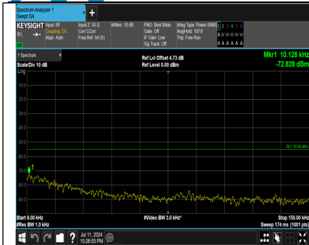
7-7-15MHz-20MHz-QPSK-QPSK-20828-20999-1RB#0-0R B#0-0.009~0.15MHz-PASS
