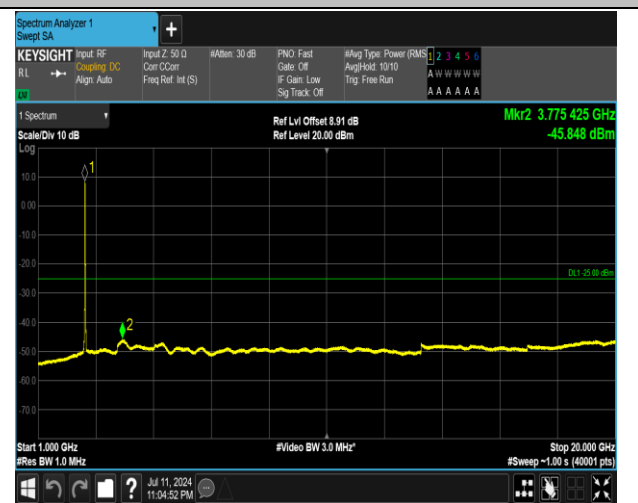
7-7-15MHz-20MHz-16QAM-16QAM-21179-21350-75RB#0 -100RB#0-1000~20000MHz-PASS
