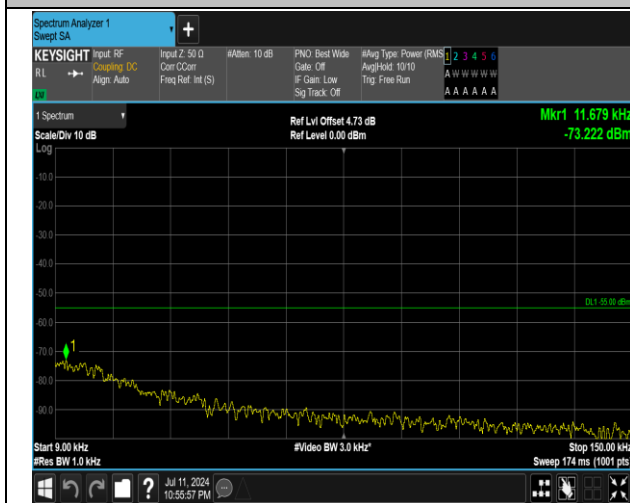
7-7-15MHz-20MHz-QPSK-QPSK-21179-21350-1RB#74-0 RB#0-0.009~0.15MHz-PASS
