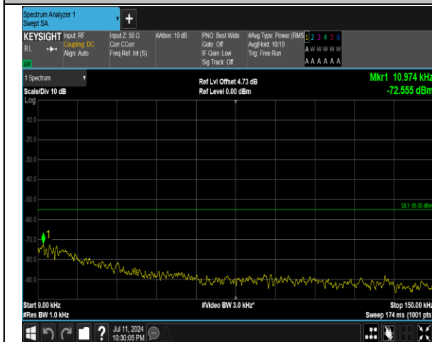
7-7-15MHz-20MHz-QPSK-QPSK-20828-20999-1RB#74-0 RB#0-0.009~0.15MHz-PASS
