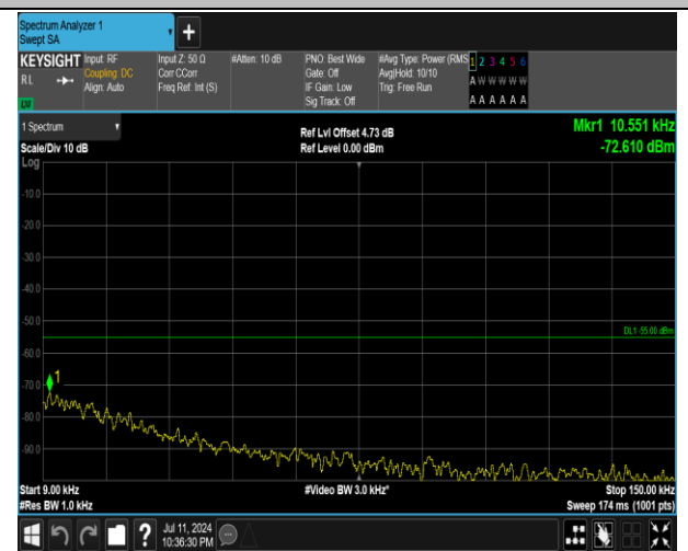
7-7-15MHz-20MHz-QPSK-QPSK-20828-20999-75RB#0-10 ORB#0-0.009~0.15MHz-PASS
