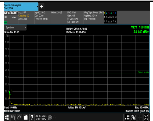
7-7-20MHz-10MHz-16QAM-16QAM-20850-20994-1RB#0- 1RB#49-0.15~30MHz-PASS
