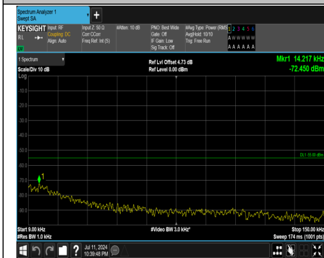
7-7-15MHz-20MHz-QPSK-QPSK-21003-21174-1RB#0-0R B#0-0.009~0.15MHz-PASS
