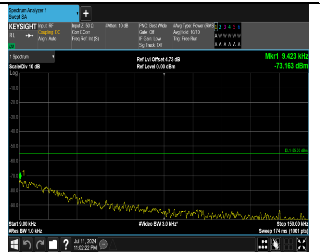
7-7-15MHz-20MHz-QPSK-QPSK-21179-21350-75RB#0-10 ORB#0-0.009~0.15MHz-PASS
