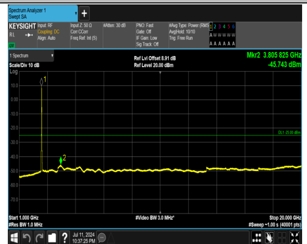
7-7-15MHz-20MHz-QPSK-QPSK-20828-20999-75RB#0-10 ORB#0-1000~20000MHz-PASS
