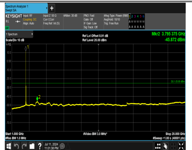
7-7-15MHz-20MHz-16QAM-16QAM-21179-21350-1RB#0- 1RB#99-1000~20000MHz-PASS
