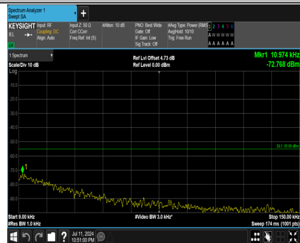
7-7-15MHz-20MHz-16QAM-16QAM-21003-21174-75RB#0 -100RB#0-0.009~0.15MHz-PASS
