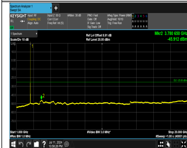
7-7-15MHz-20MHz-16QAM-16QAM-21179-21350-1RB#74-0RB#0-1000~20000MHz-PASS
