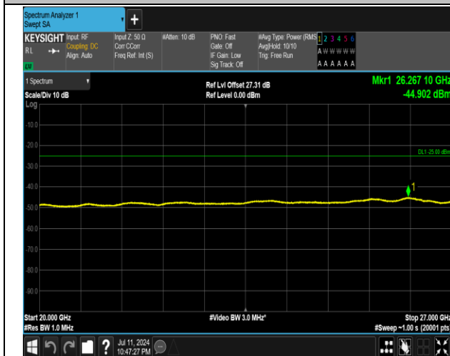
7-7-15MHz-20MHz-QPSK-QPSK-21003-21174-1RB#0-1R B#99-20000~27000MHz-PASS
