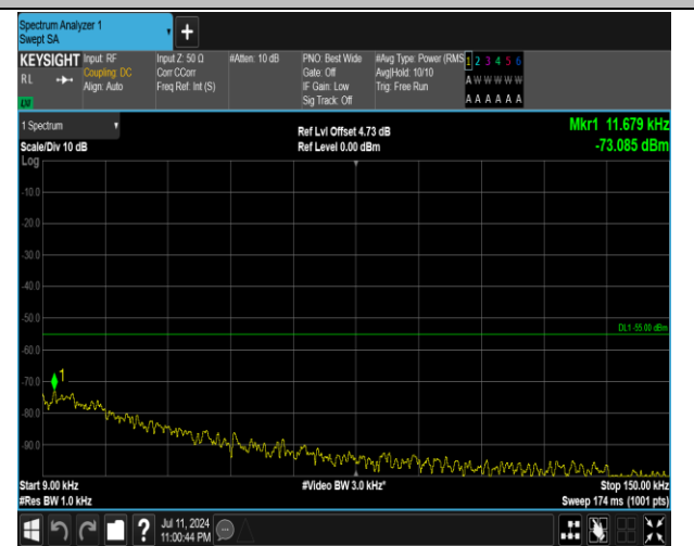
7-7-15MHz-20MHz-16QAM-16QAM-21179-21350-1RB#0- 1RB#99-0.009~0.15MHz-PASS
