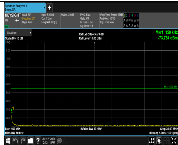
7-7-20MHz-10MHz-16QAM-16QAM-21051-21195-1RB#0-1RB#49-0.15~30MHz-PASS
