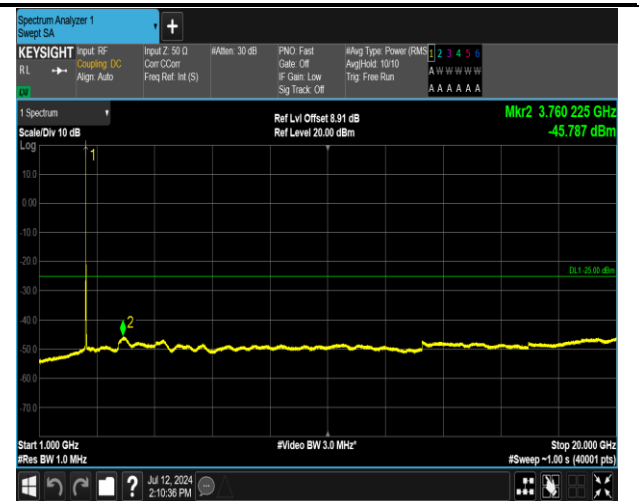
7-7-20MHz-10MHz-16QAM-16QAM-21051-21195-1RB#99 -ORB#0-1000~20000MHz-PASS
