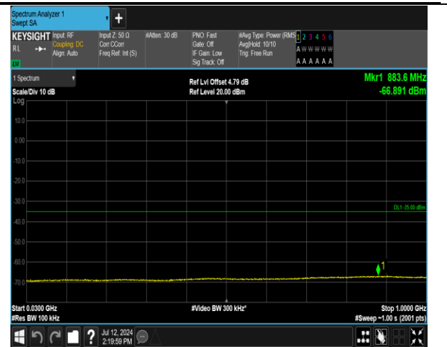
7-7-20MHz-10MHz-16QAM-16QAM-21251-21395-1RB#0- ORB#0-30~1000MHz-PASS
