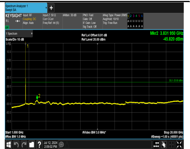
7-7-20MHz-10MHz-QPSK-QPSK-21051-21195-1RB#99-0 RB#0-1000~20000MHz-PASS
