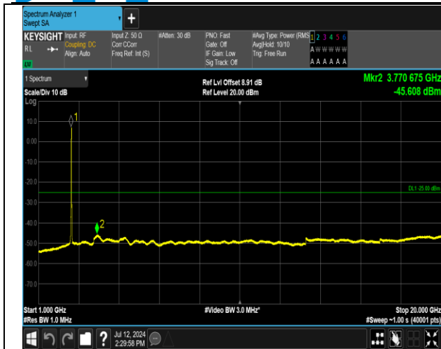
7-7-20MHz-10MHz-16QAM-16QAM-21251-21395-100RB #0-50RB#0-1000~20000MHz-PASS
