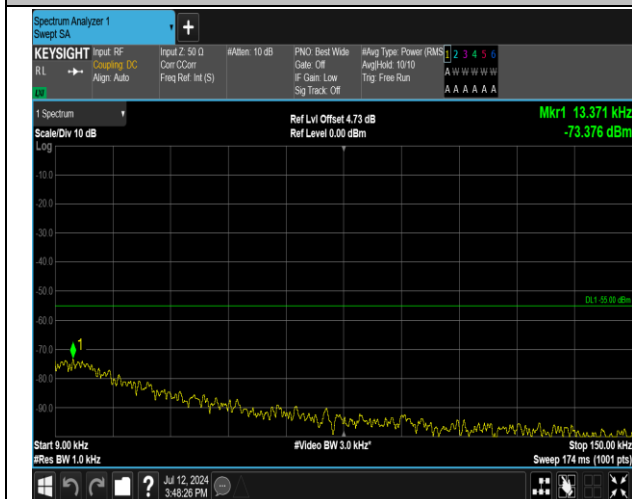
7-7-20MHz-15MHz-QPSK-QPSK-20850-21021-1RB#0-1R B#74-0.009~0.15MHz-PASS
