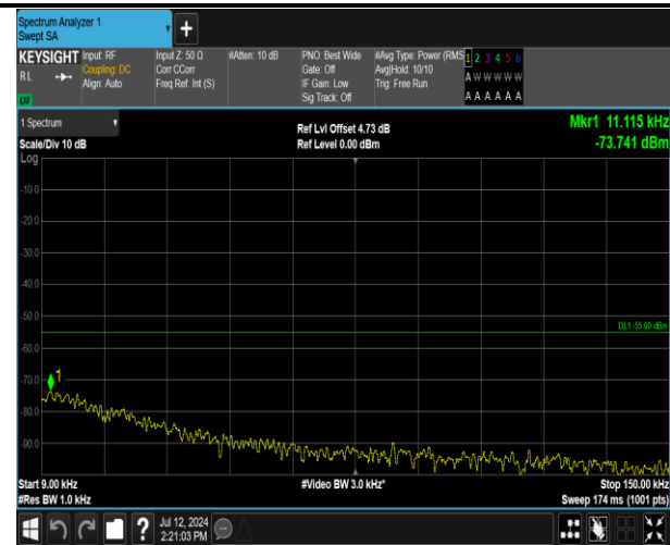
7-7-20MHz-10MHz-QPSK-QPSK-21251-21395-1RB#99-0 RB#0-0.009~0.15MHz-PASS
