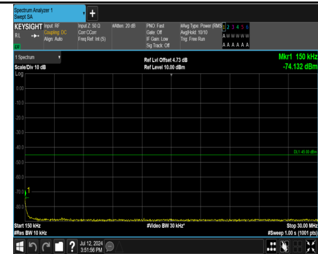
7-7-20MHz-15MHz-QPSK-QPSK-20850-21021-100RB#0-75RB#0-0.15~30MHz-PASS
