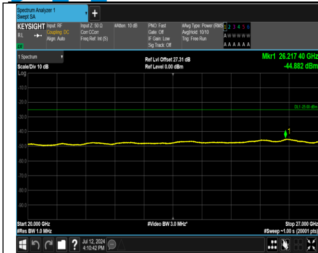
7-7-20MHz-15MHz-16QAM-16QAM-21201-21372-1RB#0- ORB#0-20000~27000MHz-PASS
