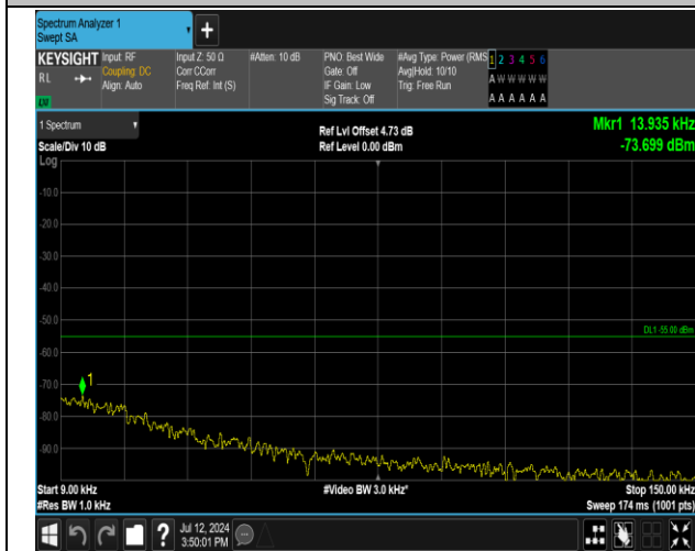
7-7-20MHz-15MHz-16QAM-16QAM-20850-21021-1RB#0- 1RB#74-0.009~0.15MHz-PASS
