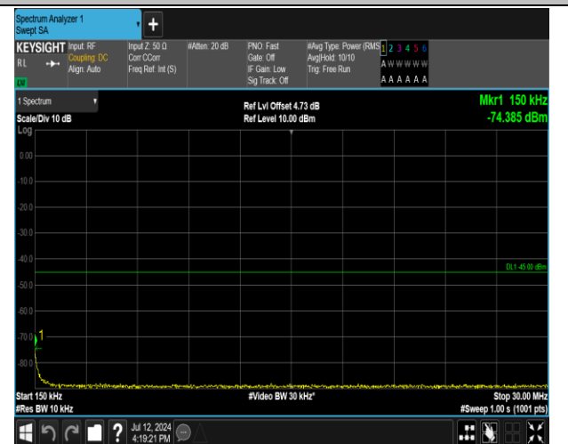
7-7-20MHz-15MHz-16QAM-16QAM-21201-21372-100RB# 0-75RB#0-0.15~30MHz-PASS
