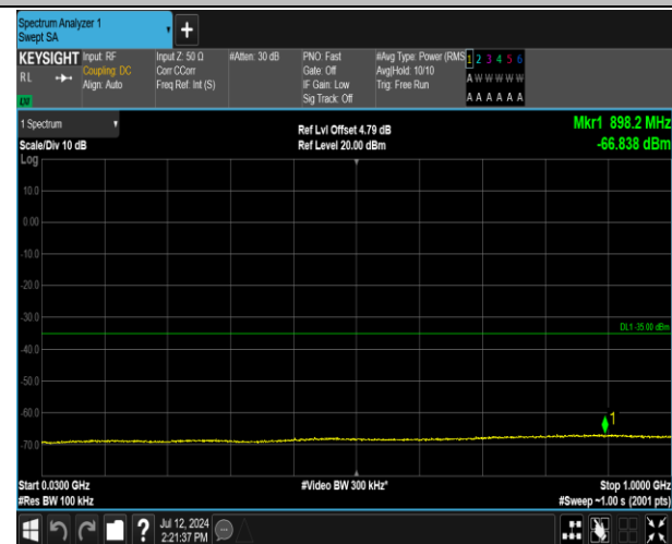
7-7-20MHz-10MHz-QPSK-QPSK-21251-21395-1RB#99-0 RB#0-30~1000MHz-PASS
