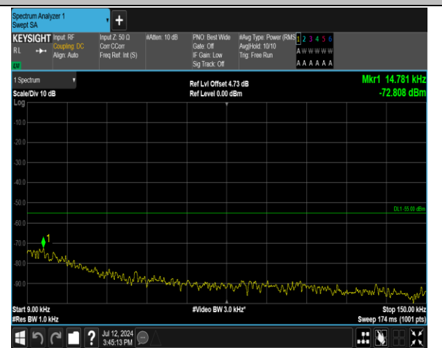
7-7-20MHz-15MHz-QPSK-QPSK-20850-21021-1RB#99-0 RB#0-0.009~0.15MHz-PASS
