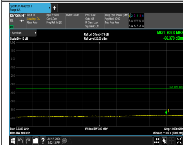
7-7-20MHz-15MHz-QPSK-QPSK-20850-21021-100RB#0-75RB#0-30~1000MHz-PASS
