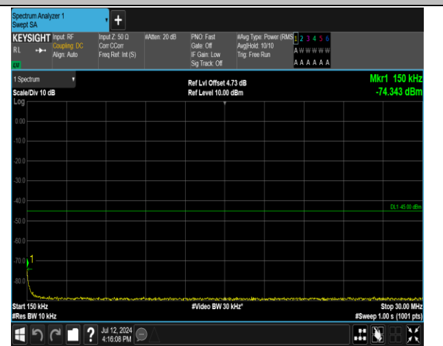
7-7-20MHz-15MHz-16QAM-16QAM-21201-21372-1RB#0- 1RB#74-0.15~30MHz-PASS
