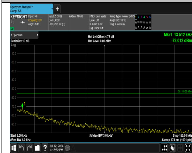
7-7-20MHz-15MHz-16QAM-16QAM-21201-21372-1RB#0- 1RB#74-0.009~0.15MHz-PASS
