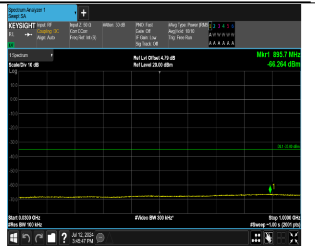
7-7-20MHz-15MHz-QPSK-QPSK-20850-21021-1RB#99-0 RB#0-30~1000MHz-PASS
