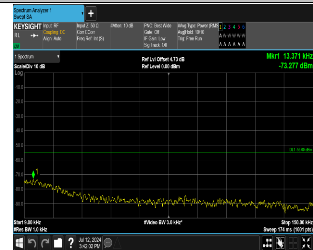
7-7-20MHz-15MHz-QPSK-QPSK-20850-21021-1RB#0-0RB#0-0.009~0.15MHz-PASS
