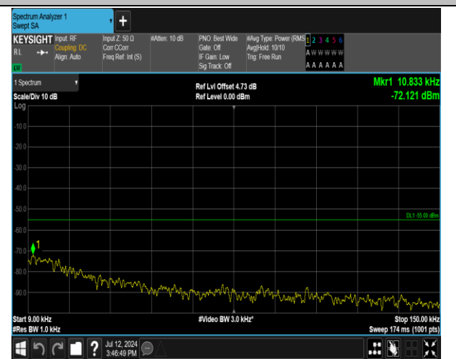
7-7-20MHz-15MHz-16QAM-16QAM-20850-21021-1RB#99-0RB#0-0.009~0.15MHz-PASS
