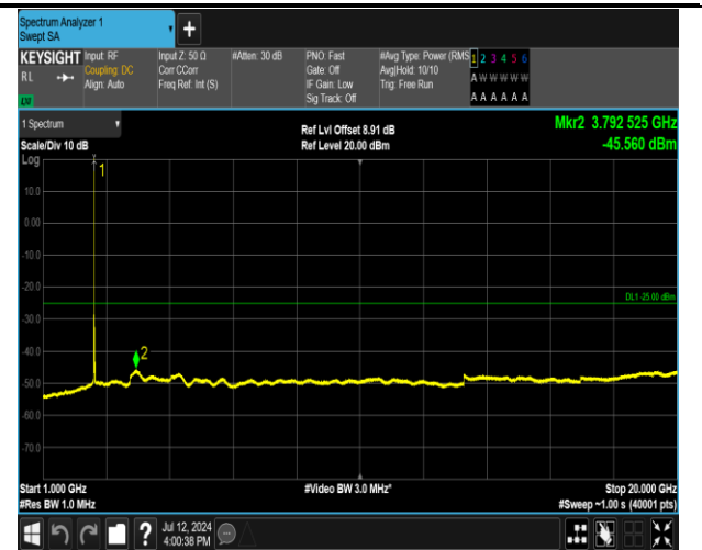
7-7-20MHz-15MHz-16QAM-16QAM-21026-21197-1RB#99 -ORB#0-1000~20000MHz-PASS
