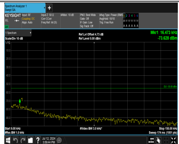
7-7-20MHz-15MHz-16QAM-16QAM-21026-21197-1RB#99 -ORB#0-0.009~0.15MHz-PASS
