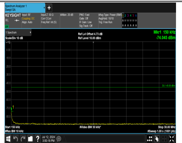
7-7-20MHz-15MHz-16QAM-16QAM-20850-21021-1RB#0- 1RB#74-0.15~30MHz-PASS
