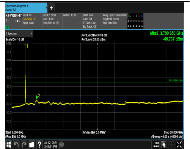
7-7-20MHz-15MHz-16QAM-16QAM-20850-21021-1RB#0- ORB#0-1000~20000MHz-PASS
