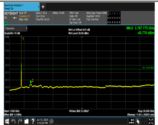
7-7-20MHz-15MHz-16QAM-16QAM-21201-21372-1RB#0- ORB#0-1000~20000MHz-PASS
