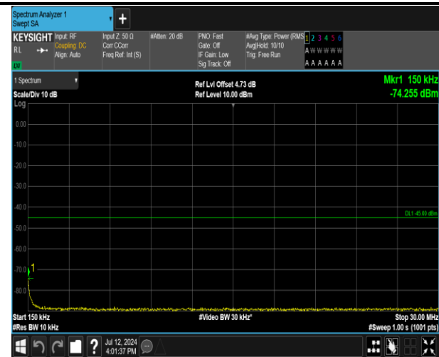
7-7-20MHz-15MHz-QPSK-QPSK-21026-21197-1RB#0-1R B#74-0.15~30MHz-PASS
