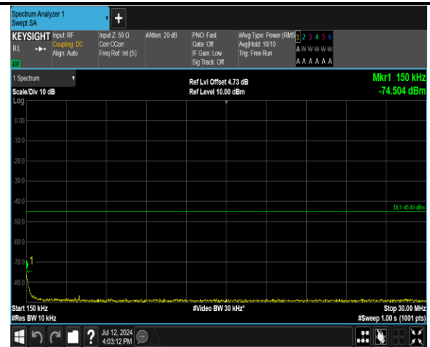
7-7-20MHz-15MHz-16QAM-16QAM-21026-21197-1RB#0- 1RB#74-0.15~30MHz-PASS
