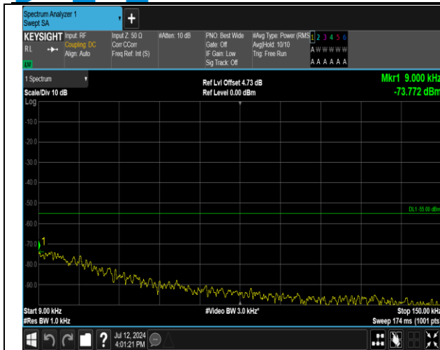
7-7-20MHz-15MHz-QPSK-QPSK-21026-21197-1RB#0-1R B#74-0.009~0.15MHz-PASS
