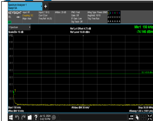
7-7-20MHz-15MHz-QPSK-QPSK-20850-21021-1RB#0-0R B#0-0.15~30MHz-PASS
