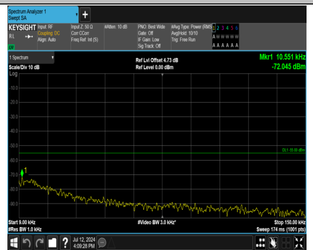
7-7-20MHz-15MHz-16QAM-16QAM-21201-21372-1RB#0- ORB#0-0.009~0.15MHz-PASS
