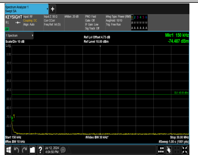
7-7-20MHz-15MHz-QPSK-QPSK-21026-21197-100RB#0-75RB#0-0.15~30MHz-PASS
