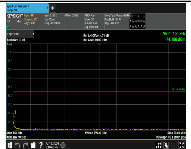
7-7-20MHz-15MHz-QPSK-QPSK-20850-21021-1RB#0-1R B#74-0.15~30MHz-PASS
