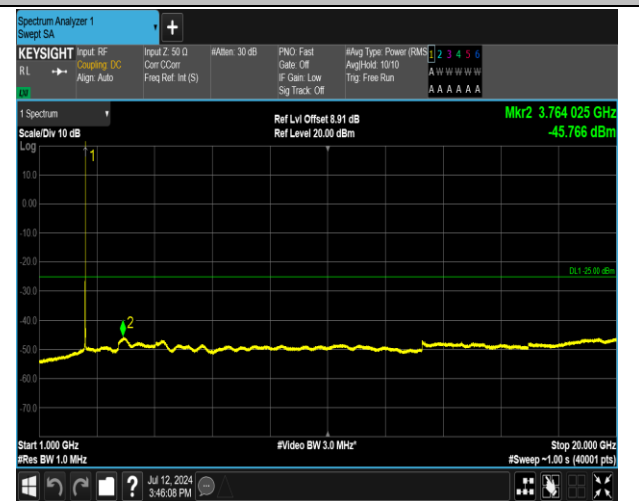
7-7-20MHz-15MHz-QPSK-QPSK-20850-21021-1RB#99-0 RB#0-1000~20000MHz-PASS
