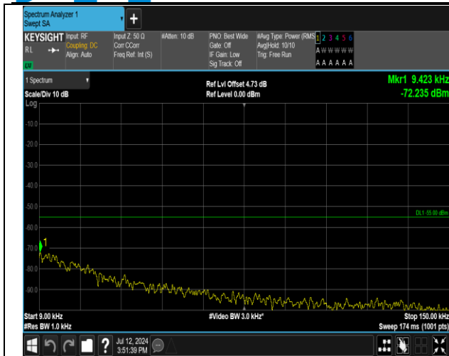
7-7-20MHz-15MHz-QPSK-QPSK-20850-21021-100RB#0-75RB#0-0.009~0.15MHz-PASS
