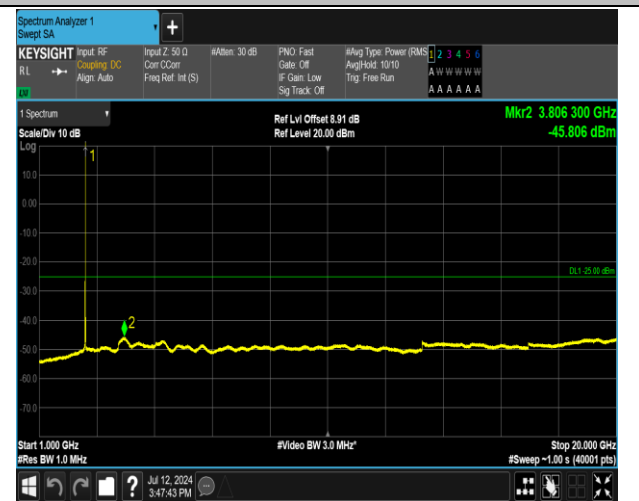
7-7-20MHz-15MHz-16QAM-16QAM-20850-21021-1RB#99-0RB#0-1000~20000MHz-PASS
