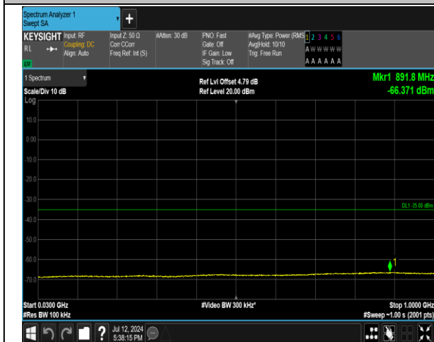
7-7-20MHz-20MHz-QPSK-QPSK-20850-21048-100RB#0-100RB#0-30~1000MHz-PASS
