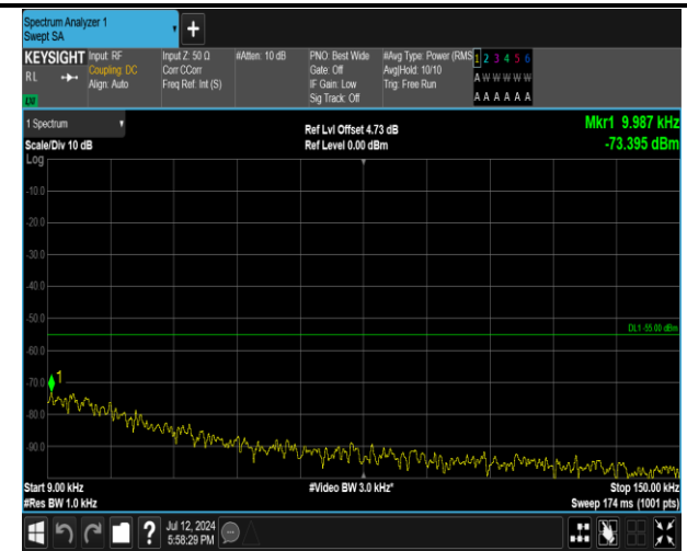
7-7-20MHz-20MHz-16QAM-16QAM-21152-21350-1RB#99-0RB#0-0.009~0.15MHz-PASS
