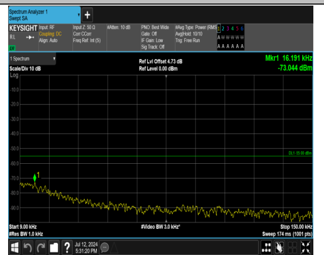
7-7-20MHz-20MHz-QPSK-QPSK-20850-21048-1RB#99-0 RB#0-0.009~0.15MHz-PASS
