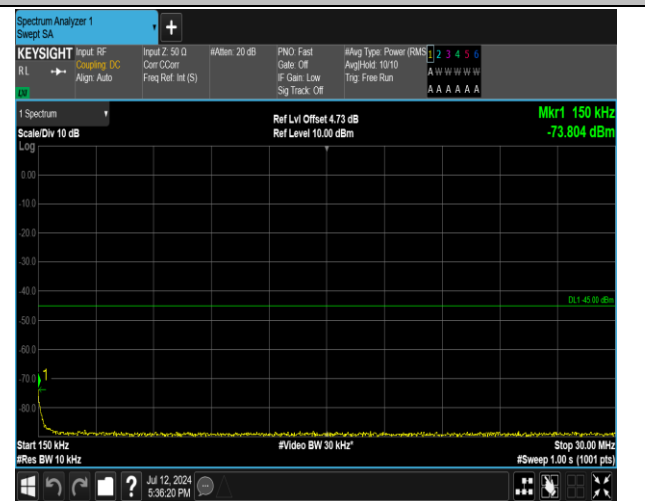
7-7-20MHz-20MHz-16QAM-16QAM-20850-21048-1RB#0- 1RB#99-0.15~30MHz-PASS
