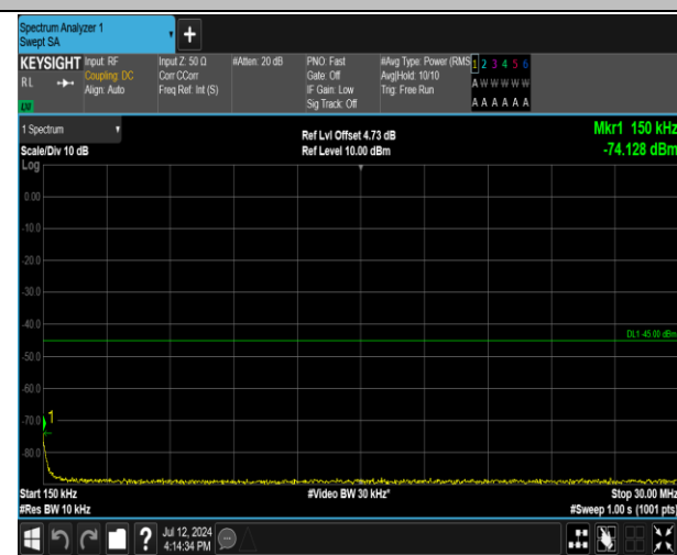
7-7-20MHz-15MHz-QPSK-QPSK-21201-21372-1RB#0-1R B#74-0.15~30MHz-PASS
