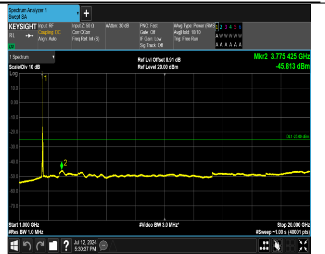
7-7-20MHz-20MHz-16QAM-16QAM-20850-21048-1RB#0- ORB#0-1000~20000MHz-PASS
