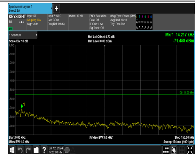
7-7-20MHz-20MHz-QPSK-QPSK-20850-21048-1RB#0-0RB#0-0.009~0.15MHz-PASS
