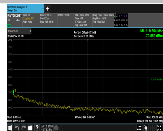
7-7-20MHz-15MHz-QPSK-QPSK-21201-21372-1RB#0-0R B#0-0.009~0.15MHz-PASS
