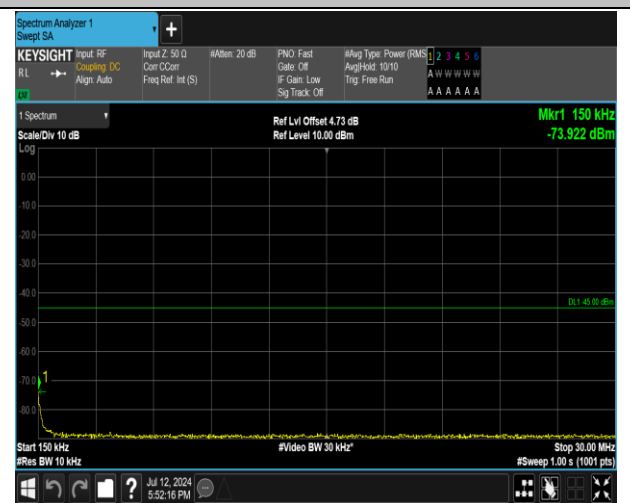
7-7-20MHz-20MHz-16QAM-16QAM-21001-21199-100RB# 0-100RB#0-0.15~30MHz-PASS
