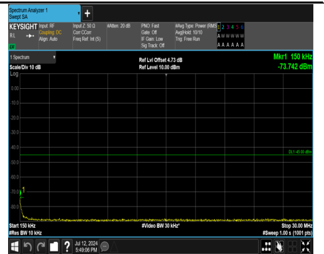
7-7-20MHz-20MHz-16QAM-16QAM-21001-21199-1RB#0- 1RB#99-0.15~30MHz-PASS
