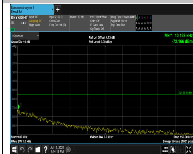
7-7-20MHz-15MHz-QPSK-QPSK-21201-21372-1RB#0-1R B#74-0.009~0.15MHz-PASS
