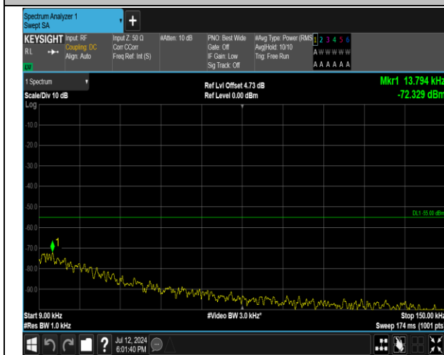
7-7-20MHz-20MHz-16QAM-16QAM-21152-21350-1RB#0- 1RB#99-0.009~0.15MHz-PASS
