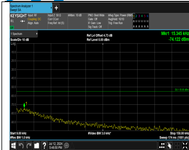
7-7-20MHz-20MHz-16QAM-16QAM-21001-21199-1RB#0- 1RB#99-0.009~0.15MHz-PASS
