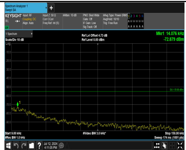
7-7-20MHz-15MHz-QPSK-QPSK-21201-21372-1RB#99-0 RB#0-0.009~0.15MHz-PASS
