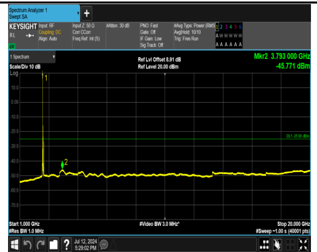
7-7-20MHz-20MHz-QPSK-QPSK-20850-21048-1RB#0-0R B#0-1000~20000MHz-PASS
