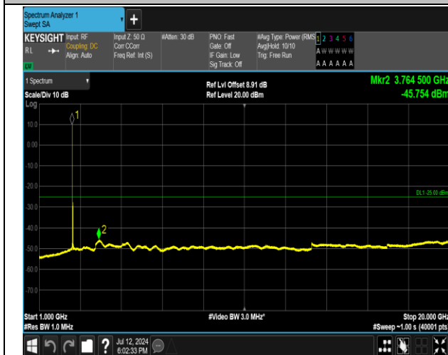
7-7-20MHz-20MHz-16QAM-16QAM-21152-21350-1RB#0- 1RB#99-1000~20000MHz-PASS
