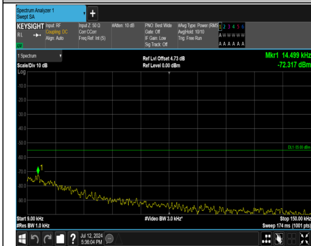
7-7-20MHz-20MHz-16QAM-16QAM-20850-21048-1RB#0- 1RB#99-0.009~0.15MHz-PASS
