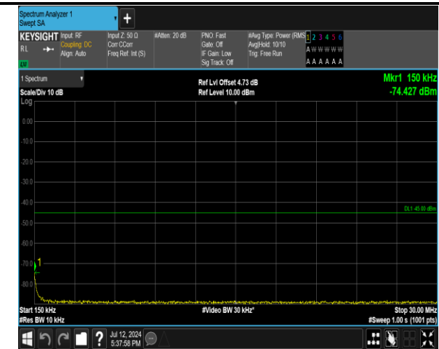
7-7-20MHz-20MHz-QPSK-QPSK-20850-21048-100RB#0-100RB#0-0.15~30MHz-PASS
