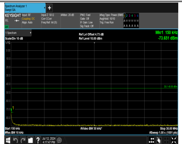
7-7-20MHz-15MHz-QPSK-QPSK-21201-21372-100RB#0-75RB#0-0.15~30MHz-PASS
