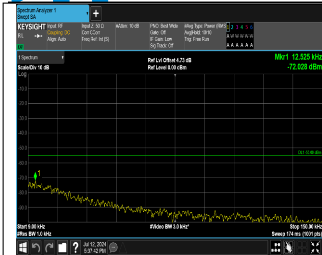
7-7-20MHz-20MHz-QPSK-QPSK-20850-21048-100RB#0-100RB#0-0.009~0.15MHz-PASS
