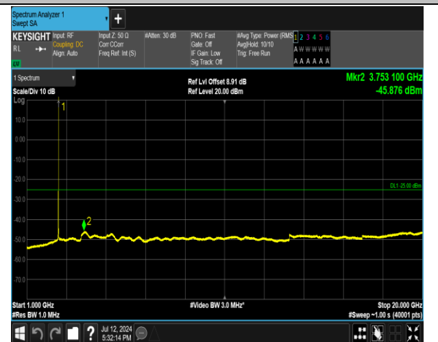
7-7-20MHz-20MHz-QPSK-QPSK-20850-21048-1RB#99-0 RB#0-1000~20000MHz-PASS
