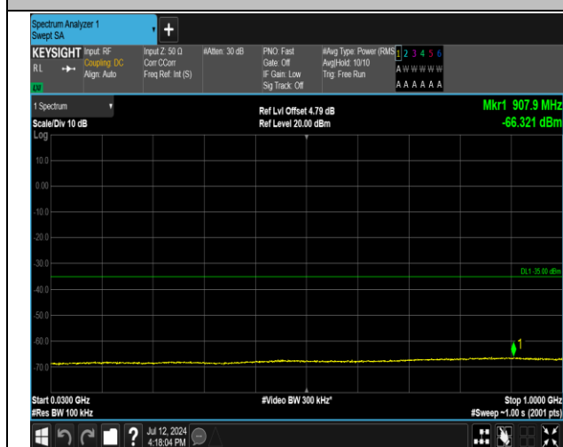
7-7-20MHz-15MHz-QPSK-QPSK-21201-21372-100RB#0-75RB#0-30~1000MHz-PASS
