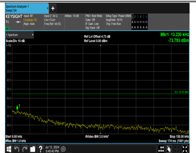
7-7-20MHz-20MHz-16QAM-16QAM-21001-21199-1RB#99 -0RB#0-0.009~0.15MHz-PASS
