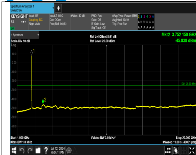
7-7-20MHz-20MHz-QPSK-QPSK-21152-21350-100RB#0-100RB#0-1000~20000MHz-PASS
