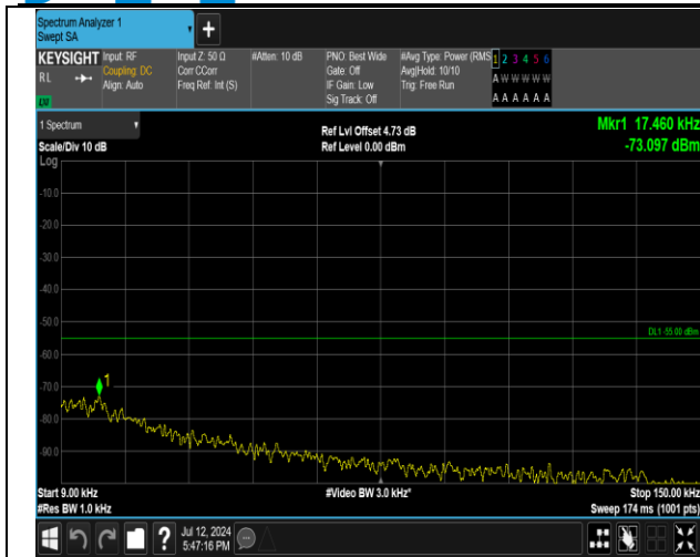
7-7-20MHz-20MHz-QPSK-QPSK-21001-21199-1RB#0-1R B#99-0.009~0.15MHz-PASS
