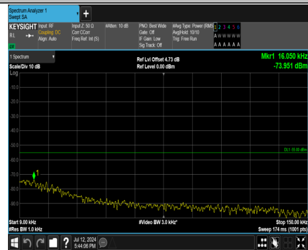
7-7-20MHz-20MHz-QPSK-QPSK-21001-21199-1RB#99-0 RB#0-0.009~0.15MHz-PASS
