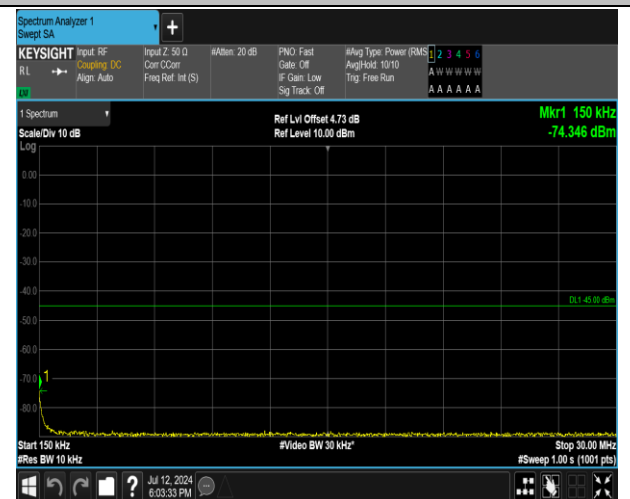
7-7-20MHz-20MHz-QPSK-QPSK-21152-21350-100RB#0-100RB#0-0.15~30MHz-PASS
