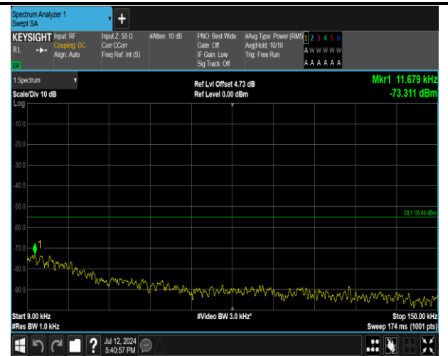
7-7-20MHz-20MHz-QPSK-QPSK-21001-21199-1RB#0-0RB#0-0.009~0.15MHz-PASS
