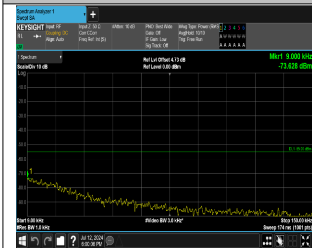
7-7-20MHz-20MHz-QPSK-QPSK-21152-21350-1RB#0-1R B#99-0.009~0.15MHz-PASS
