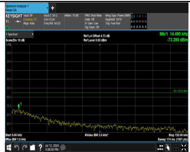
7-7-20MHz-20MHz-QPSK-QPSK-21152-21350-1RB#99-0 RB#0-0.009~0.15MHz-PASS
