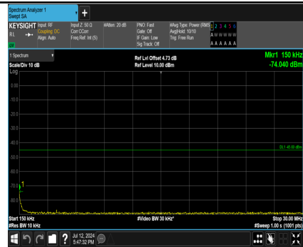
7-7-20MHz-20MHz-QPSK-QPSK-21001-21199-1RB#0-1R B#99-0.15~30MHz-PASS
