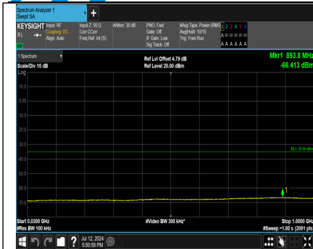
7-7-20MHz-20MHz-QPSK-QPSK-21001-21199-100RB#0-100RB#0-30~1000MHz-PASS
