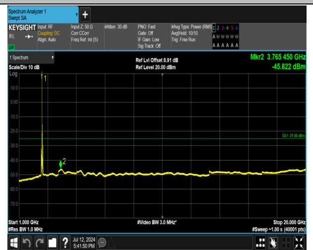
7-7-20MHz-20MHz-QPSK-QPSK-21001-21199-1RB#0-0RB#0-1000~20000MHz-PASS
