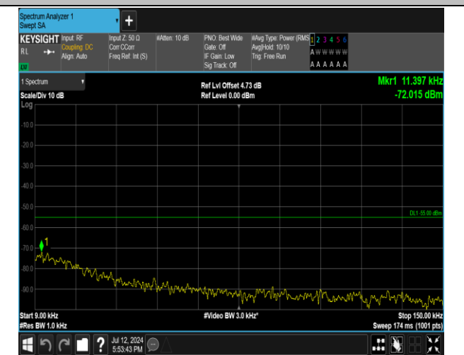
7-7-20MHz-20MHz-QPSK-QPSK-21152-21350-1RB#0-0RB#0-0.009~0.15MHz-PASS
