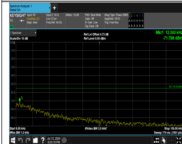
7-7-20MHz-20MHz-QPSK-QPSK-21152-21350-100RB#0-100RB#0-0.009~0.15MHz-PASS
