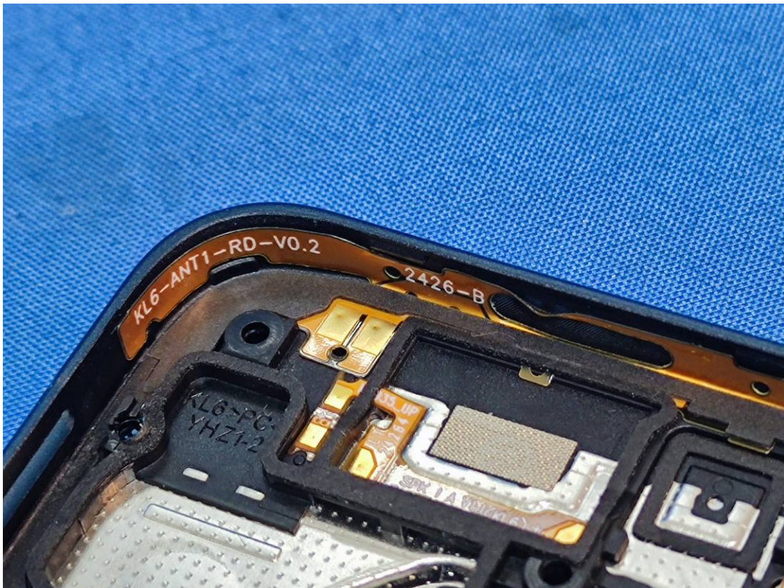
WWAN Antenna(ANT 1)
