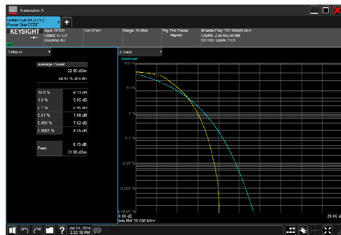
n12_15MHz_15kHz_707.5MHz_DFT-s-OFDM 16 QAM RB75@0 8.75dB
