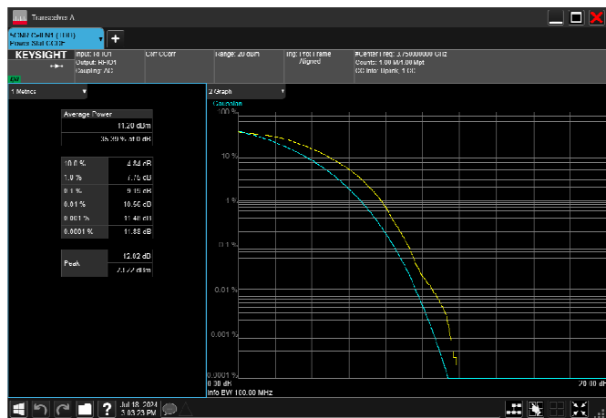
n78_3_100MHz_30kHz_3750MHz_CP-OFDM 16 QAM_RB273@0 10.97dB
