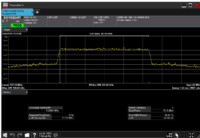
n12_10MHz_15kHz_707.5MHz_CP-OFDM 64 QAM_RB52@0 9.284MHz
