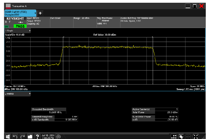
n12_10MHz_15kHz_707.5MHz_CP-OFDM 256 QAM_RB52@0 9.257MHz
