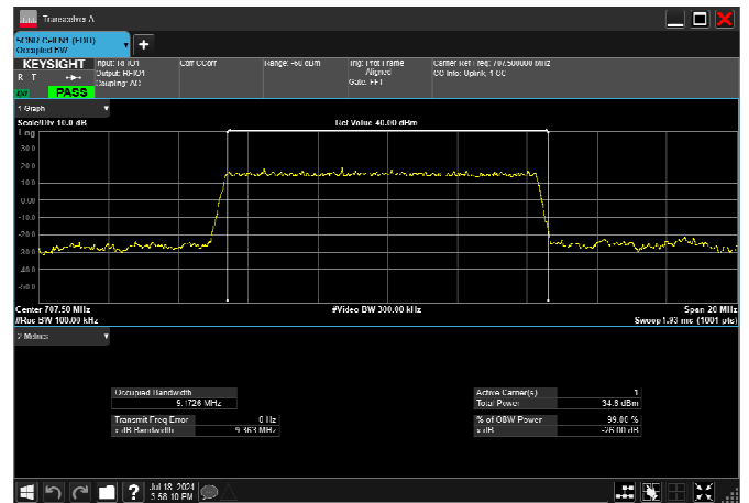
n12_10MHz_15kHz_707.5MHz_DFT-s-OFDM 16 QAM_RB50@0 9.179MHz
