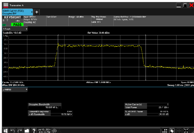
n7_20MHz_15kHz_2535MHz_DFT-s-OFDM QPSK_RB100@0 18.899MHz
