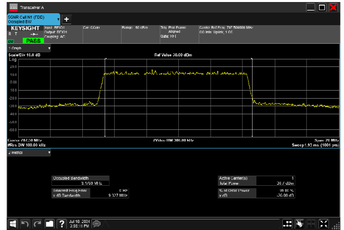
n12_10MHz_15kHz_707.5MHz_CP-OFDM 16 QAM_RB52@0 9.292MHz
