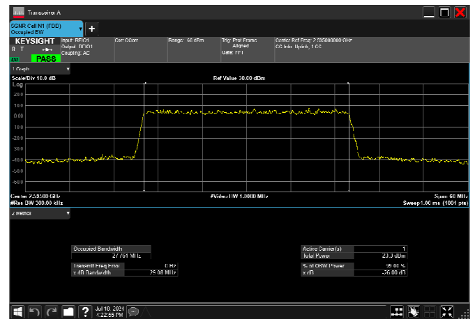
n38_30MHz_30kHz_2595MHz_CP-OFDM 256 QAM_RB78@0 27.761MHz
