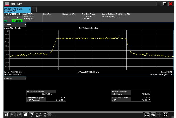
n41_10MHz_30kHz_2592.99MHz_CP-OFDM 16 QAM_RB24@0 8.575MHz
