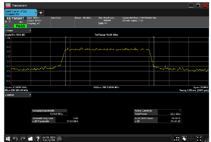
n41_15MHz_30kHz_2592.99MHz_DFT-s-OFDM 64 QAM_RB36@0 13.443MHz
