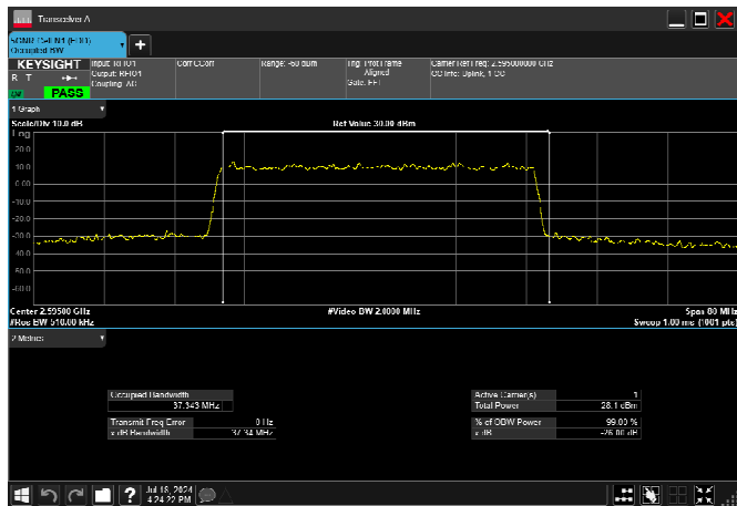
n38_40MHz_30kHz_2595MHz_DFT-s-OFDM 256 QAM_RB100@0 37.283MHz
