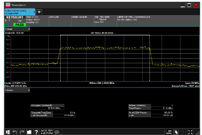
n41_40MHz_30kHz_2592.99MHz_CP-OFDM 256 QAM_RB106@0 37.786MHz
