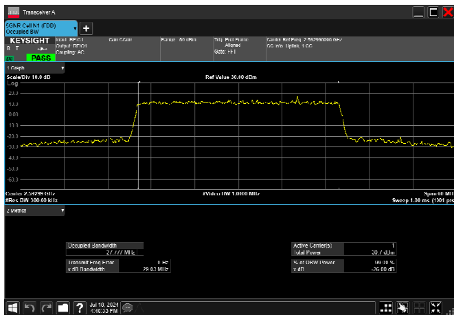
n41_30MHz_30kHz_2592.99MHz_CP-OFDM 256 QAM_RB78@0 27.768MHz
