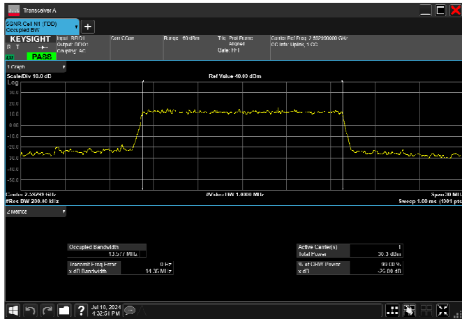
n41_15MHz_30kHz_2592.99MHz_CP-OFDM 256 QAM_RB38@0 13.528MHz
