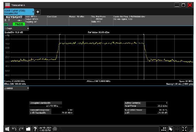
n41_40MHz_30kHz_2592.99MHz_DFT-s-OFDM \pi/2 BPSK_RB100@0 37.647MHz
