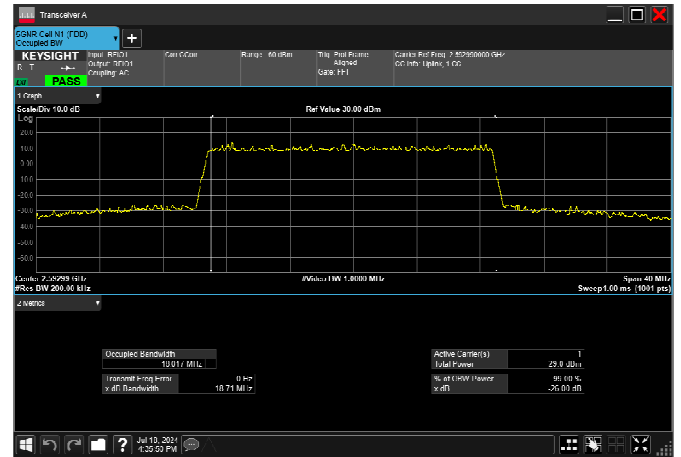
n41_20MHz_30kHz_2592.99MHz_CP-OFDM 16 QAM_RB51@0 18.178MHz
