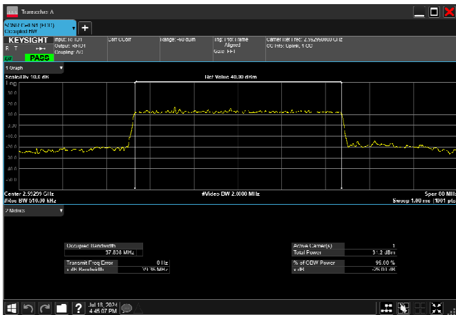
n41_40MHz_30kHz_2592.99MHz_CP-OFDM 64 QAM_RB106@0 37.817MHz
