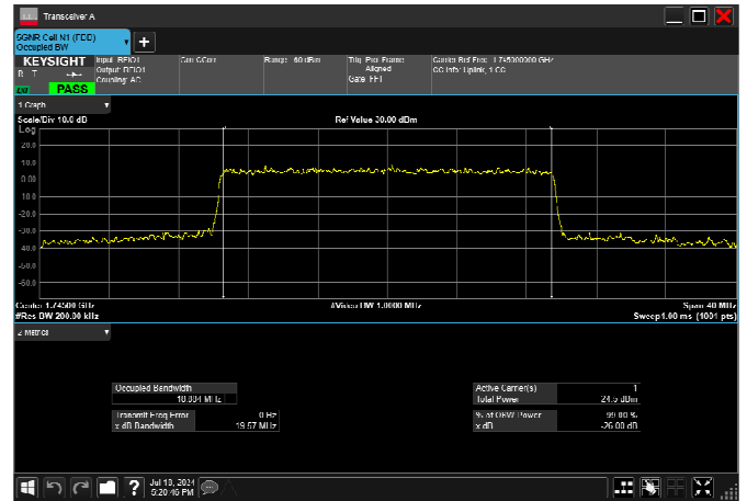
n66_25MHz_15kHz_1745MHz_DFT-s-OFDM \pi/2 BPSK_RB128@0 23.545MHz
