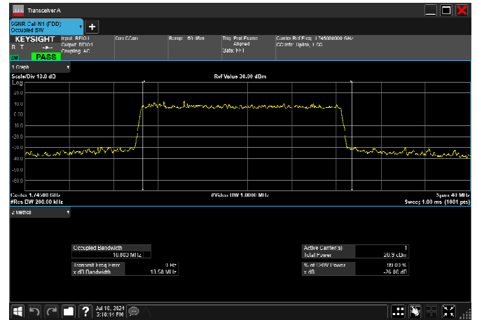
n66_20MHz_15kHz_1745MHz_DFT-s-OFDM 64 QAM_RB100@0 18.663MHz
