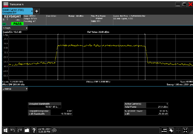
n66_20MHz_15kHz_1745MHz_CP-OFDM 256 QAM_RB106@0 18.898MHz
