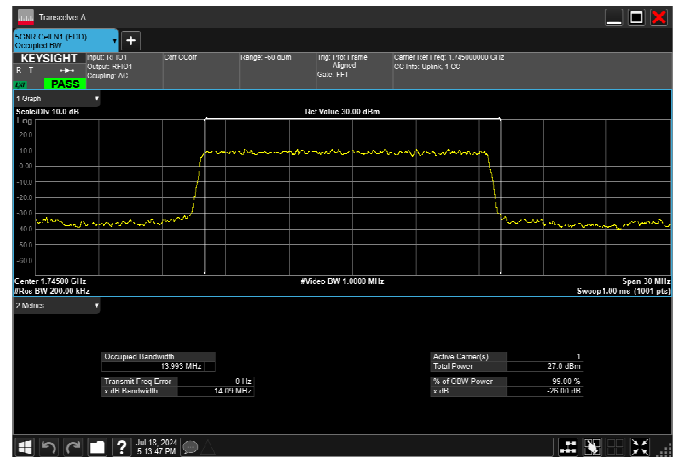
n66_15MHz_15kHz_1745MHz_DFT-s-OFDM 16 QAM_RB75@0 14.047MHz
