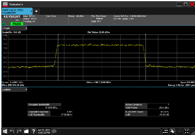
n77_1_50MHz_30kHz_3500MHz_CP-OFDM QPSK_RB133@0 47.439MHz
