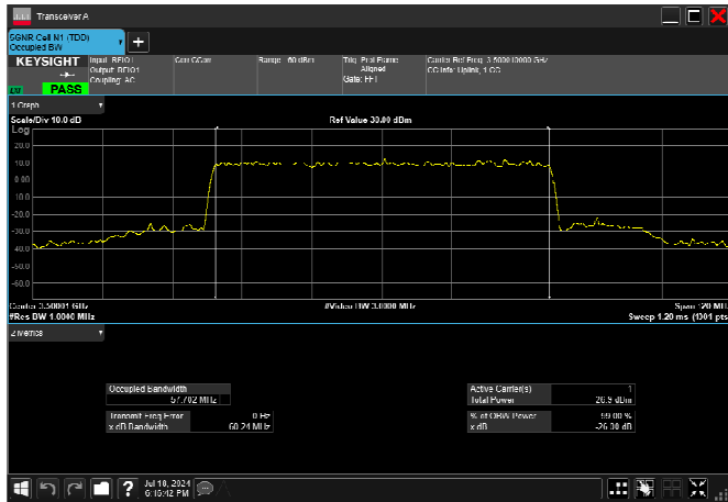
n77_1_60MHz_30kHz_3500MHz_CP-OFDM 256 QAM_RB162@0 57.714MHz
