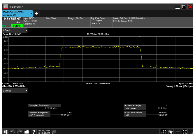
n77_1_70MHz_30kHz_3500MHz_CP-OFDM 64 QAM_RB189@0 67.240MHz
