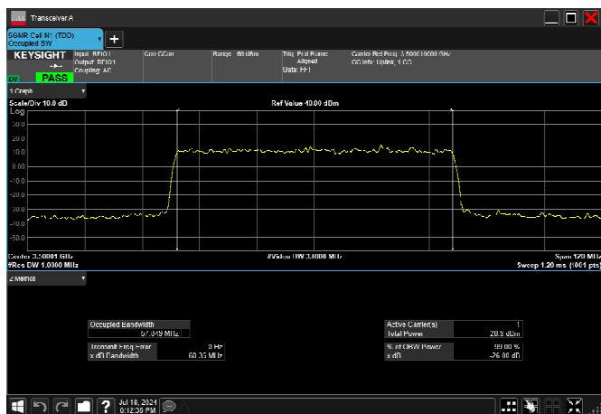
n77_1_60MHz_30kHz_3500MHz_DFT-s-OFDM 16 QAM_RB162@0 57.632MHz
