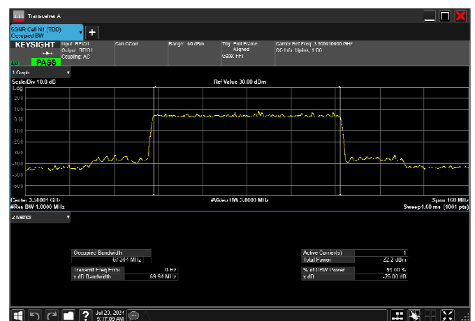
n77_1_70MHz_30kHz_3500MHz_CP-OFDM 256 QAM_RB189@0 67.304MHz
