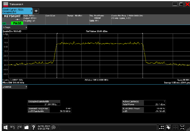
n77_1_40MHz_30kHz_3500MHz_CP-OFDM 256 QAM_RB106@0 37.766MHz
