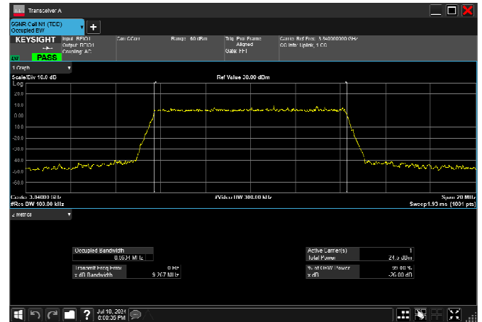
n77_3_10MHz_30kHz_3840MHz_CP-OFDM 16 QAM_RB24@0 8.571MHz
