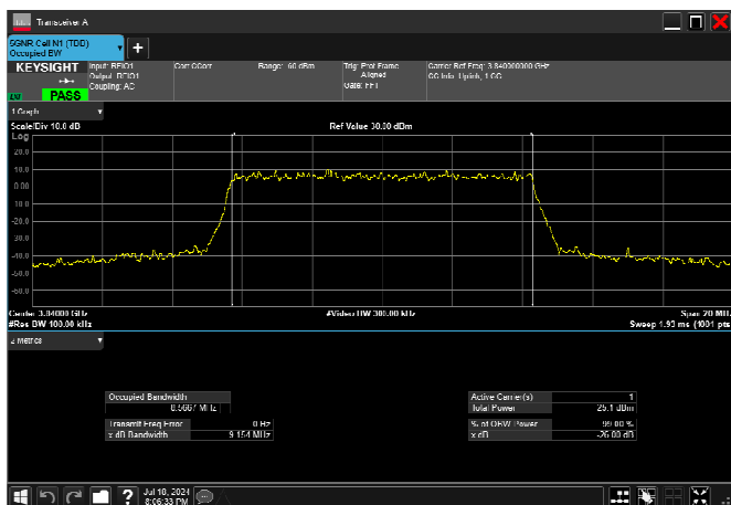
n77_3_10MHz_30kHz_3840MHz_CP-OFDM 64 QAM_RB24@0 8.567MHz
