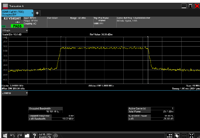
n77_3_20MHz_30kHz_3840MHz_CP-OFDM 64 QAM_RB51@0 18.181MHz
