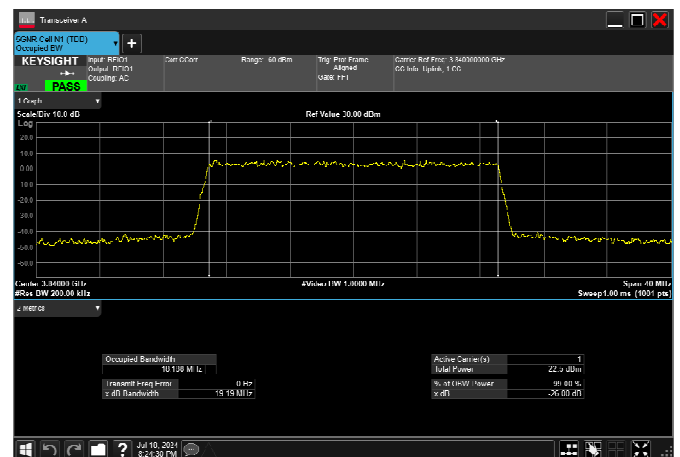
n77_3_20MHz_30kHz_3840MHz_CP-OFDM 256 QAM_RB51@0 18.188MHz
