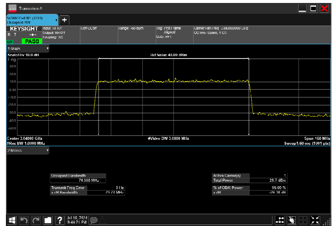
n77_3_80MHz_30kHz_3840MHz_DFT-s-OFDM 16 QAM_RB216@0 76.875MHz
