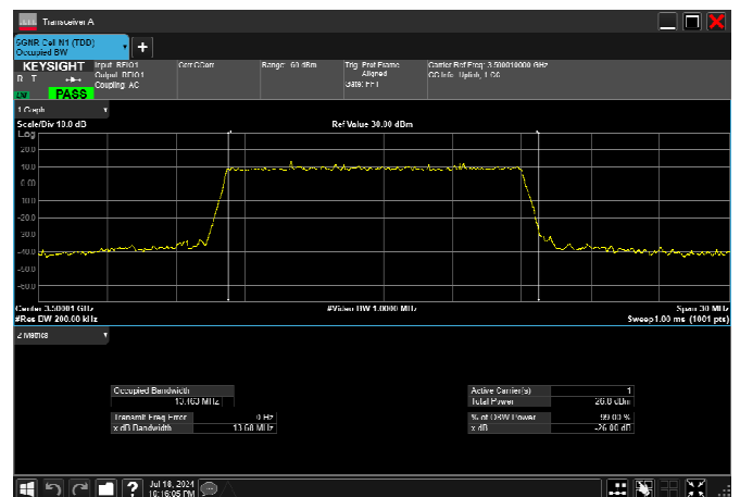
n78_1_15MHz_30kHz_3500MHz_DFT-s-OFDM 16 QAM_RB36@0 13.463MHz
