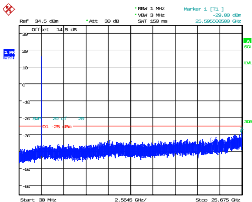
5MHz_High_QPSK_1@0 -29.00dBm
