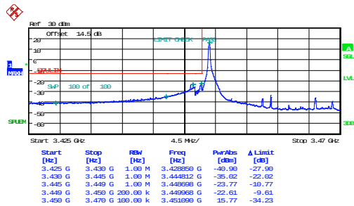
1_20MHz_Low_QPSK_1@0
