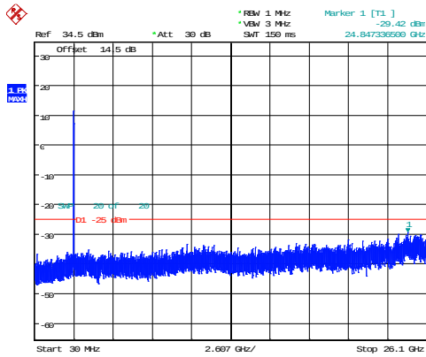
20MHz_High_QPSK_100@0 -29.42dBm
