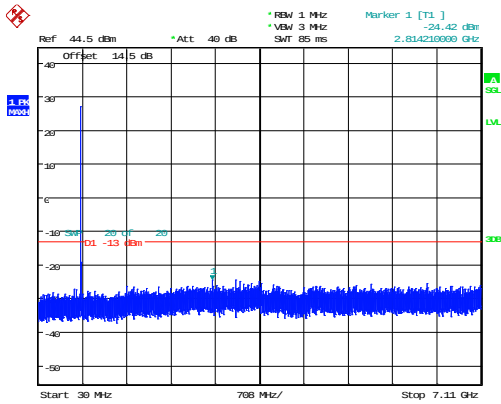
10MHz_High_QPSK_1@0 -24.42dBm
