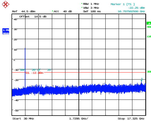
20MHz_Middle_QPSK_100@0 -22.25dBm
