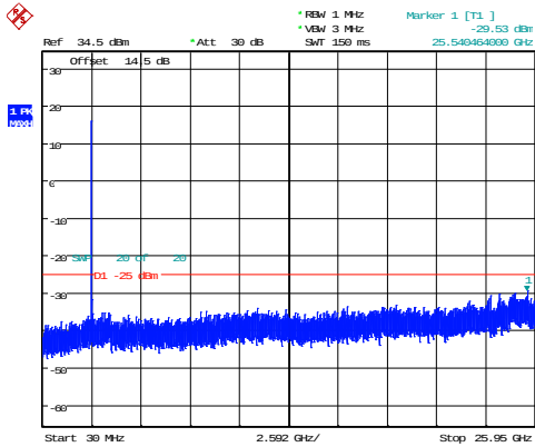
20MHz_Middle_QPSK_1@0 -29.53dBm
