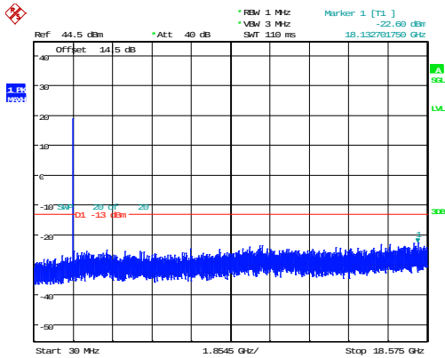
15MHz_Low_QPSK_1@0 -22.60dBm
