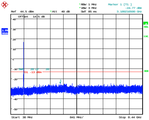
10MHz_High_QPSK_50@0 -24.77dBm
