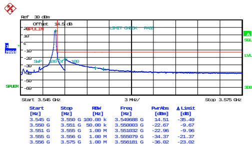
1_5MHz_High_16QAM_1@24
