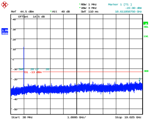
15MHz_High_QPSK_75@0 -22.90dBm
