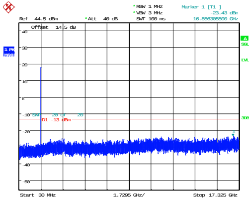
5MHz_Middle_QPSK_1@0 -23.43dBm
