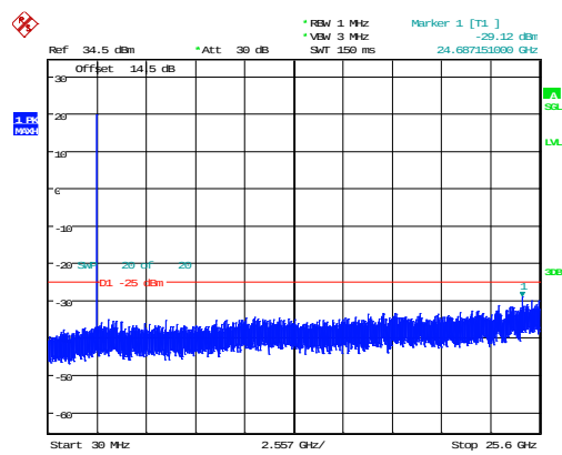
20MHz_High_QPSK_1@0 -29.12dBm
