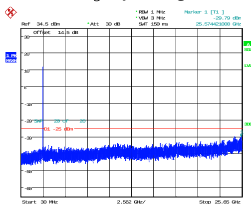
10MHz_High_QPSK_50@0 -29.79dBm
