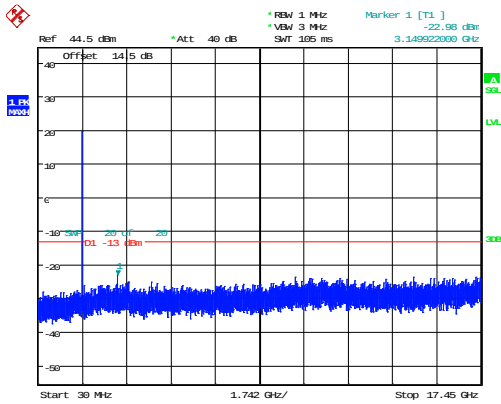
20MHz_High_QPSK_1@0 -22.98dBm
