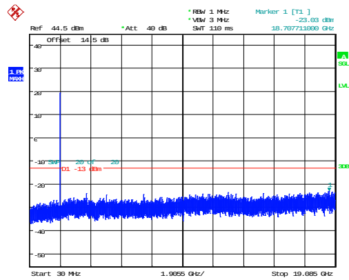
3MHz_High_QPSK_1@0 -23.03dBm
