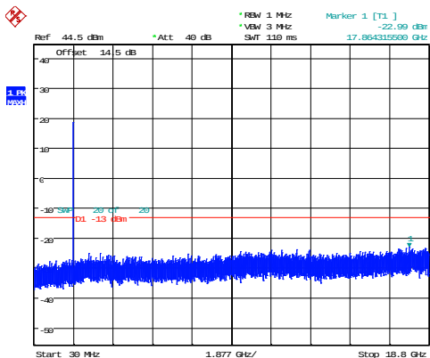
1.4MHz_Middle_QPSK_6@0 -22.99dBm
