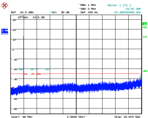
5MHz_High_QPSK_25@0 -29.81dBm
