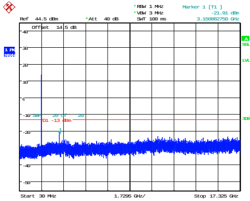
5MHz_Middle_QPSK_25@0 -21.91dBm
