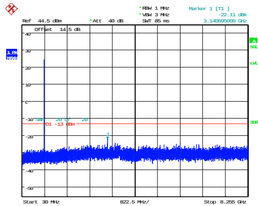
3MHz_Low_QPSK_1@0 -22.11dBm
