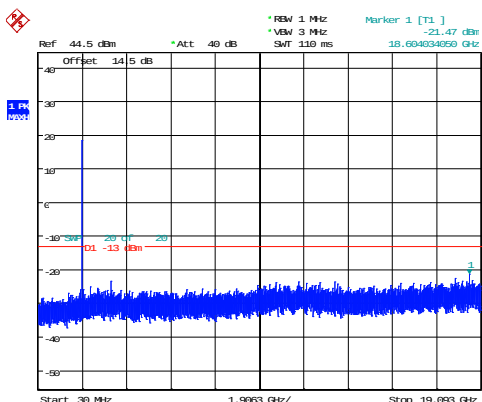
1.4MHz_High_QPSK_6@0 -21.47dBm
