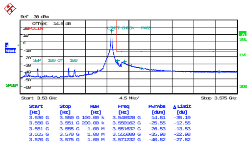
1_20MHz_High_QPSK_1@99
