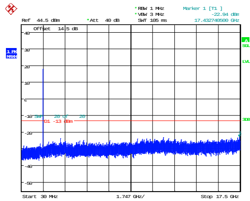
10MHz_High_QPSK_1@0 -22.94dBm
