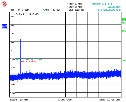
10MHz_High_QPSK_50@0 -22.23dBm
