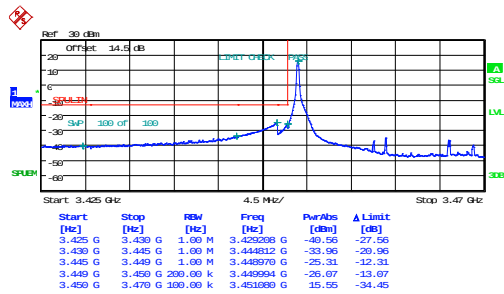
1_20MHz_Low_16QAM_1@0
