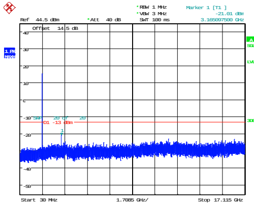
3MHz_Low_QPSK_15@0 -21.01dBm
