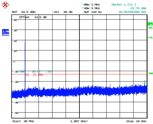
20MHz_High_QPSK_1@0 -22.75dBm
