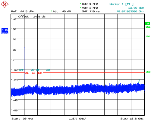
15MHz_Middle_QPSK_75@0 -23.60dBm
