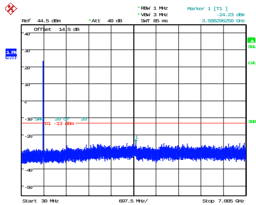
3MHz_Low_QPSK_15@0 -24.23dBm
