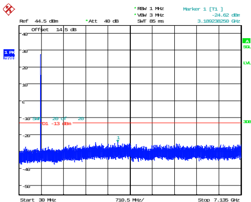
5MHz_High_QPSK_1@0 -24.62dBm
