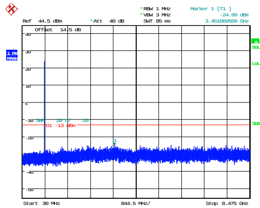
3MHz_High_QPSK_1@0 -24.99dBm
