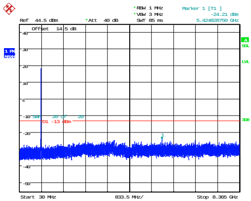
5MHz_Middle_QPSK_25@0 -24.21dBm
