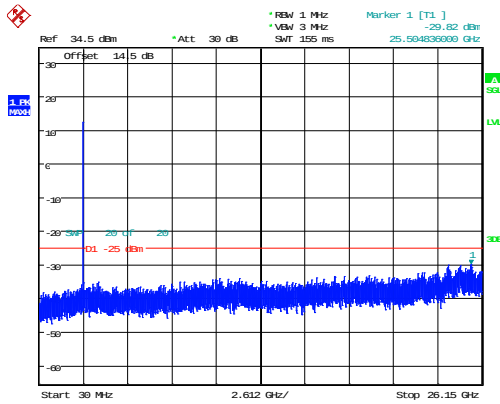
10MHz_High_QPSK_50@0 -29.82dBm
