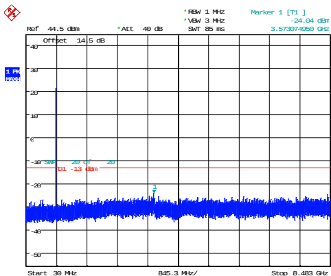
1.4MHz_High_QPSK_6@0 -24.04dBm
