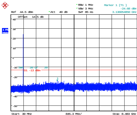
1.4MHz_High_QPSK_1@0 -24.68dBm
