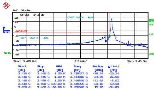
1_10MHz_Low_16QAM_1@0
