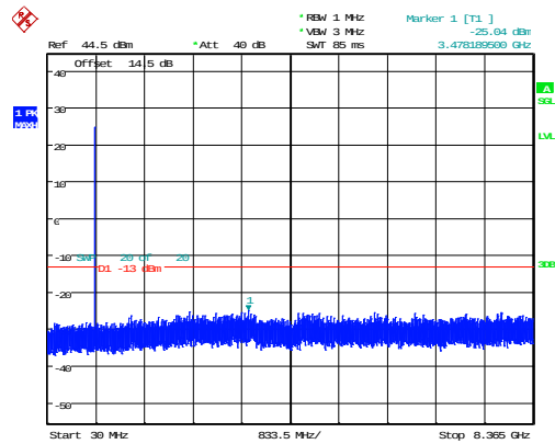
5MHz_Middle_QPSK_1@0 -25.04dBm
