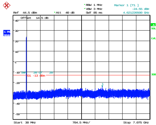
3MHz_Middle_QPSK_15@0 -24.55dBm
