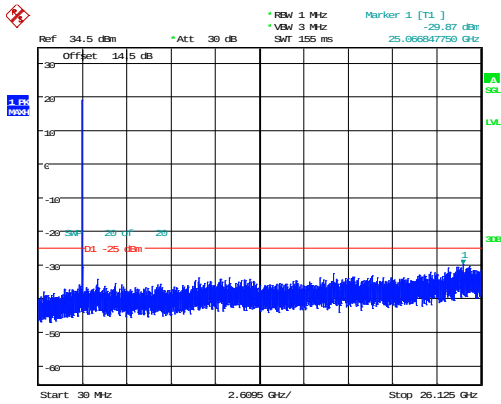
15MHz_High_QPSK_1@0 -29.87dBm
