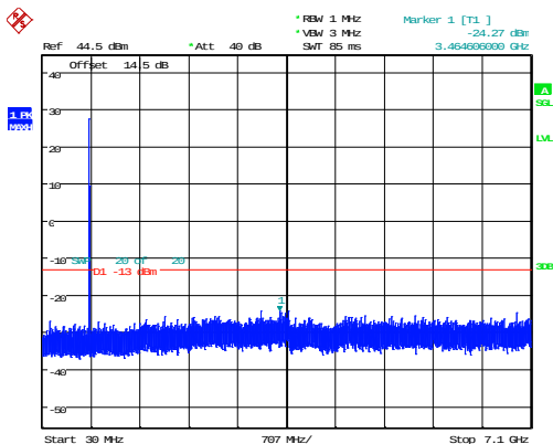
5MHz_Middle_QPSK_1@0 -24.27dBm
