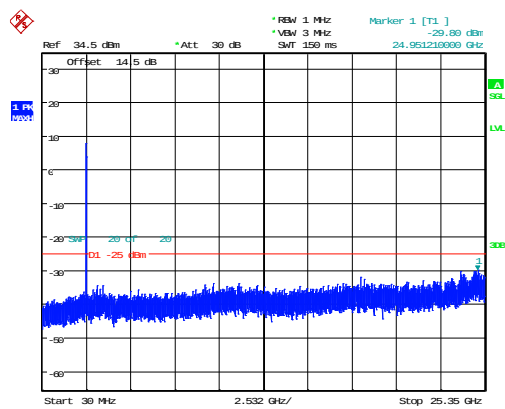
20MHz_Middle_QPSK_100@0 -29.80dBm
