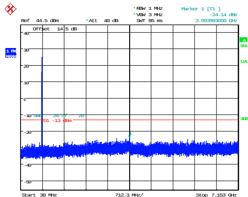
1.4MHz_High_QPSK_6@0 -24.14dBm
