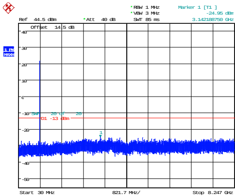
1.4MHz_Low_QPSK_6@0 -24.95dBm
