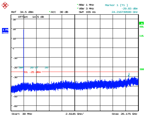
5MHz_High_QPSK_1@0 -29.83dBm
