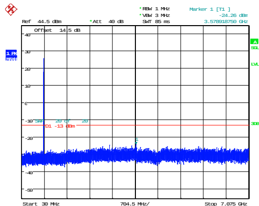
1.4MHz_Middle_QPSK_6@0 -24.26dBm
