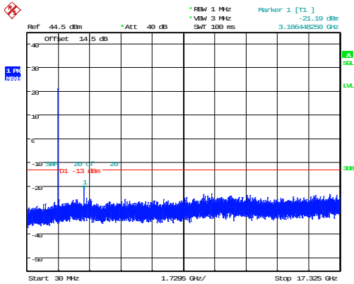
3MHz_Middle_QPSK_1@0 -21.19dBm
