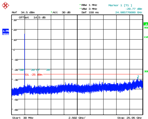
5MHz_Middle_QPSK_25@0 -29.77dBm
