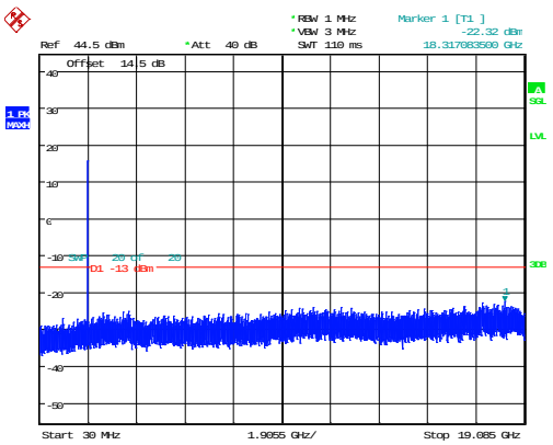
3MHz_High_QPSK_15@0 -22.32dBm
