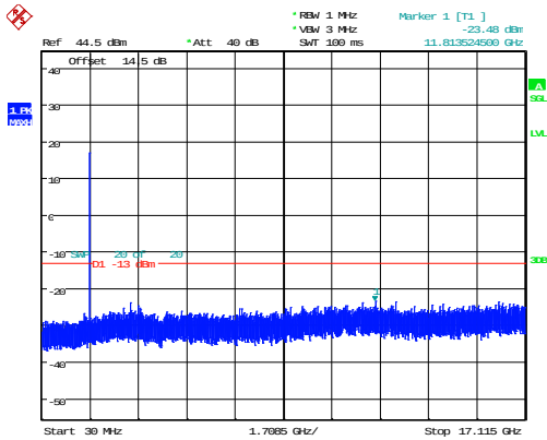
3MHz_Low_QPSK_1@0 -23.48dBm
