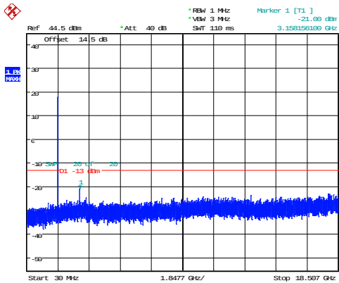
1.4MHz_Low_QPSK_6@0 -21.00dBm
