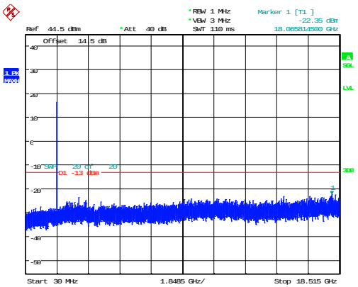
3MHz_Low_QPSK_15@0 -22.35dBm
