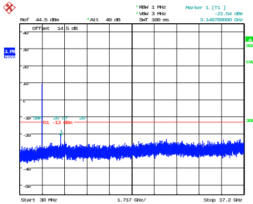
20MHz_Low_QPSK_100@0 -21.54dBm
