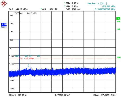
15MHz_Middle_QPSK_75@0 -23.85dBm
