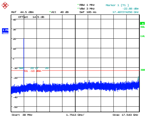
1.4MHz_High_QPSK_1@0 -22.88dBm
