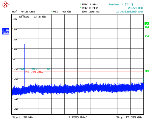
3MHz_High_QPSK_15@0 -23.50dBm
