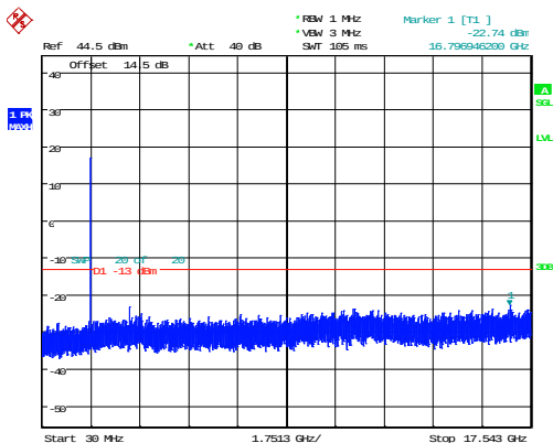
1.4MHz_High_QPSK_6@0 -22.74dBm
