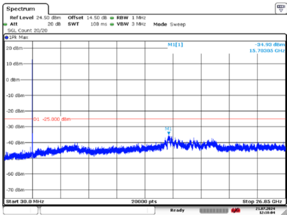
10MHz_High_QPSK_50@0 -34.93dBm
