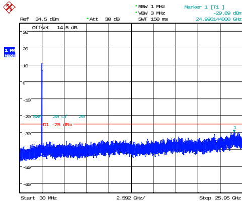
20MHz_Middle_QPSK_100@0 -29.89dBm
