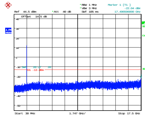
10MHz_High_QPSK_50@0 -22.04dBm
