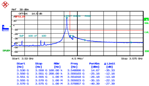
1_20MHz_High_16QAM_1@99
