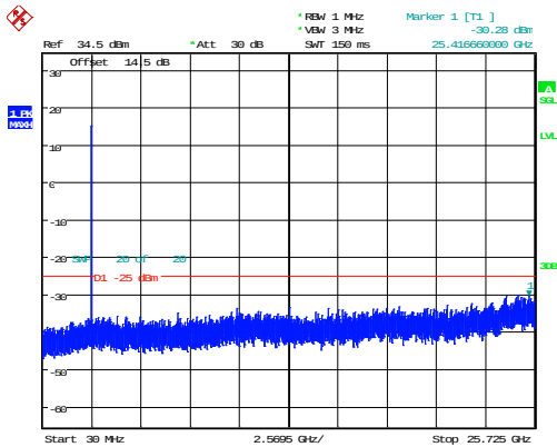
5MHz_Low_QPSK_1@0 -30.28dBm
