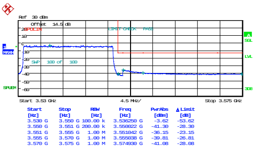
1_20MHz_High_QPSK_100@0
