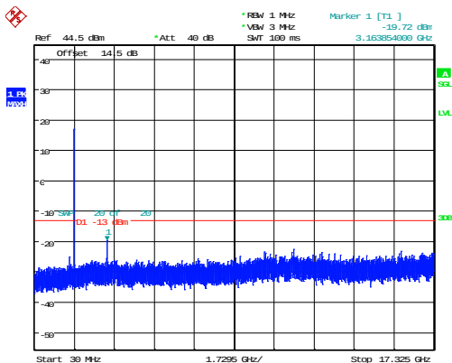
1.4MHz_Middle_QPSK_6@0 -19.72dBm
