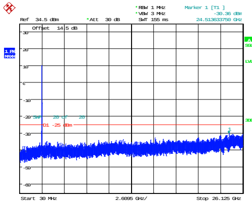
15MHz_High_QPSK_75@0 -30.36dBm
