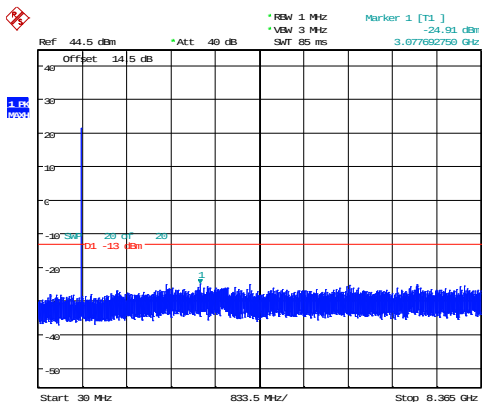
1.4MHz_Middle_QPSK_6@0 -24.91dBm
