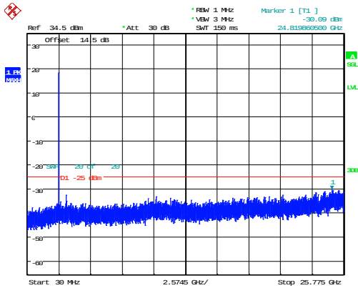
15MHz_Low_QPSK_1@0 -30.09dBm
