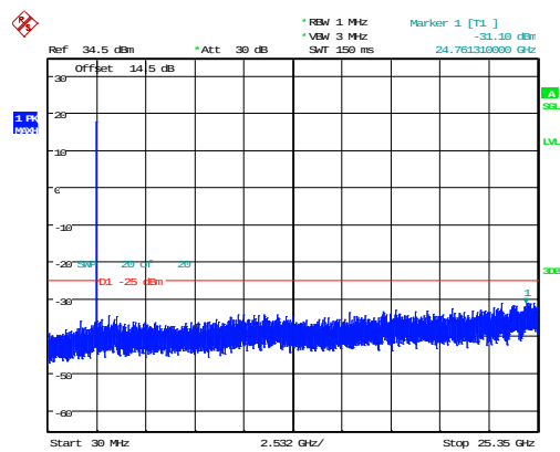
20MHz_Middle_QPSK_1@0 -31.10dBm
