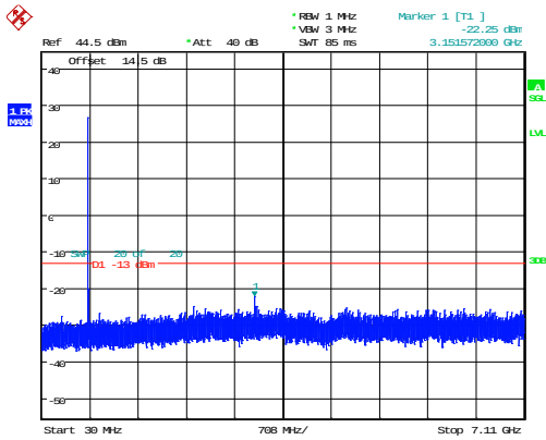
10MHz_High_QPSK_1@0 -22.25dBm
