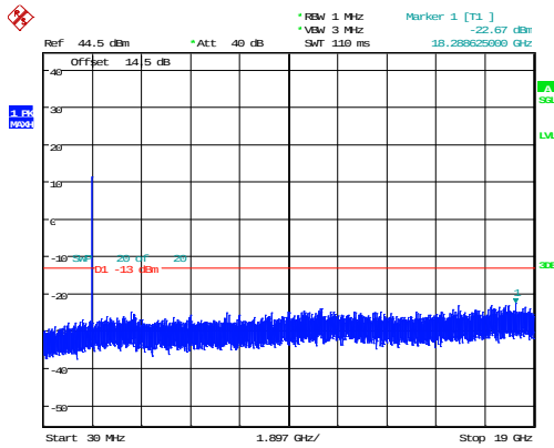
20MHz_High_QPSK_100@0 -22.67dBm
