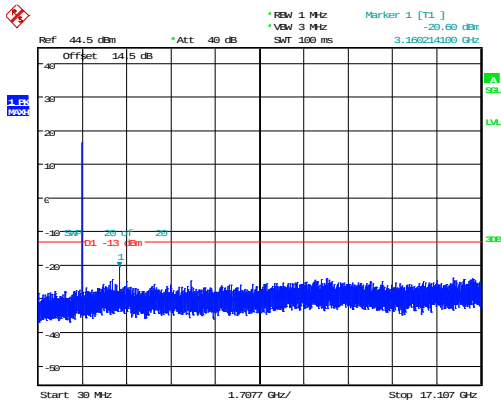
1.4MHz_Low_QPSK_6@0 -20.60dBm
