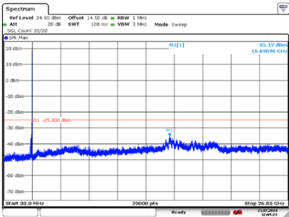
10MHz_High_QPSK_1@0 -35.12dBm
