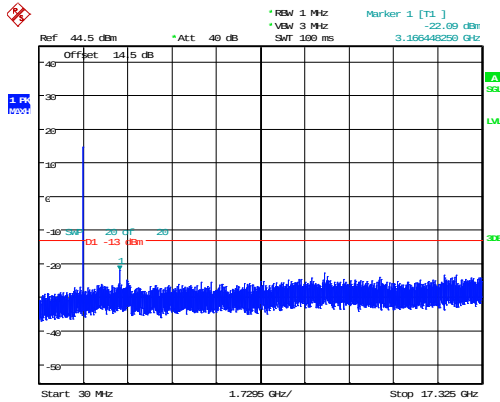
3MHz_Middle_QPSK_15@0 -22.09dBm
