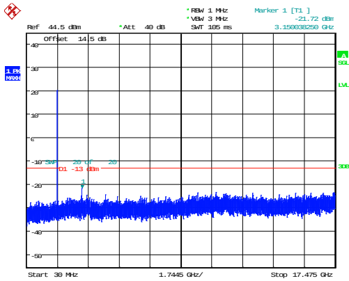
15MHz_High_QPSK_1@0 -21.72dBm
