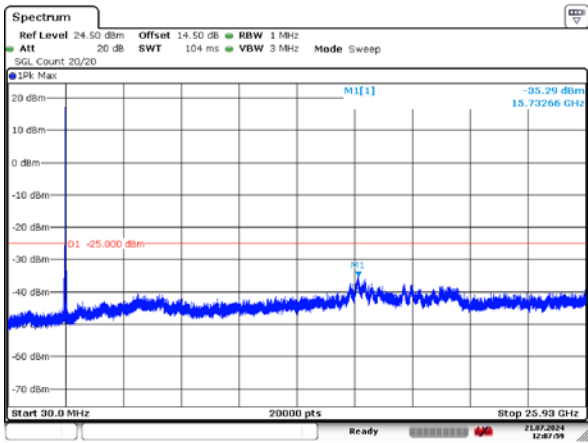
10MHz_Middle_QPSK_1@0 -35.29dBm
