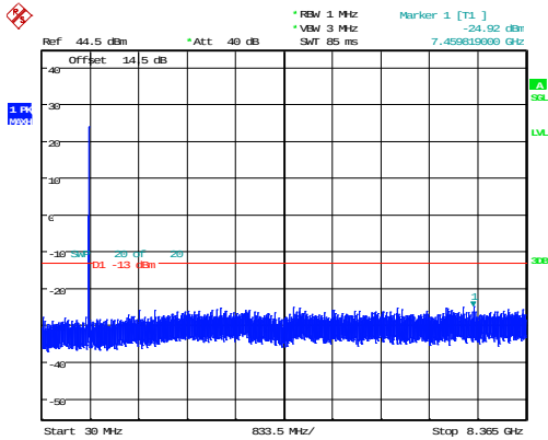
10MHz_Middle_QPSK_1@0 -24.92dBm
