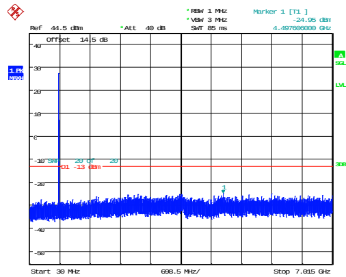
5MHz_Low_QPSK_1@0 -24.95dBm
