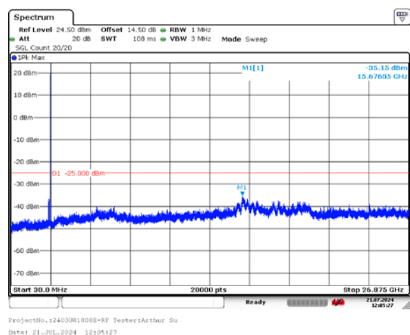
5MHz_High_QPSK_1@0 -35.15dBm
