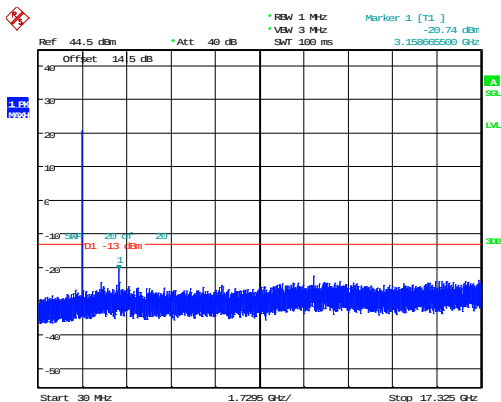
1.4MHz_Middle_QPSK_1@0 -20.74dBm
