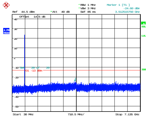
5MHz_High_QPSK_25@0 -24.60dBm
