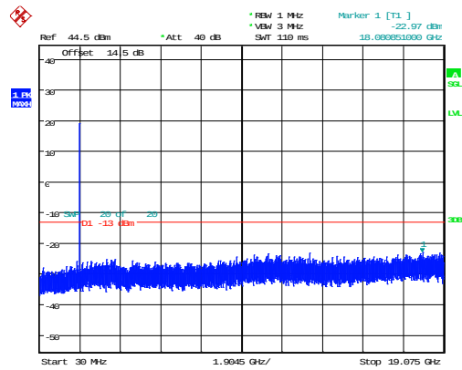
5MHz_High_QPSK_1@0 -22.97dBm
