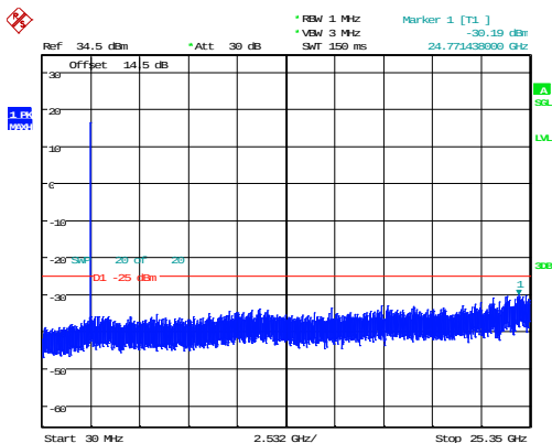
5MHz_Middle_QPSK_1@0 -30.19dBm
