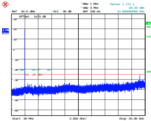
15MHz_Middle_QPSK_1@0 -28.93dBm
