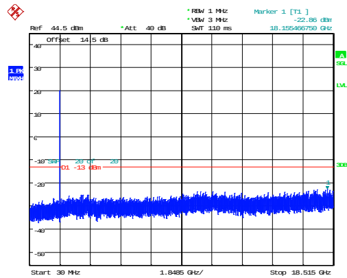
3MHz_Low_QPSK_1@0 -22.86dBm
