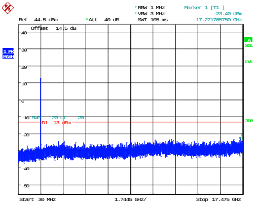
15MHz_High_QPSK_75@0 -23.40dBm
