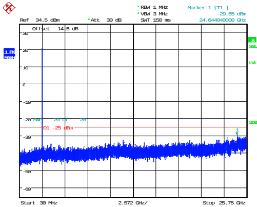
10MHz_Low_QPSK_1@0 -29.55dBm
