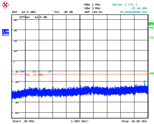
10MHz_High_QPSK_1@0 -22.40dBm
