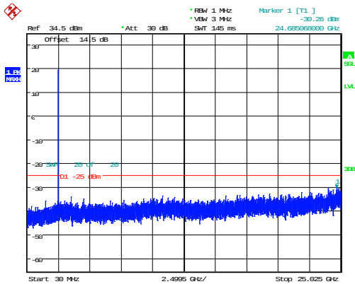
5MHz_Low_QPSK_1@0 -30.26dBm
