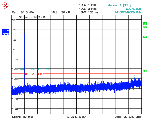
5MHz_High_QPSK_25@0 -29.71dBm
