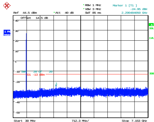
1.4MHz_High_QPSK_1@0 -24.95dBm
