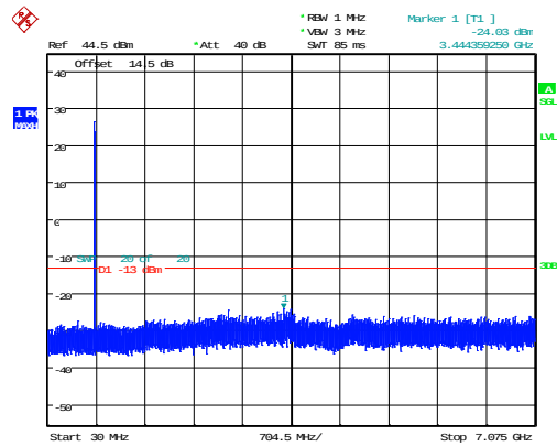
3MHz_Middle_QPSK_1@0 -24.03dBm
