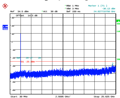
15MHz_High_QPSK_75@0 -30.13dBm
