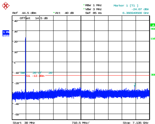
5MHz_High_QPSK_25@0 -24.07dBm
