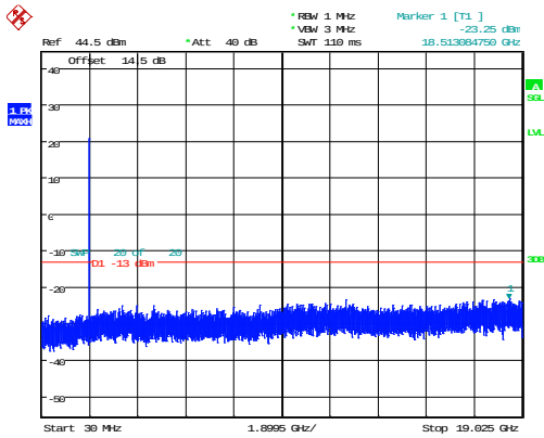
15MHz_High_QPSK_1@0 -23.25dBm
