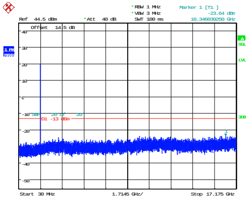
15MHz_Low_QPSK_1@0 -23.64dBm
