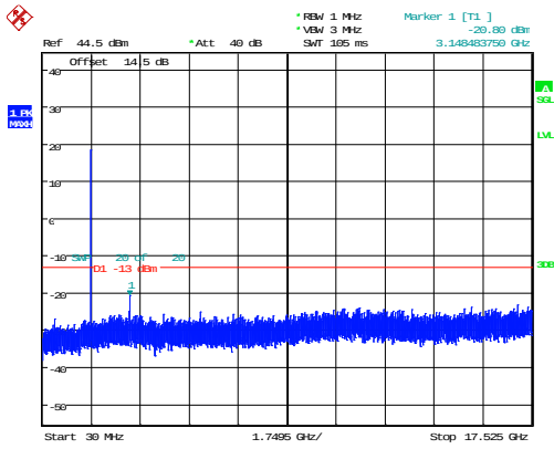
5MHz_High_QPSK_1@0 -20.80dBm
