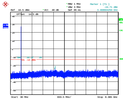
3MHz_Middle_QPSK_1@0 -24.71dBm
