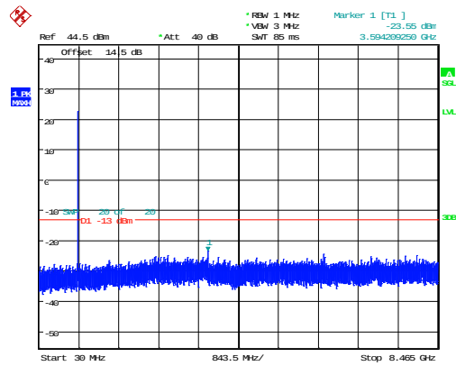
5MHz_High_QPSK_1@0 -23.55dBm
