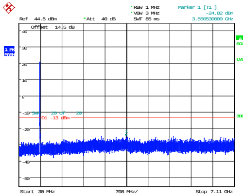
10MHz_High_QPSK_50@0 -24.82dBm
