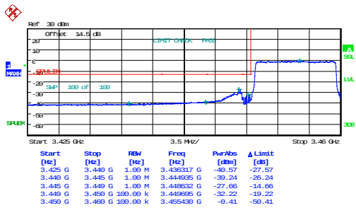
1_10MHz_Low_16QAM_50@0
