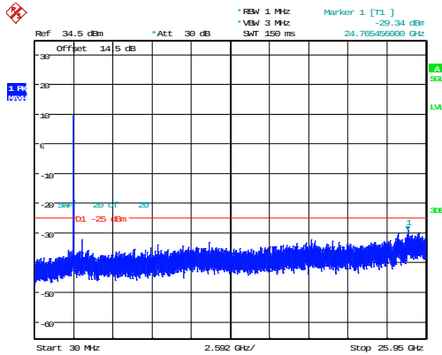
15MHz_Middle_QPSK_75@0 -29.34dBm
