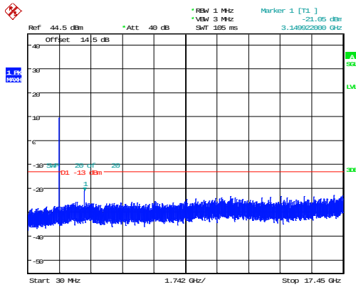
20MHz_High_QPSK_100@0 -21.05dBm
