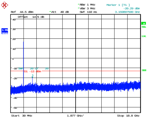
3MHz_Middle_QPSK_15@0 -20.29dBm
