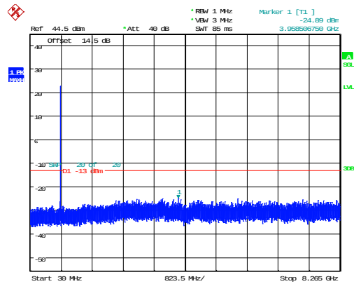
5MHz_Low_QPSK_1@0 -24.89dBm
