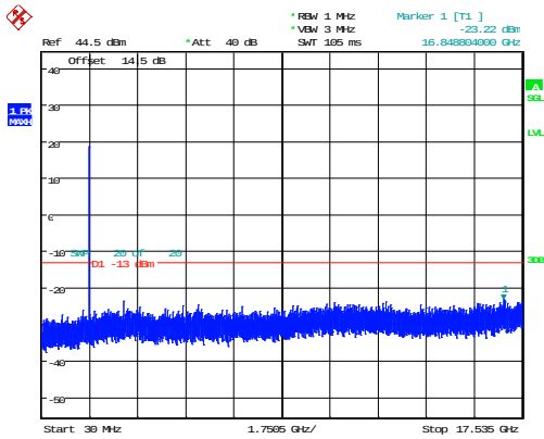
3MHz_High_QPSK_1@0 -23.22dBm
