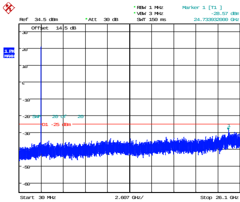
20MHz_High_QPSK_1@0 -28.57dBm
