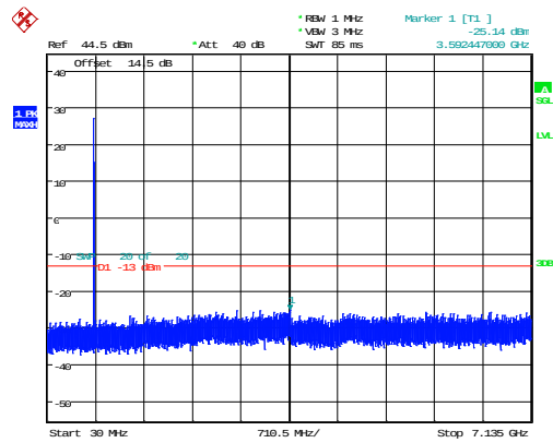
5MHz_High_QPSK_1@0 -25.14dBm
