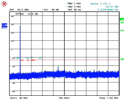
10MHz_Low_QPSK_1@0 -23.37dBm
