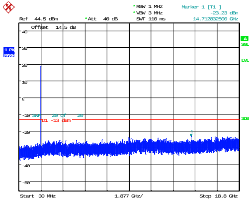
15MHz_Middle_QPSK_1@0 -23.23dBm
