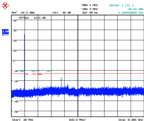
1.4MHz_Middle_QPSK_1@0 -20.62dBm
