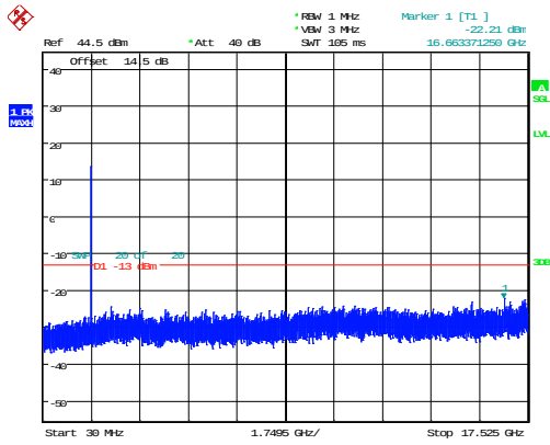
5MHz_High_QPSK_25@0 -22.21dBm
