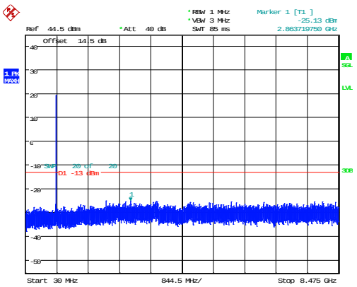
3MHz_High_QPSK_15@0 -25.13dBm
