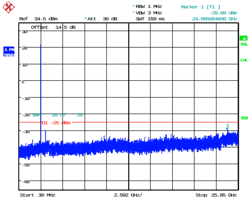
10MHz_Middle_QPSK_1@0 -29.69dBm
