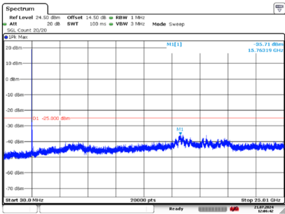
10MHz_Low_QPSK_1@0 -35.71dBm
