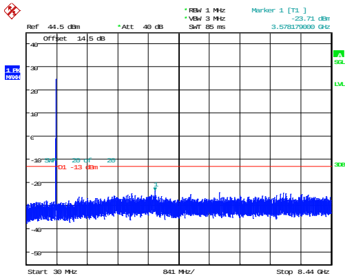
10MHz_High_QPSK_1@0 -23.71dBm
