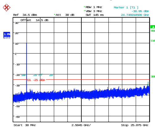
15MHz_Low_QPSK_75@0 -30.95dBm
