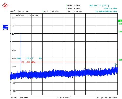
15MHz_Middle_QPSK_75@0 -30.23dBm
