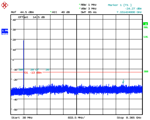
3MHz_Middle_QPSK_15@0 -24.27dBm
