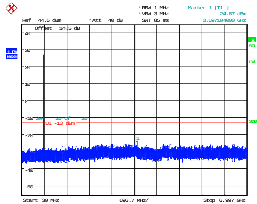
1.4MHz_Low_QPSK_1@0 -24.87dBm
