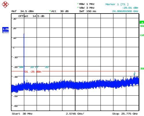
15MHz_Low_QPSK_75@0 -29.01dBm
