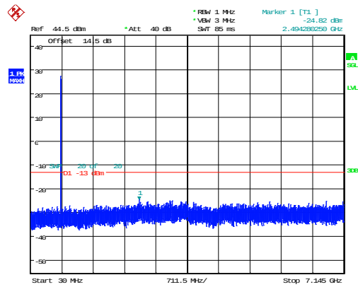
3MHz_High_QPSK_1@0 -24.82dBm
