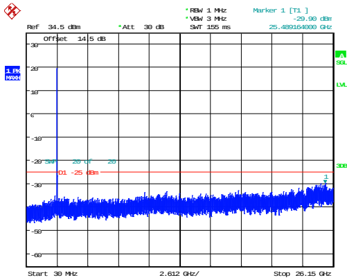
10MHz_High_QPSK_1@0 -29.90dBm
