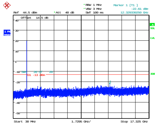
10MHz_Middle_QPSK_1@0 -22.61dBm
