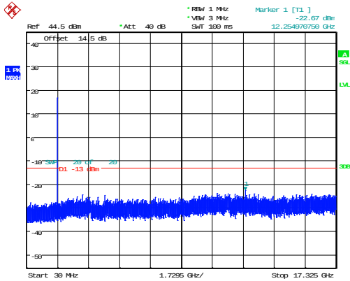
15MHz_Middle_QPSK_1@0 -22.67dBm
