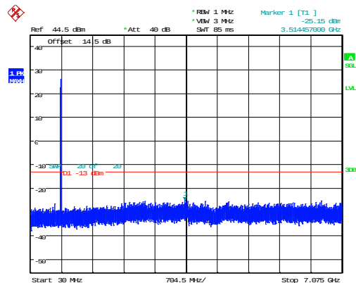
1.4MHz_Middle_QPSK_1@0 -25.15dBm
