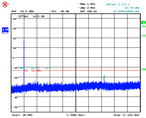
5MHz_Low_QPSK_1@0 -21.79dBm
