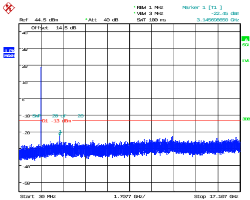
1.4MHz_Low_QPSK_1@0 -22.45dBm
