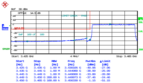
1_15MHz_Low_QPSK_75@0
