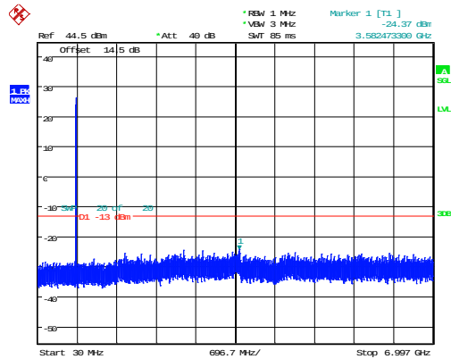
1.4MHz_Low_QPSK_6@0 -24.37dBm
