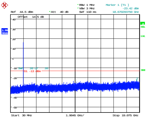
5MHz_High_QPSK_25@0 -23.42dBm
