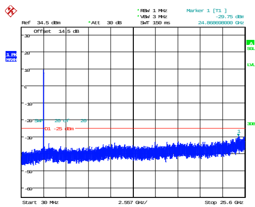
20MHz_High_QPSK_100@0 -29.75dBm
