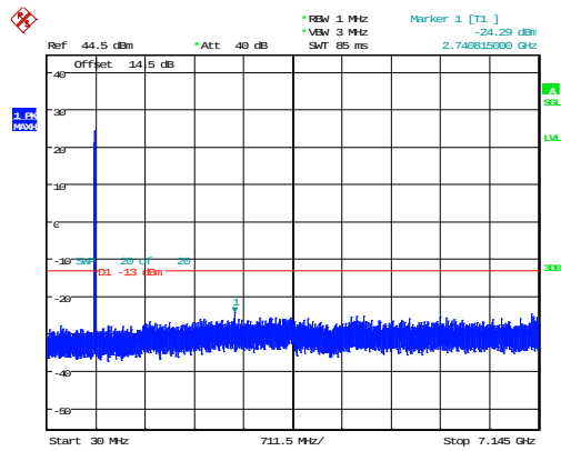
3MHz_High_QPSK_15@0 -24.29dBm
