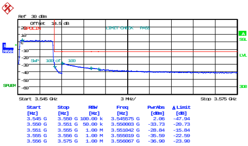
1_5MHz_High_QPSK_25@0
