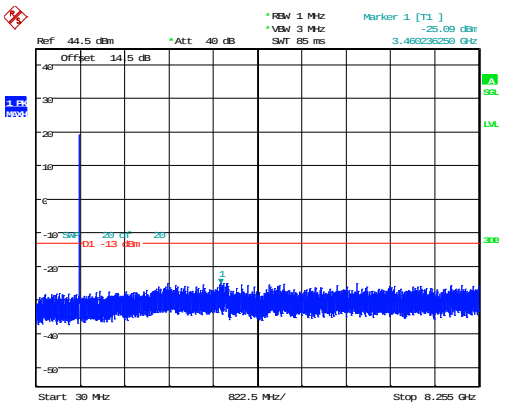
3MHz_Low_QPSK_15@0 -25.09dBm
