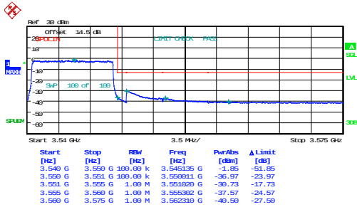
1_10MHz_High_16QAM_50@0
