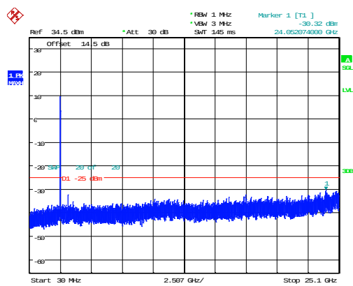
20MHz_Low_QPSK_100@0 -30.32dBm
