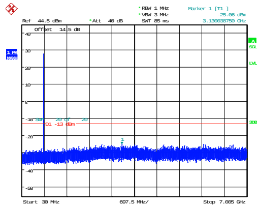
3MHz_Low_QPSK_1@0 -25.06dBm
