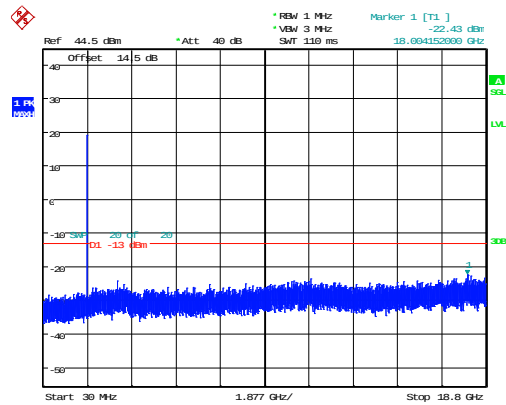
3MHz_Middle_QPSK_1@0 -22.43dBm
