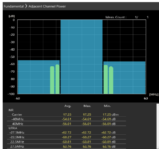
40MHz_30kHz_3680MHz-OFDM QPSK_RB50@25 -54.61,-56.01dB
