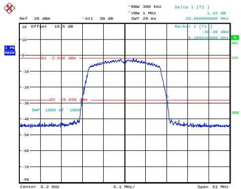
n20_5200MHz 20.808MHz
