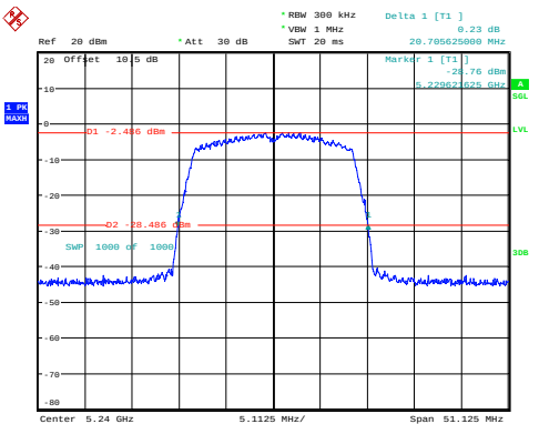
n20_5240MHz 20.706MHz
