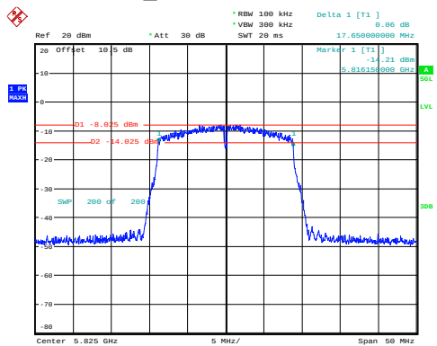
n20_5825MHz 17.650MHz
