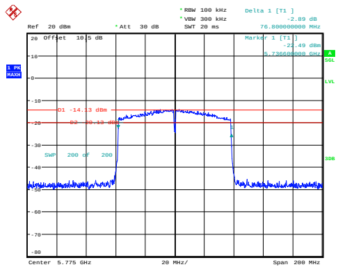
ac80_5775MHz 76.800MHz
