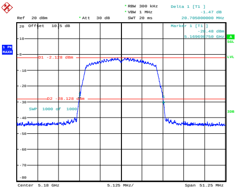
n20_5180MHz 20.705MHz
