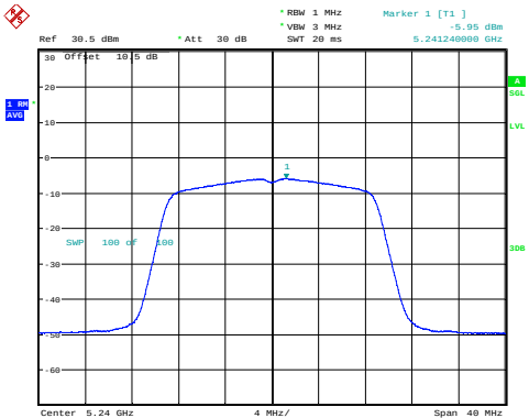
n20_5240MHz -5.95dBm/MHz
