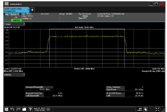
n78_2_60MHz_30kHz_3625MHz_CP-OFDM 16 QAM_RB162@0 57.691MHz
