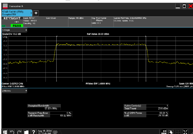
n78_2_60MHz_30kHz_3625MHz_CP-OFDM 64 QAM_RB162@0 57.874MHz
