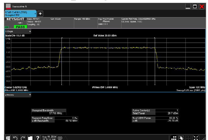
n78_2_60MHz_30kHz_3625MHz_CP-OFDM 256 QAM_RB162@0 57.708MHz
