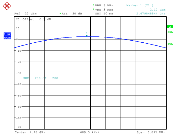
8DPSK_High 2.12dBm
