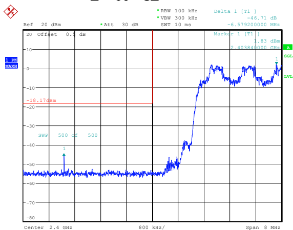
8DPSK_Hopping_Lower 46.71dB
