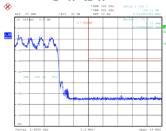
8DPSK_Hopping_Upper 54.11dB
