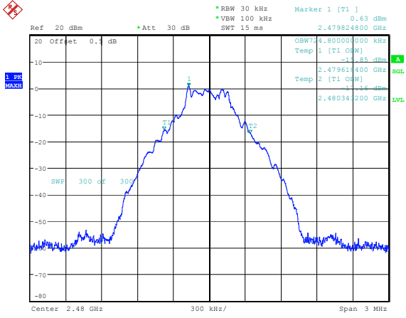
GFSK_High 0.725MHz
