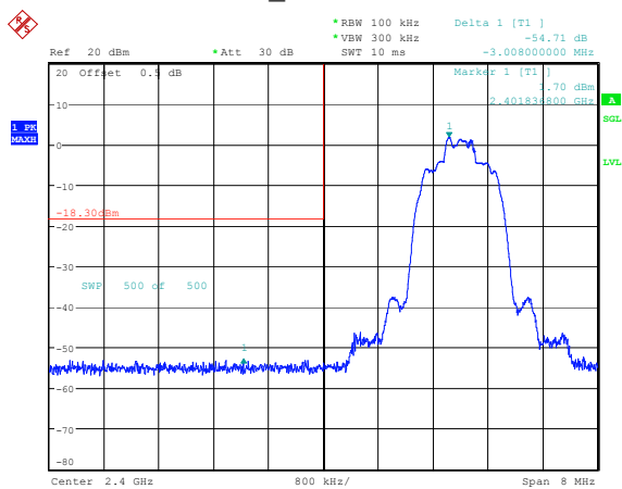
8DPSK_Low 54.71dB
