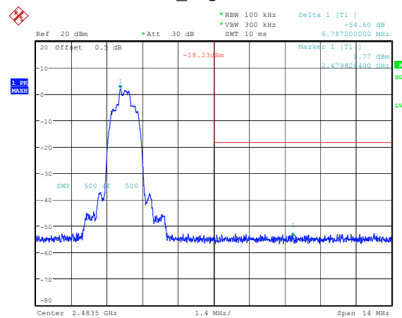
8DPSK_High 54.60dB
