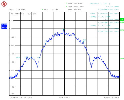
Middle 2.070MHz
