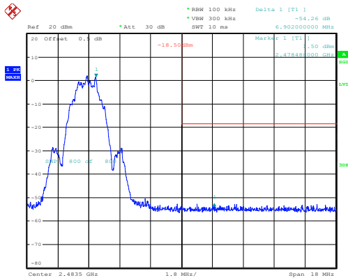
High 54.26dB
