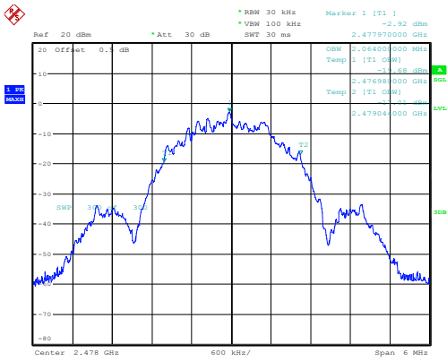
High 2.064MHz
