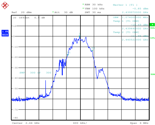
Middle 1.074MHz
