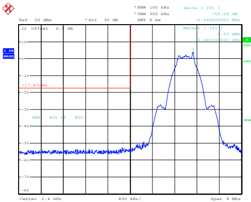
Low 55.28dB
