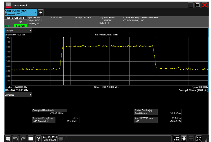
n77_3_50MHz_30kHz_3840MHz_CP-OFDM 16 QAM_RB133@0 47.403MHz
