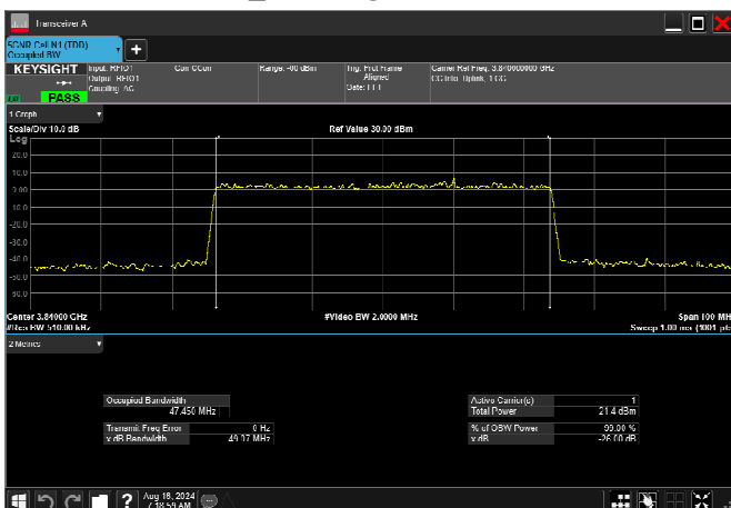
n77_3_50MHz_30kHz_3840MHz_CP-OFDM 64 QAM_RB133@0 47.450MHz
