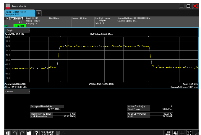
n77_3_50MHz_30kHz_3840MHz_CP-OFDM 256 QAM_RB133@0 47.293MHz
