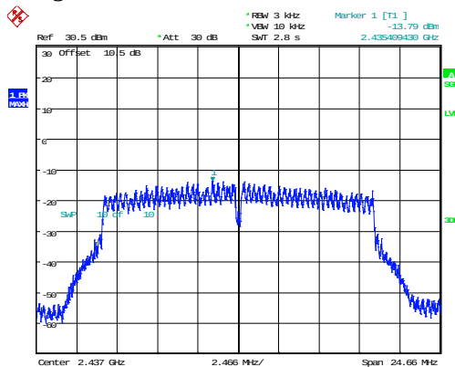
g_2437MHz_Chain 1 -13.79dBm/3kHz
