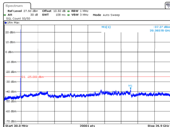
n41_30MHz_30kHz_2592.99MHz_DFT-s-OFDM QPSK_RB1@77 -37.37dBm
