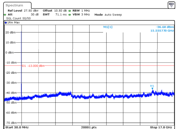
n66_10MHz_15kHz_1775MHz_DFT-s-OFDM QPSK_RB1@0 -36.68dBm
