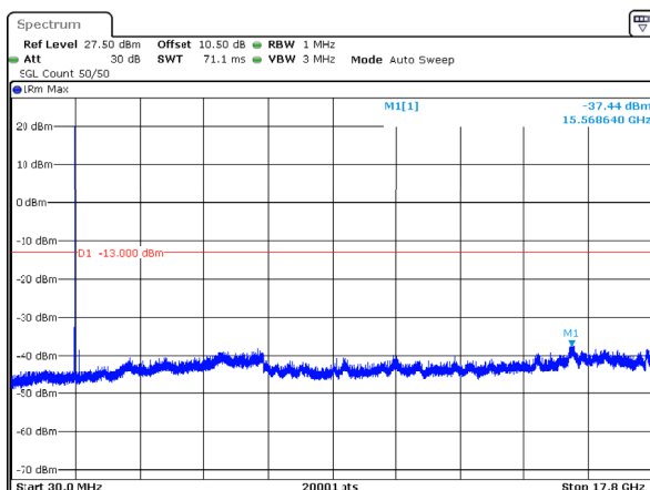
n66_10MHz_15kHz_1775MHz_DFT-s-OFDM QPSK_RB1@51 -37.44dBm
