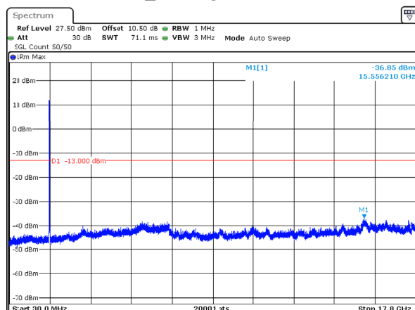
n66_15MHz_15kHz_1772.5MHz_DFT-s-OFDM QPSK_RB75@0 -36.85dBm
