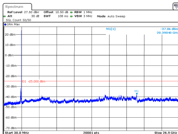
n41_100MHz_30kHz_2592.99MHz_DFT-s-OFDM QPSK_RB1@272 -37.86dBm
