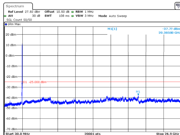
n41_50MHz_30kHz_2664.99MHz_DFT-s-OFDM QPSK_RB128@0 -37.72dBm
