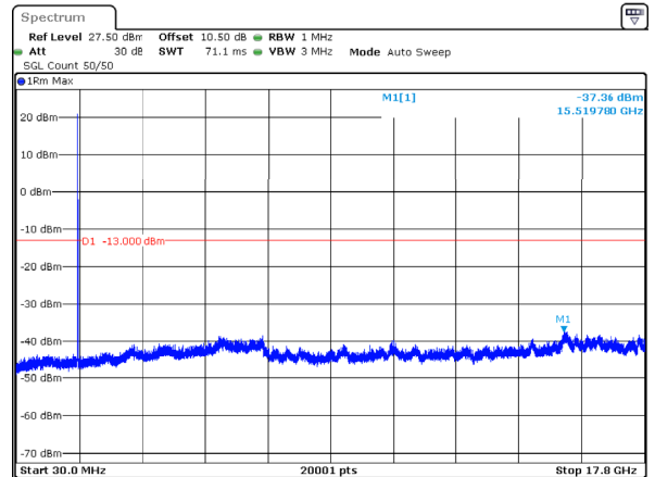
n66_10MHz_15kHz_1745MHz_DFT-s-OFDM QPSK_RB1@51 -37.36dBm
