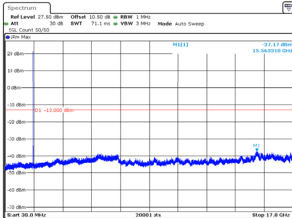
n66_10MHz_15kHz_1745MHz_DFT-s-OFDM QPSK_RB1@0 -37.17dBm
