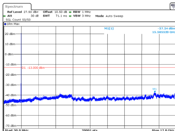
n66_15MHz_15kHz_1772.5MHz_DFT-s-OFDM QPSK_RB1@78 -37.54dBm
