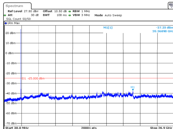
n41_20MHz_30kHz_2592.99MHz_DFT-s-OFDM QPSK_RB1@0 -37.33dBm
