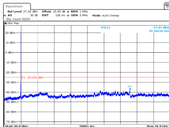
n41_50MHz_30kHz_2664.99MHz_DFT-s-OFDM QPSK_RB1@132 -37.62dBm
