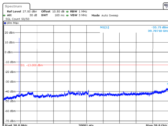
n77_3_70MHz_30kHz_3735MHz_DFT-s-OFDM QPSK_RB1@0 -35.73dBm
