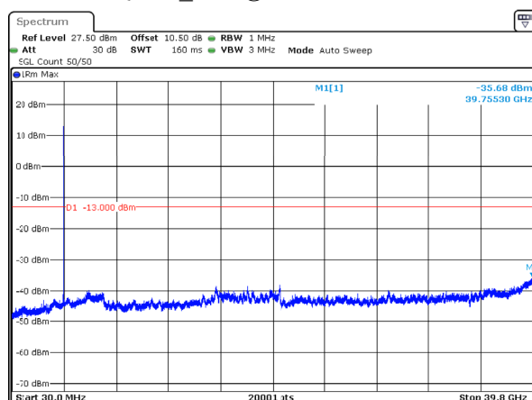
n77_3_80MHz_30kHz_3940MHz_DFT-s-OFDM QPSK_RB1@216 -35.68dBm
