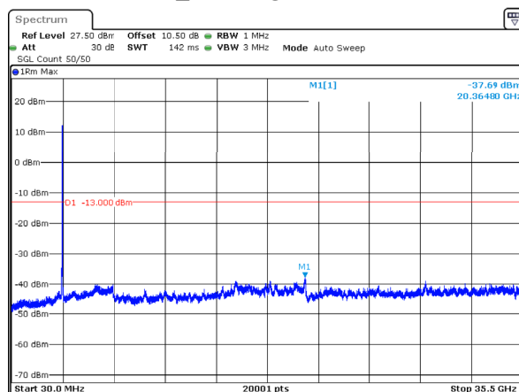
n78_1_40MHz_30kHz_3500MHz_DFT-s-OFDM QPSK_RB100@0 -37.69dBm
