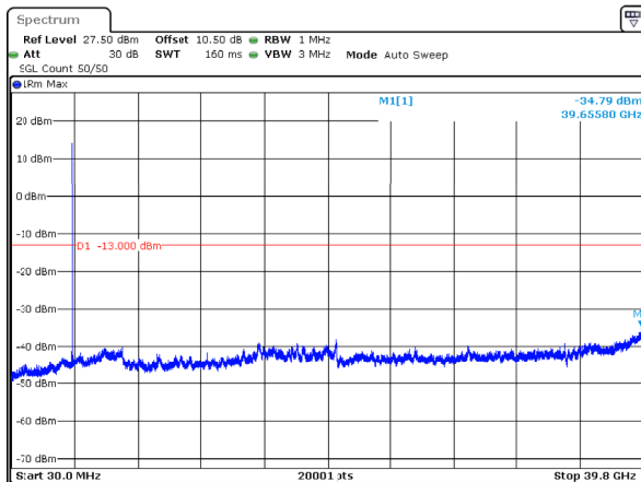
n77_3_60MHz_30kHz_3840MHz_DFT-s-OFDM QPSK_RB1@161 -34.79dBm
