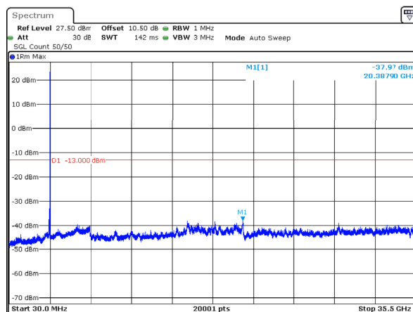
n78_1_40MHz_30kHz_3500MHz_DFT-s-OFDM QPSK_RB1@105 -37.97dBm
