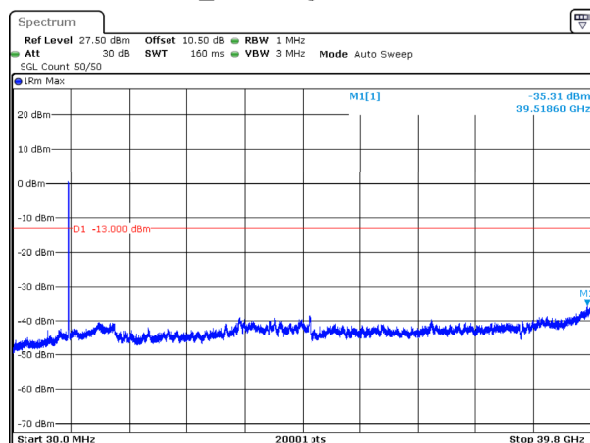
n77_3_80MHz_30kHz_3840MHz_DFT-s-OFDM QPSK_RB216@0 -35.31dBm
