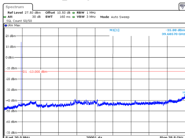
n77_3_70MHz_30kHz_3735MHz_DFT-s-OFDM QPSK_RB1@188 -35.88dBm
