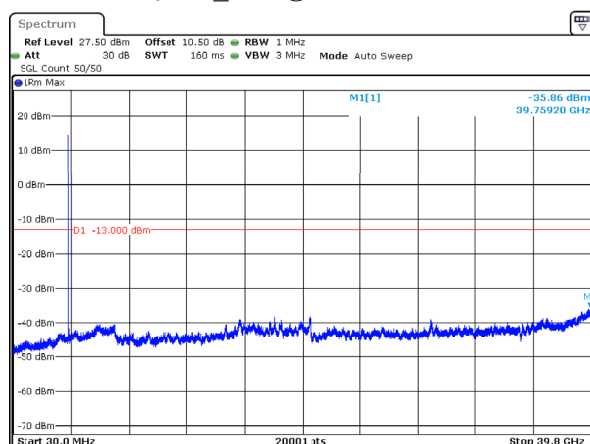
n77_3_70MHz_30kHz_3840MHz_DFT-s-OFDM QPSK_RB1@0 -35.86dBm
