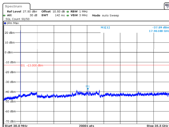
n78_1_20MHz_30kHz_3540MHz_DFT-s-OFDM QPSK_RB1@50 -37.89dBm
