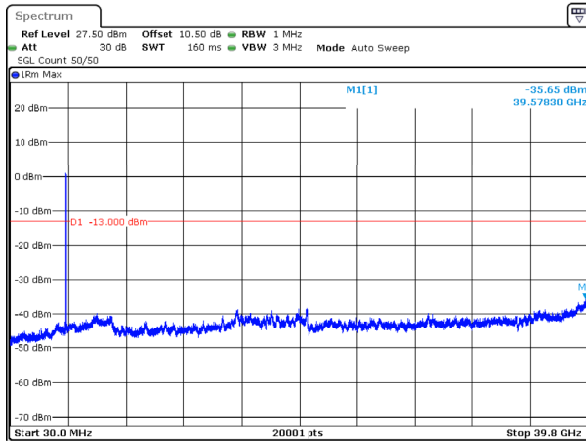
n77_3_60MHz_30kHz_3840MHz_DFT-s-OFDM QPSK_RB162@0 -35.65dBm
