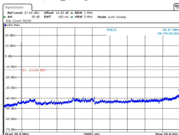
n77_3_70MHz_30kHz_3840MHz_DFT-s-OFDM QPSK_RB1@188 -35.67dBm
