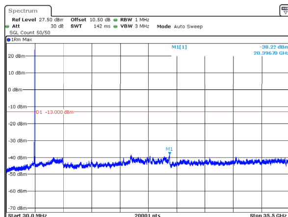
n78_1_50MHz_30kHz_3475MHz_DFT-s-OFDM QPSK_RB1@132 -38.22dBm
