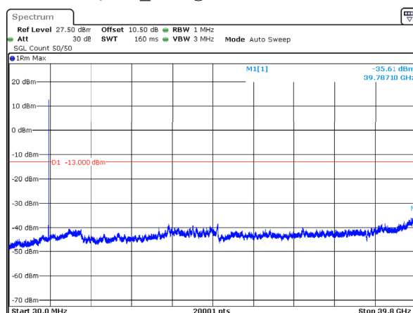
n77_3_50MHz_30kHz_3840MHz_DFT-s-OFDM QPSK_RB1@132 -35.61dBm
