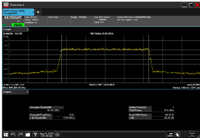
n77_2_20MHz_30kHz_3625MHz_CP-OFDM 256 QAM_RB51@0 18.183MHz
