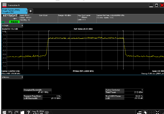
n77_2_50MHz_30kHz_3625MHz_CP-OFDM 64 QAM_RB133@0 47.461MHz
