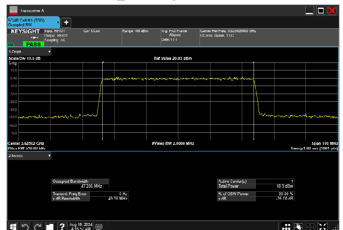
n77_2_50MHz_30kHz_3625MHz_CP-OFDM 256 QAM_RB133@0 47.286MHz
