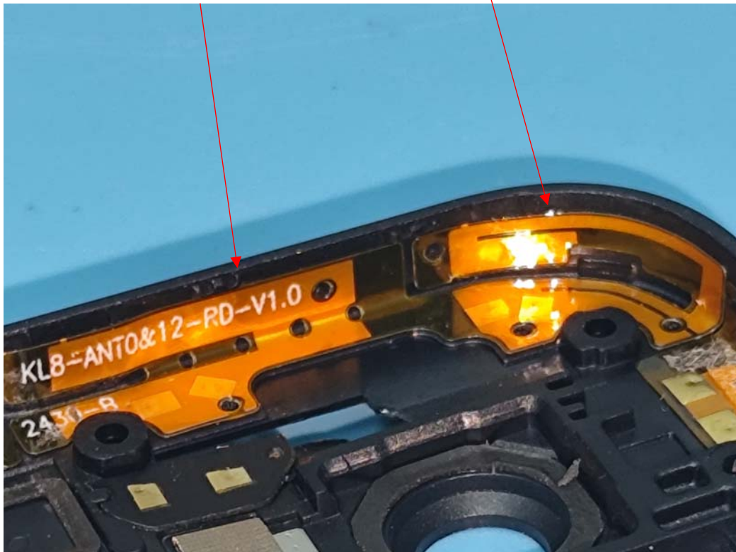
ANT12 (BT/WIFI_2.4G(chain 0)+5G) ANT0 (GPS+B42/N77/78 PRX)
