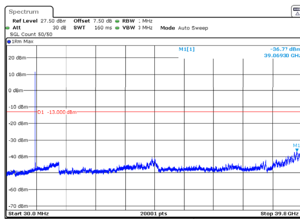
n77_3_30MHz_30kHz_3840MHz_DFT-s-OFDM QPSK_RB1@0 -36.77dBm
