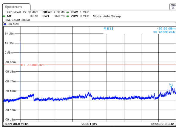
n77_3_40MHz_30kHz_3840MHz_DFT-s-OFDM QPSK_RB1@105 -36.96dBm
