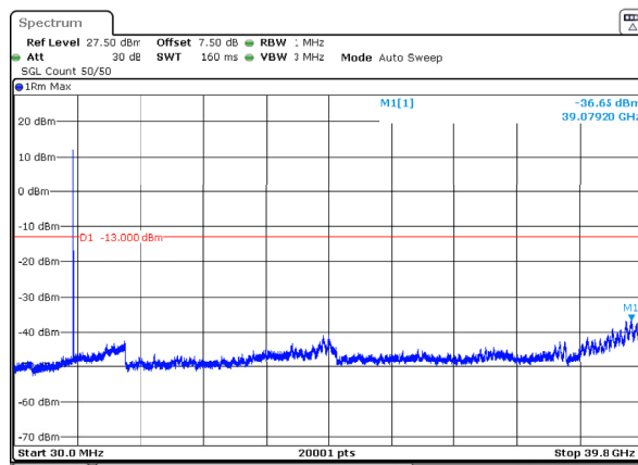
n77_3_30MHz_30kHz_3715MHz_DFT-s-OFDM QPSK_RB1@77 -36.65dBm
