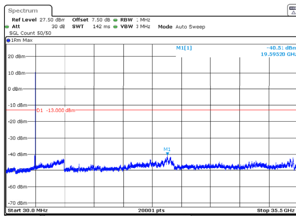
n77_1_80MHz_30kHz_3490MHz_DFT-s-OFDM QPSK_RB1@216 -40.51dBm
