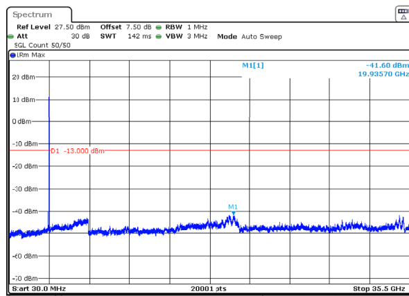
n77_1_80MHz_30kHz_3500MHz_DFT-s-OFDM QPSK_RB1@216 -41.60dBm
