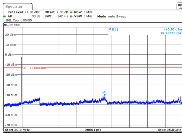
n77_1_80MHz_30kHz_3500MHz_DFT-s-OFDM QPSK_RB216@0 -40.95dBm
