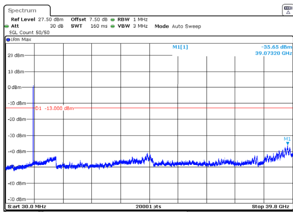
n77_3_40MHz_30kHz_3840MHz_DFT-s-OFDM QPSK_RB100@0 -35.65dBm
