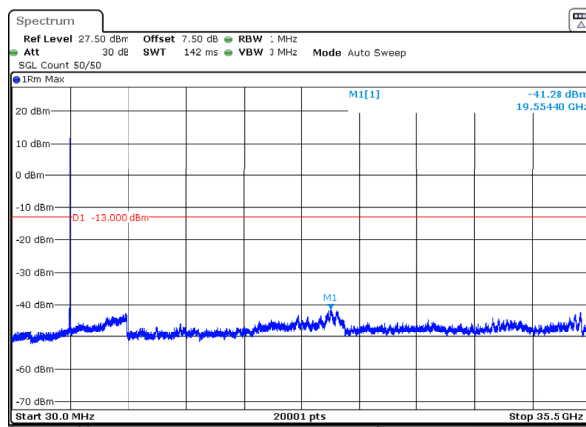
n77_1_70MHz_30kHz_3515MHz_DFT-s-OFDM QPSK_RB1@188 -41.28dBm
