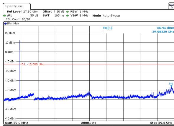
n77_3_30MHz_30kHz_3715MHz_DFT-s-OFDM QPSK_RB1@0 -36.95dBm
