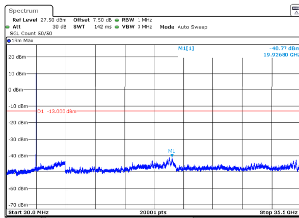
n77_1_80MHz_30kHz_3510MHz_DFT-s-OFDM QPSK_RB1@216 -40.77dBm
