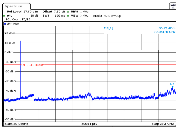
n77_3_20MHz_30kHz_3840MHz_DFT-s-OFDM QPSK_RB1@50 -36.77dBm
