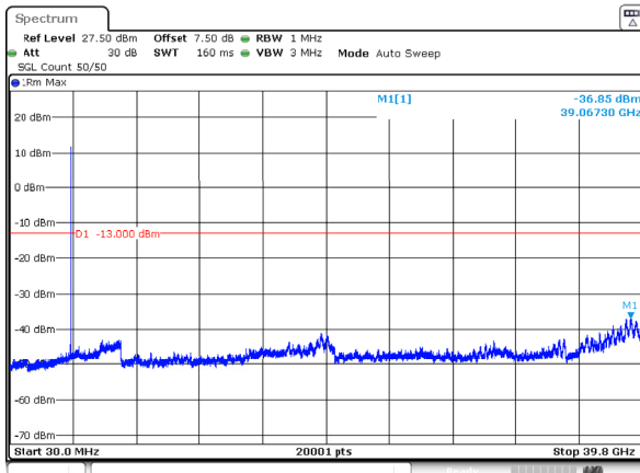
n77_3_30MHz_30kHz_3840MHz_DFT-s-OFDM QPSK_RB1@77 -36.85dBm
