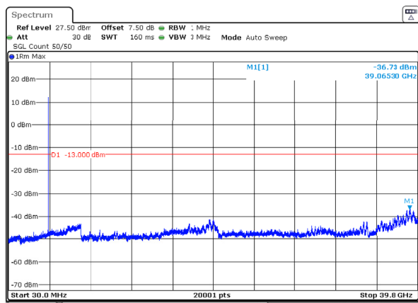
n77_3_10MHz_30kHz_3840MHz_DFT-s-OFDM QPSK_RB1@23 -36.73dBm
