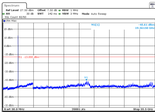
n77_1_90MHz_30kHz_3495MHz_DFT-s-OFDM QPSK_RB1@244 -40.61dBm
