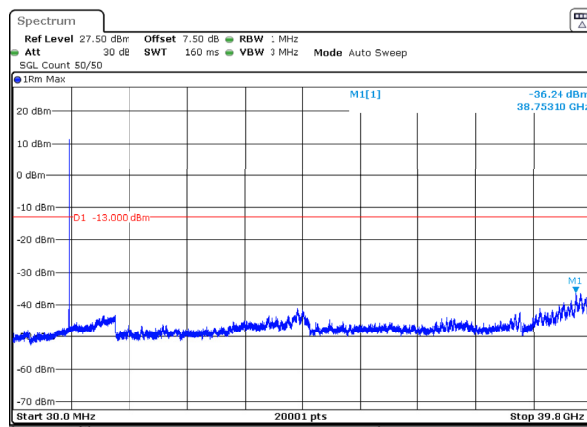
n77_3_50MHz_30kHz_3840MHz_DFT-s-OFDM QPSK_RB1@132 -36.24dBm
