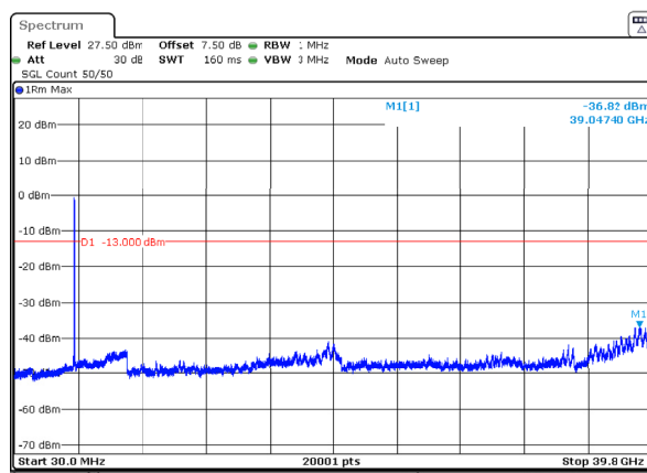
n77_3_60MHz_30kHz_3730MHz_DFT-s-OFDM QPSK_RB162@0 -36.82dBm
