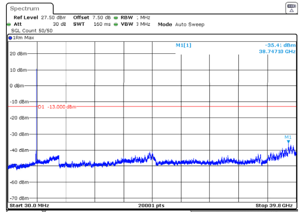
n77_3_100MHz_30kHz_3840MHz_DFT-s-OFDM QPSK_RB1@272 -35.41dBm
