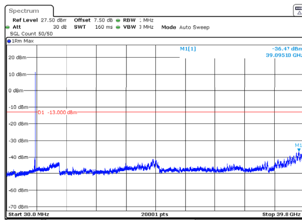
n77_3_90MHz_30kHz_3745MHz_DFT-s-OFDM QPSK_RB1@244 -36.47dBm
