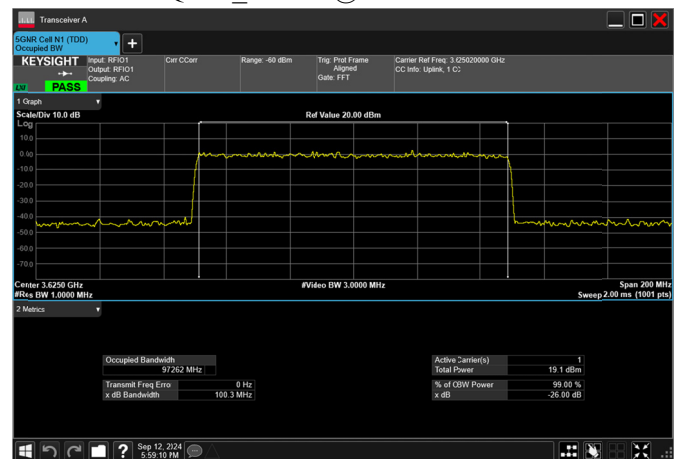
n77_2_100MHz_30kHz_3625MHz_CP-OFDM 256 QAM_RB273@0 97.262MHz
