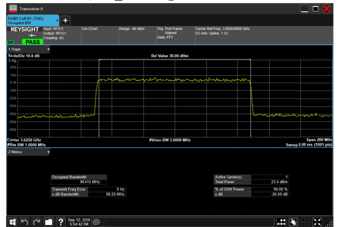
n77_2_100MHz_30kHz_3625MHz_DFT-s-OFDM 16 QAM_RB270@0 96.415MHz
