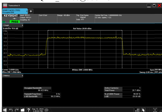
n77_2_100MHz_30kHz_3600MHz_DFT-s-OFDM 256 QAM_RB270@0 96.423MHz
