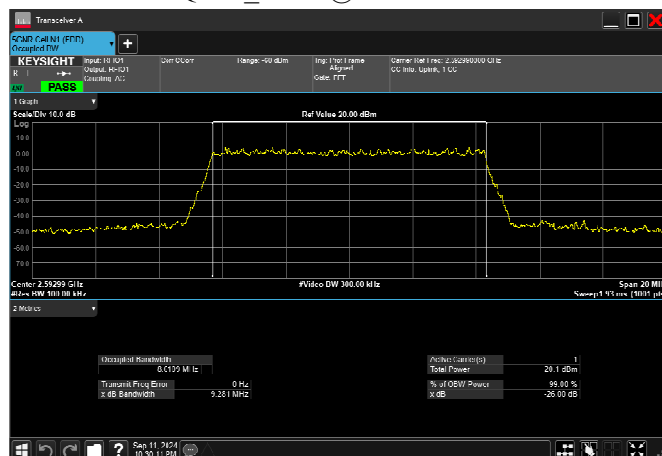
n41_10MHz_30kHz_2592.99MHz_CP-OFDM 256 OAM RB24@0 8.611MHz
