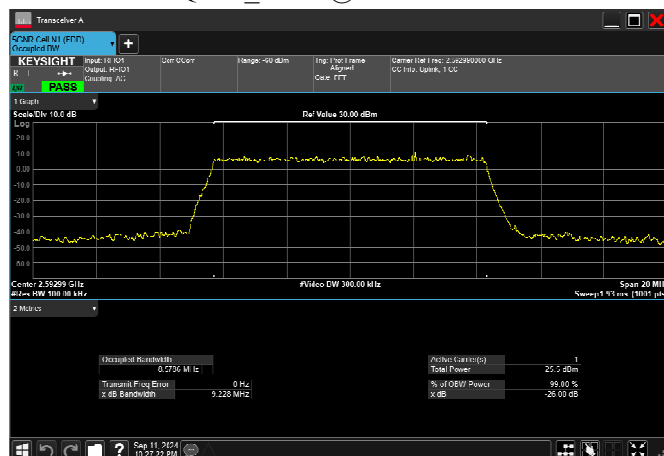
n41_10MHz_30kHz_2592.99MHz_DFT-s-OFDM 16 QAM RB24@0 8.579MHz
