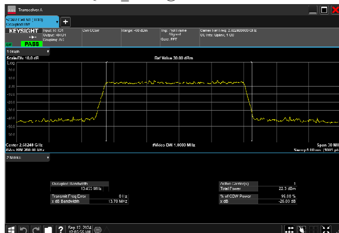
n41_15MHz_30kHz_2682.48MHz_CP-OFDM 16 QAM RB38@0 13.562MHz
