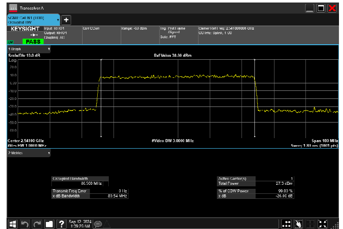
n41_90MHz_30kHz_2541MHz_DFT-s-OFDM 64 QAM_RB243@0 86.571MHz
