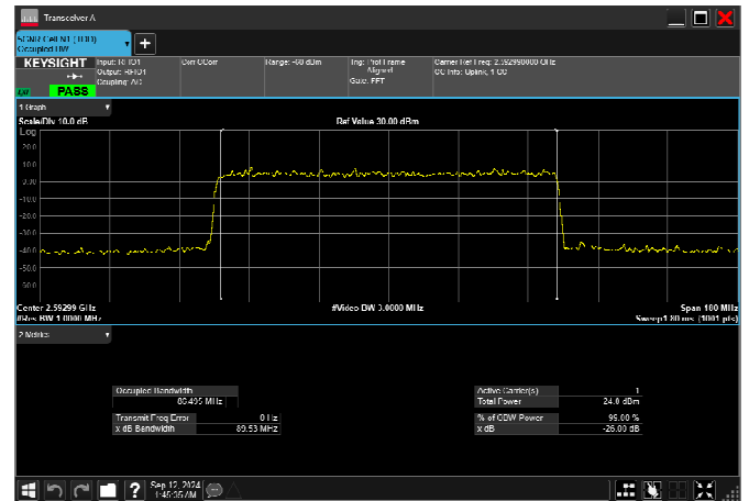
n41_90MHz_30kHz_2592.99MHz_CP-OFDM 16 QAM_RB245@0 87.260MHz
