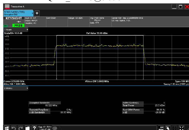
n41_90MHz_30kHz_2592.99MHz_DFT-s-OFDM 16 QAM RB243@0 86.522MHz
