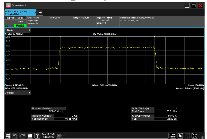
n41_90MHz_30kHz_2592.99MHz_CP-OFDM 256 QAM_RB245@0 87.297MHz
