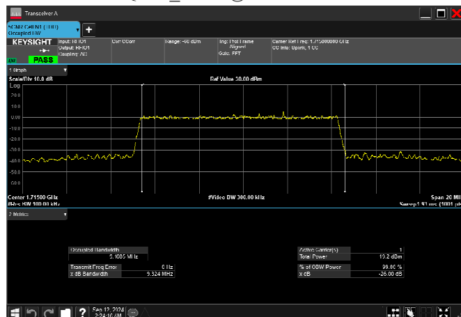
n66_10MHz_15kHz_1715MHz_CP-OFDM 16 QAM RB52@0 9.296MHz
