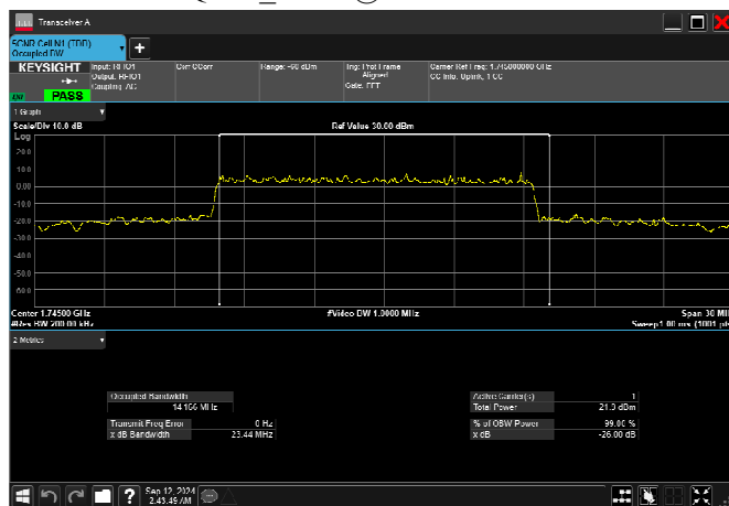
n66_15MHz_15kHz_1745MHz_DFT-s-OFDM 16 QAM RB75@0 14.166MHz
