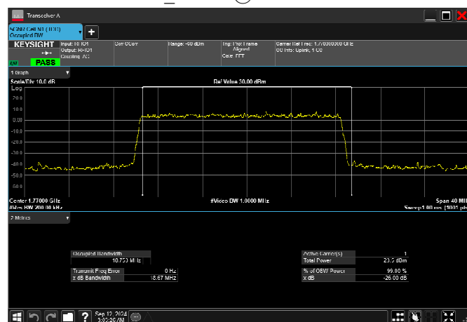
n66_20MHz_15kHz_1770MHz_DFT-s-OFDM 16 OAM RB100@0 18.802MHz
