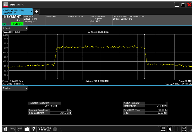
n66_30MHz_15kHz_1745MHz_CP-OFDM 256 QAM_RB160@0 28.464MHz
