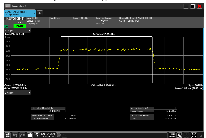
n66_30MHz_15kHz_1765MHz_DFT-s-OFDM 16 QAM_RB160@0 28.468MHz
