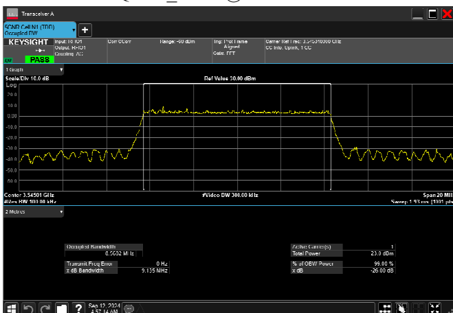
n77_1_10MHz_30kHz_3545MHz_DFT-s-OFDM QPSK_RB24@0 8.568MHz
