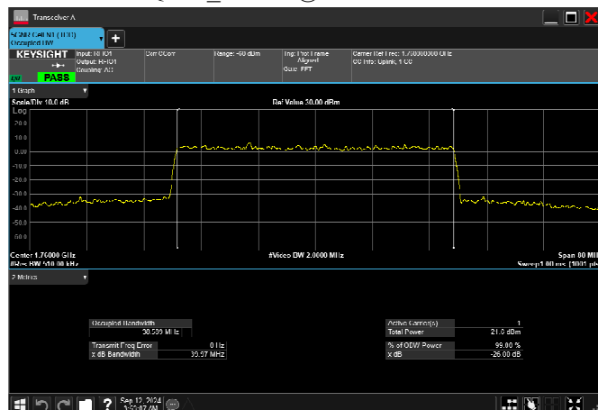
n66_40MHz_15kHz_1760MHz_CP-OFDM 64 QAM RB216@0 38.589MHz
