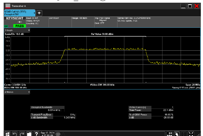
n77_1_10MHz_30kHz_3545MHz_DFT-s-OFDM 16 QAM_RB24@0 8.601MHz
