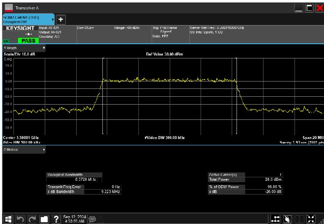
n77_1_10MHz_30kHz_3500MHz_CP-OFDM 256 QAM_RB24@0 8.615MHz
