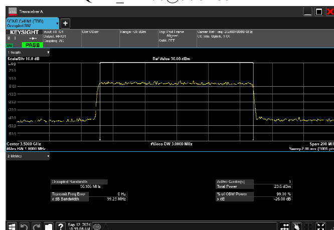
n77_1_100MHz_30kHz_3500MHz_DFT-s-OFDM 16 OAM RB270@0 96.186MHz
