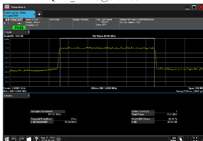
n77_1_90MHz_30kHz_3500MHz_CP-OFDM 256 QAM RB245@0 87.193MHz
