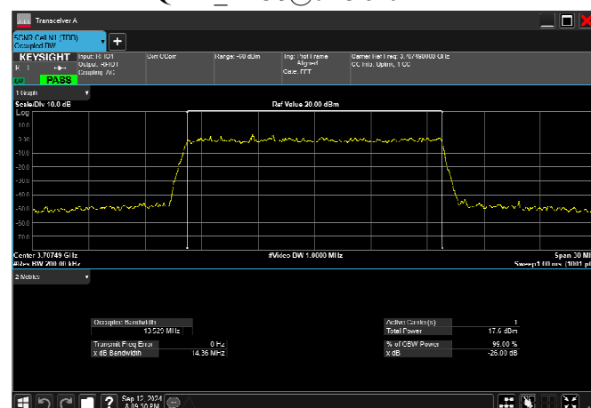
n77_3_15MHz_30kHz_3707.5MHz_CP-OFDM 256 QAM RB38@0 13.529MHz
