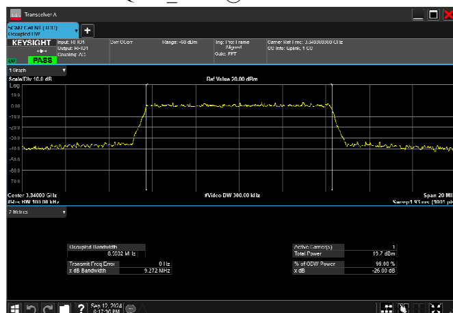
n77_3_10MHz_30kHz_3840MHz_CP-OFDM 16 OAM RB24@0.8577MHz
