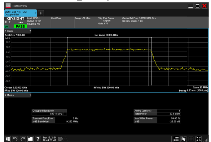
n77_2_10MHz_30kHz_3625MHz_DFT-s-OFDM 16 QAM_RB24@0 8.601MHz
