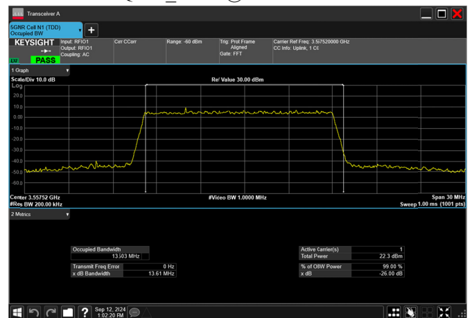
n77_2_15MHz_30kHz_3557.5MHz_DFT-s-OFDM 16 QAM_RB36@0 13.503MHz
