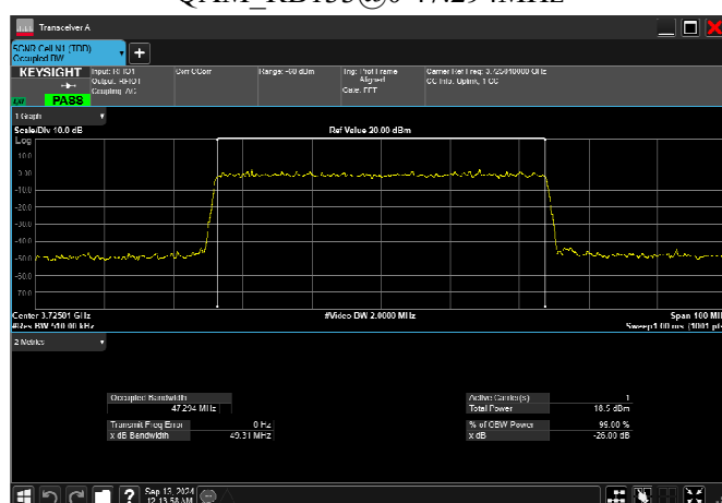
n77_3_50MHz_30kHz_3725MHz_CP-OFDM 256 OAM RB133@0 47.294MHz
