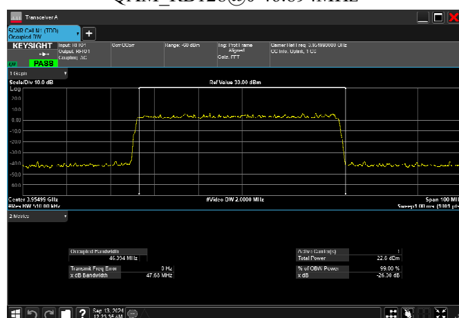
n77_3_50MHz_30kHz_3955MHz_DFT-s-OFDM 16 OAM RB128@0 46.894MHz
