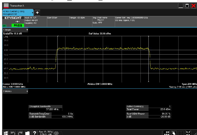
n77_3_100MHz_30kHz_3930MHz_CP-OFDM 16 QAM_RB273@0 97.226MHz
