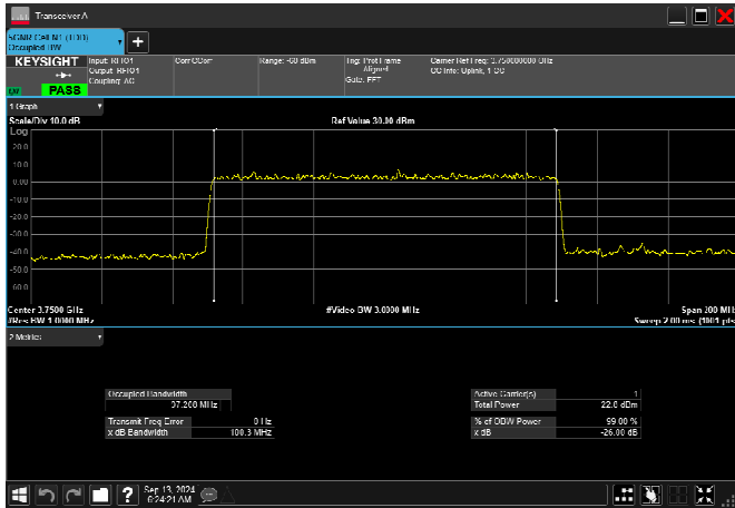
n77_3_100MHz_30kHz_3750MHz_CP-OFDM 256 QAM_RB273@0 97.297MHz
